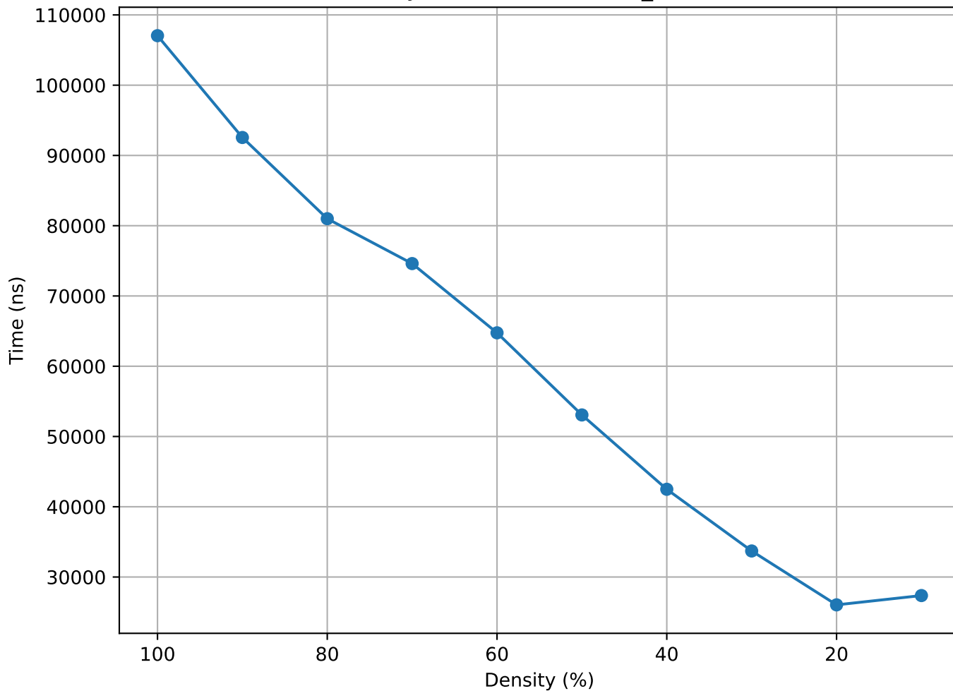
Matrix Density vs Time (lowThrust_12 - truncated)
