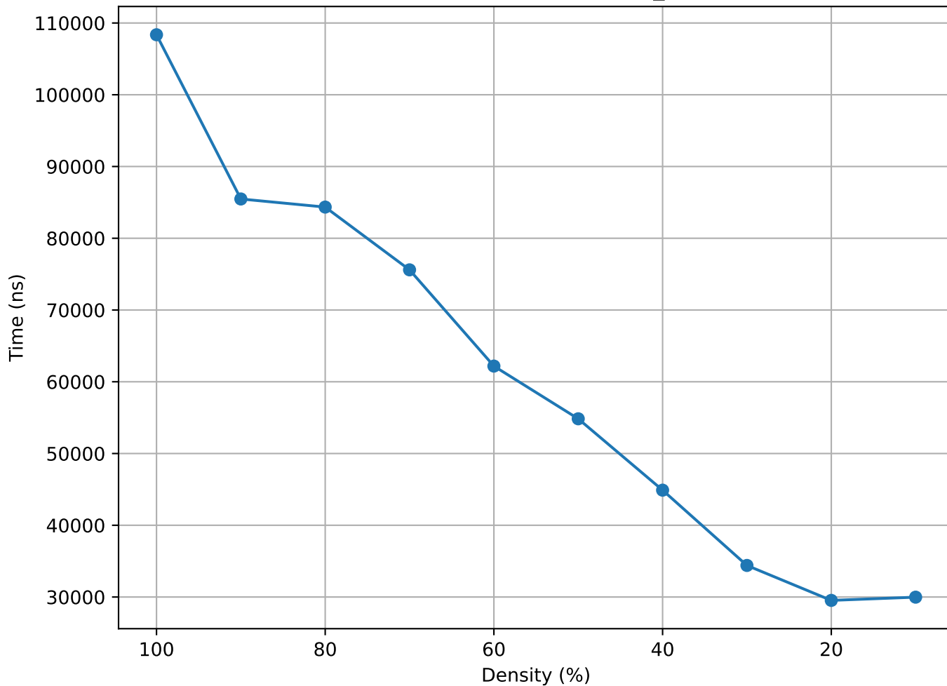
Matrix Density vs Time (lowThrust_13 - consec)
