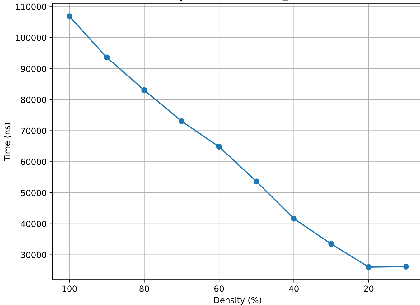
Matrix Density vs Time (lowThrust_13 - truncated)
