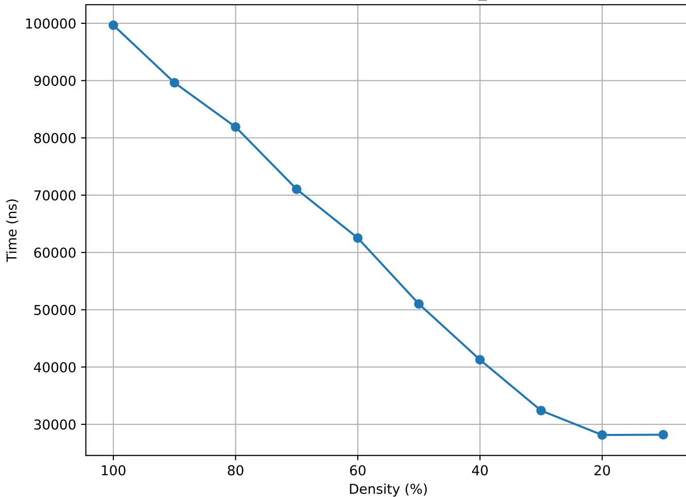
Matrix Density vs Time (lowThrust_7 - consec)
