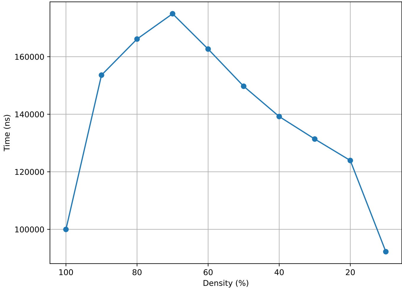
Matrix Density vs Time (lowThrust_7 - random)
