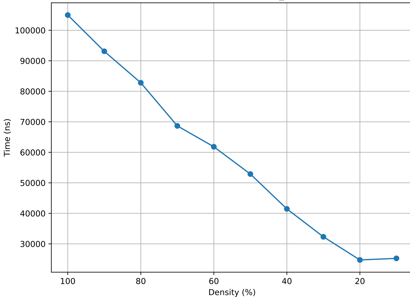
Matrix Density vs Time (lowThrust_9 - truncated)
