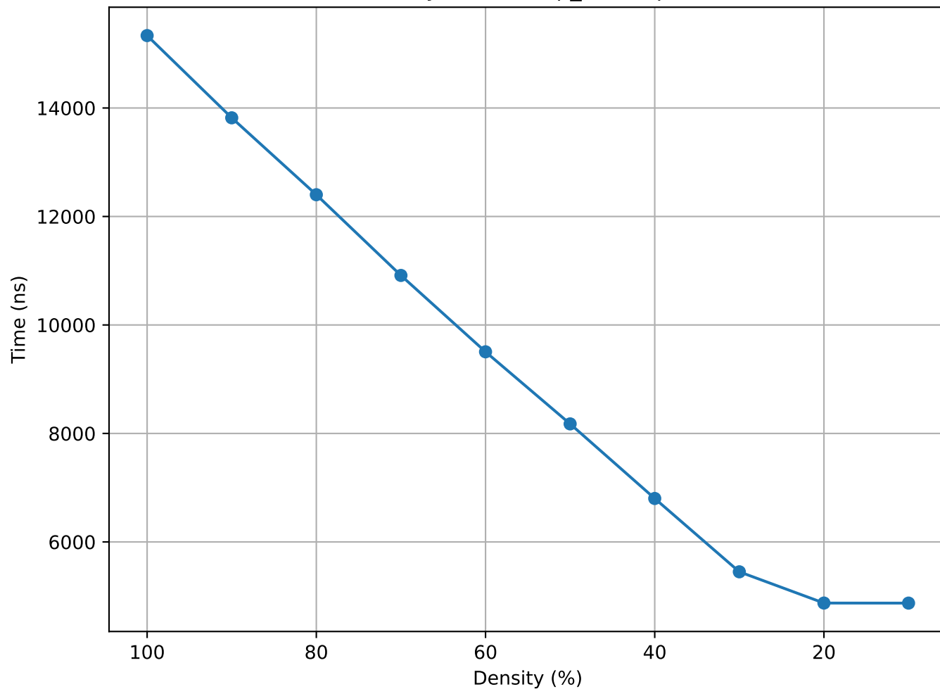
Matrix Density vs Time (lp_wood1p - consec)
