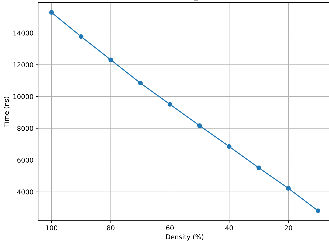
Matrix Density vs Time (lp_wood1p - truncated)
