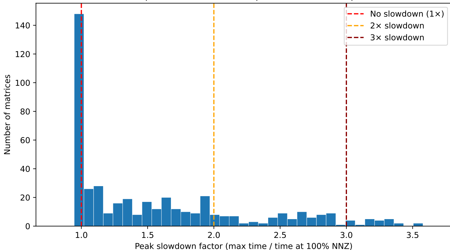
Distribution of timing slowdown under random NNZ removal n=461 matrices | >1.05x: 303 (66%) | >2x: 103 (22%) | >3x: 23 (5%)
