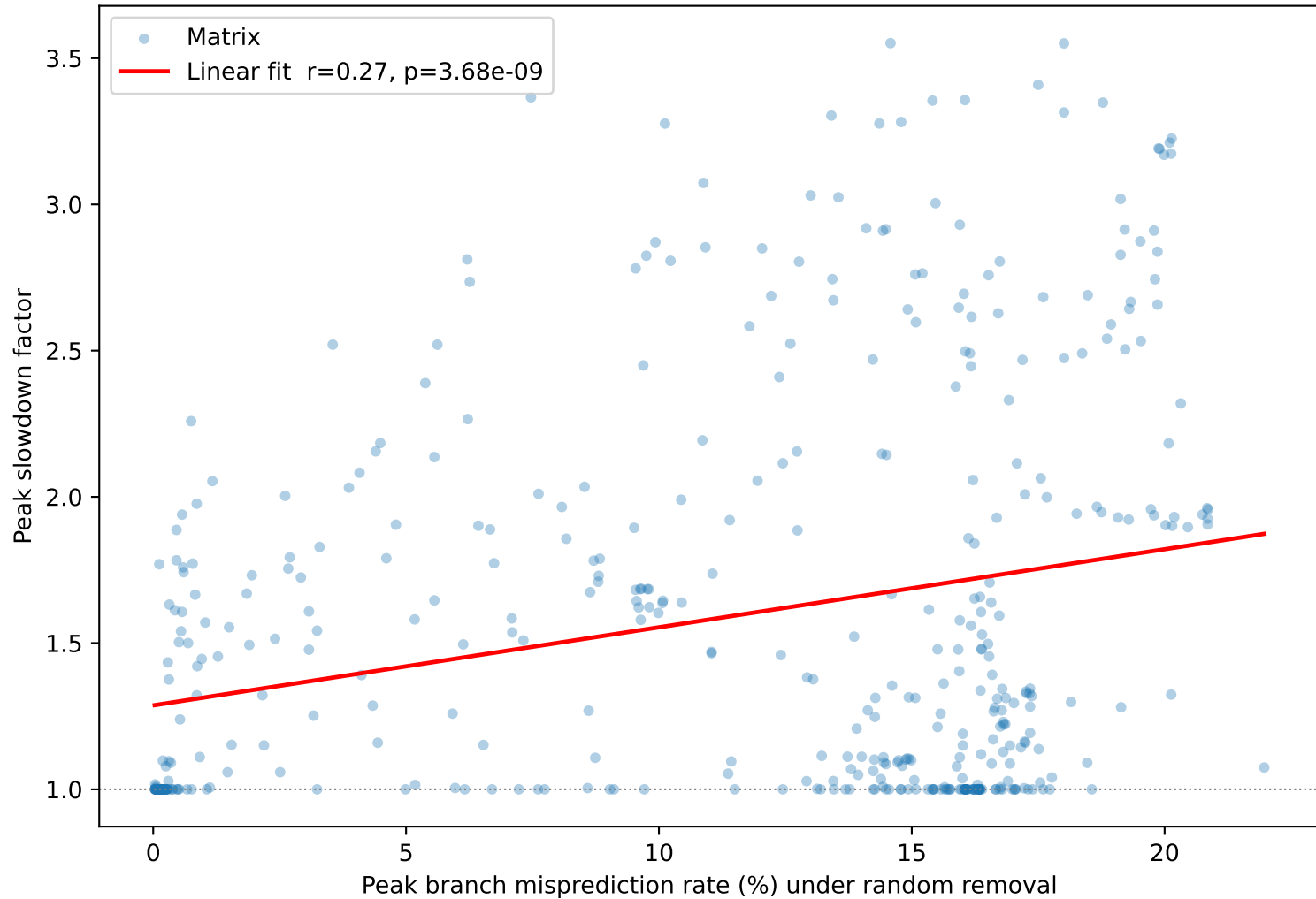
Peak slowdown vs peak branch misprediction rate n=461 SpMV matrices (sweep_matrices_warmup)
