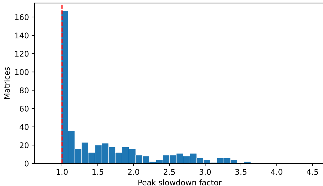
Naive CSR SpMV (n=460) 302 (66%) anomalous
