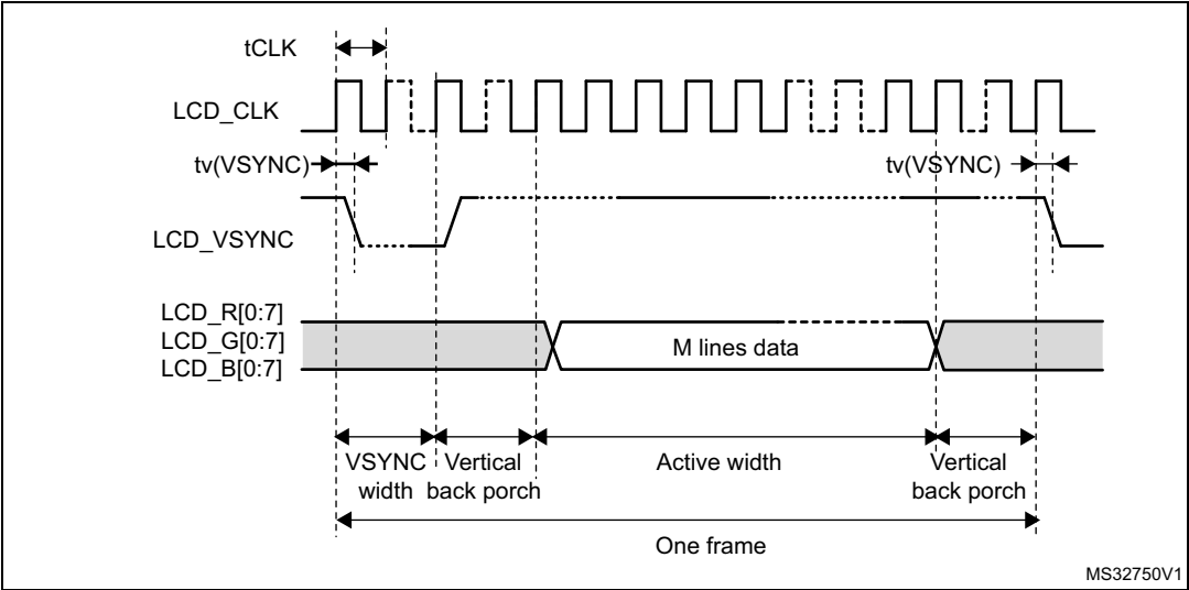
Figure 46. LCD-TFT vertical timing diagram
