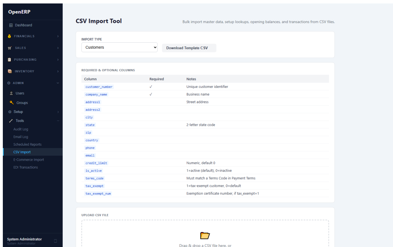
Figure 1.8: CSV Import Tool showing the Customers import type with required/optional columns and file upload area
