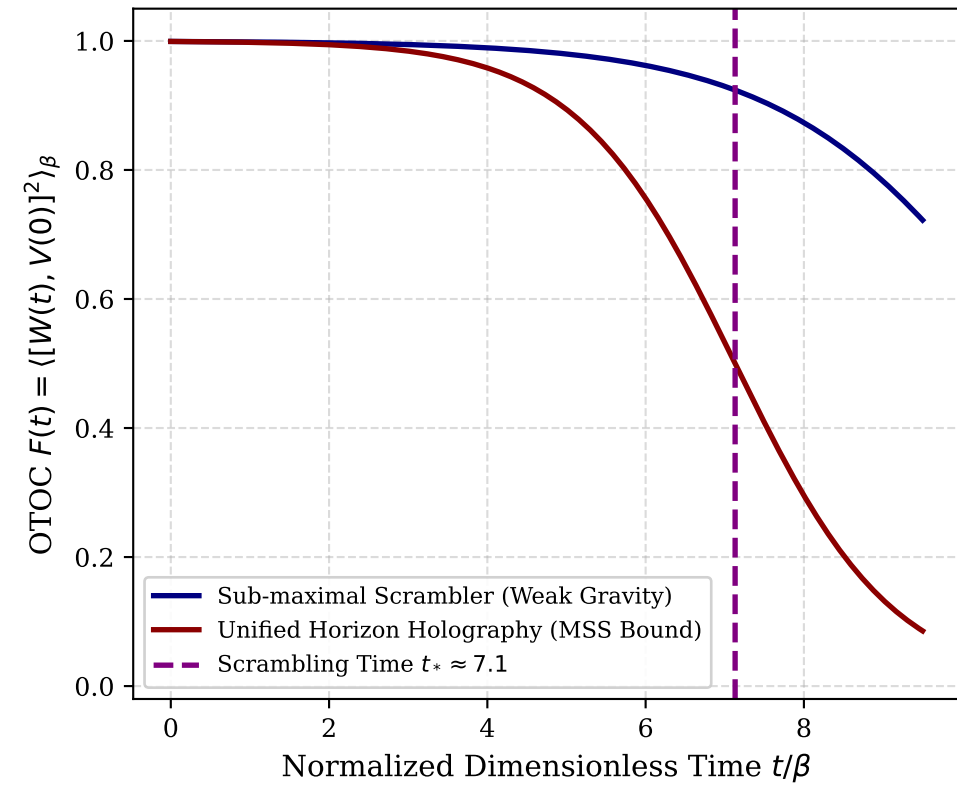
(c) Analog Horizon Chaos in Quantum Simulators
