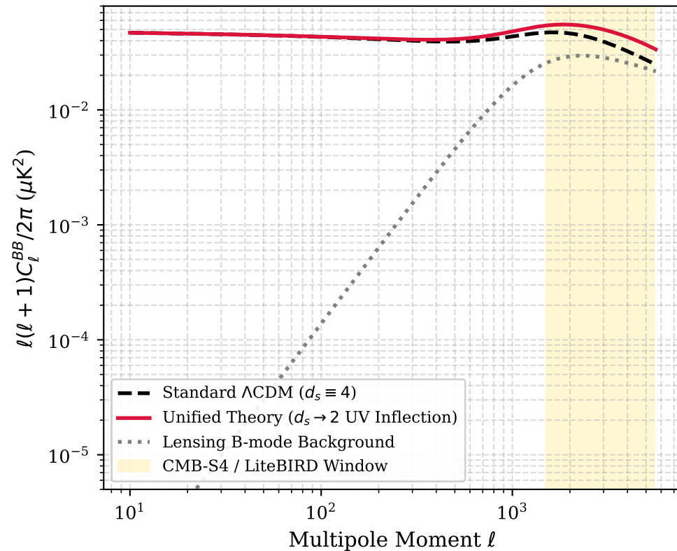
(b) Primordial B -Mode CMB Power Spectrum
