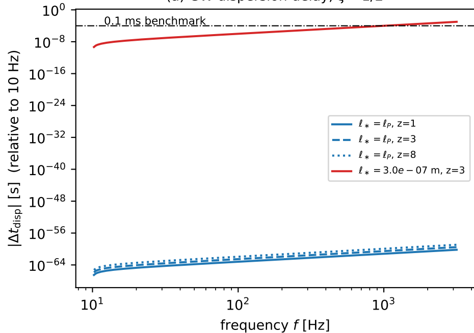
(a) GW dispersion delay, \xi = 1/2
