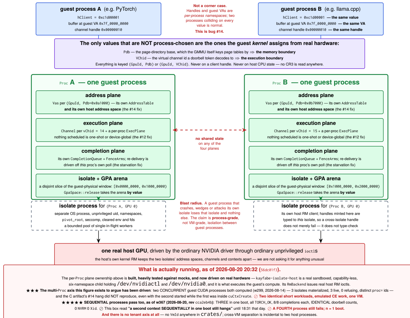
Figure 4: The process and isolation model, and the problem it exists to solve. ★ Two concurrent guest CUDA processes have now been driven through this model on real hardware , each with its own isolate, arena and address space, both computing correctly — so the founding #14 hazard did not reproduce. One VM, two identical short workloads. ★★★★★ And as of 2026-08-20 (w367, §8.11) so have three sequential ones , in one boot, with identical doorbell counts and 8/8 completions each — the model's own cross-process refusal held throughout (a live peer's framebuffer backing was refused by name 132 times), and what was reclaimed was a join no live or dead process named. ☹️ A fourth process still fails; n = 1 boot. The per-Proc ownership of all four planes is built and heavily tested against mocks. ★ The sandboxed isolate process at the bottom is now real — capability-less, six fresh namespaces, holding /dev/nvidiactl and /dev/nvidia0, spawned in response to the guest's own action. ☹️ What remains unexercised is the axis above Proc: there is no tenant identity anywhere in the system, no two-VM run has been attempted, and the serialisation that made the two-process run safe is bounded today only by the hypervisor's big lock — a bound that weakens exactly when the forwarded work gets longer.
