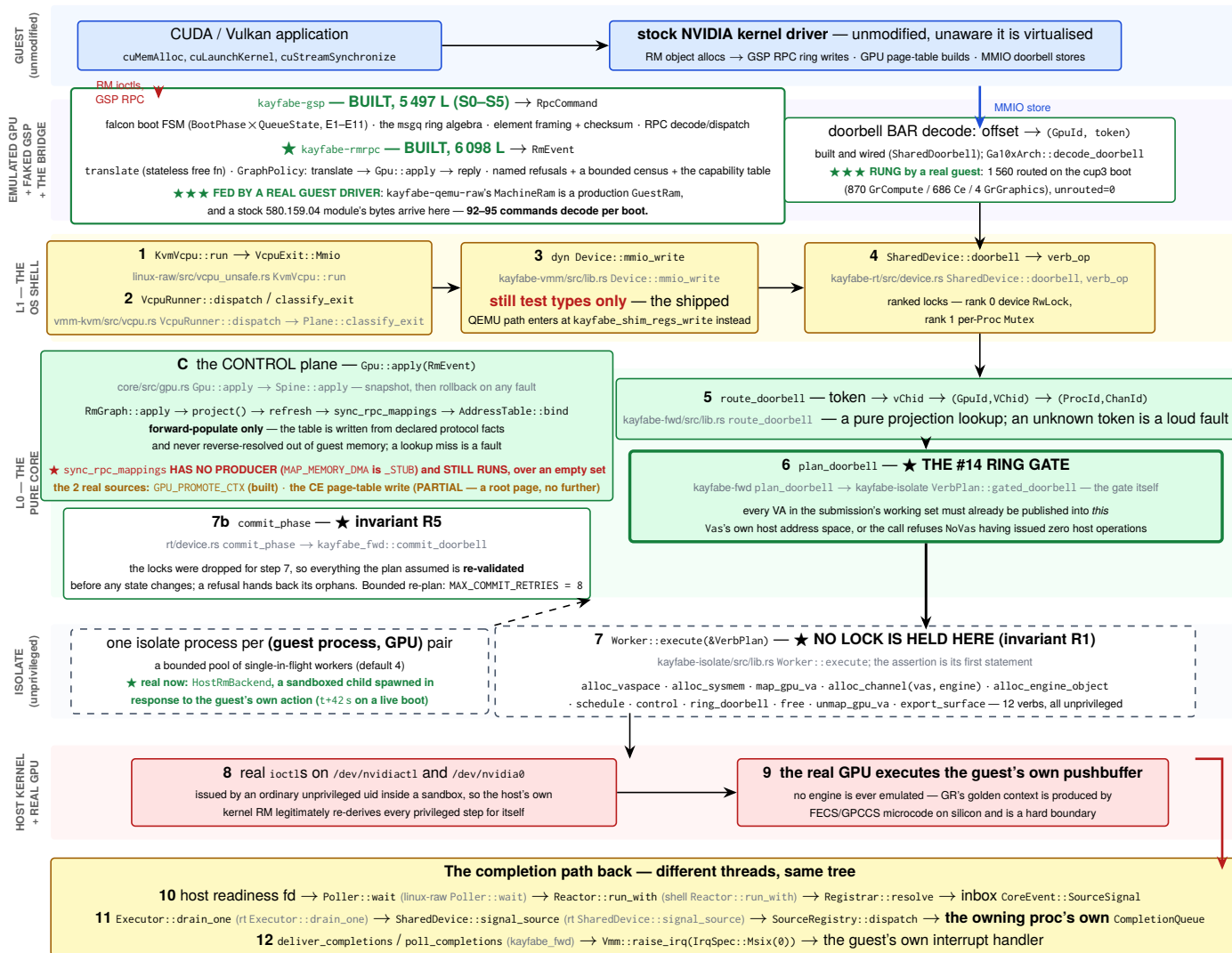
Figure 3: The data path, verified function by function against the tree at 0f577b15. Numbered steps are the execution plane; C is the control plane, which populates the address table from declared protocol facts. Boxes name symbols , not line numbers: the repository converted its own 105 pins to symbols in 3fd1455 after they drifted. What changed at this revision is that most of the red went green — the guest band now really does feed the emulated-device band, the isolate band has a real RmBackend, and steps 7–9 have executed on silicon. The red that is left is the joint : the doorbell box, which is built, wired and has never been rung by a guest. Red text marks what does not exist or has not happened.
