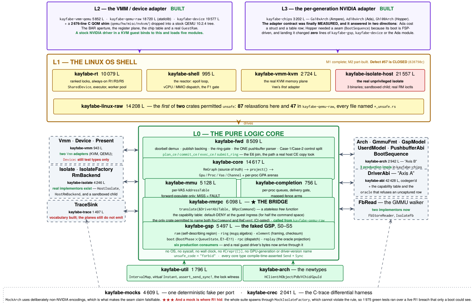
Figure 1: The layer model and the hexagonal ports. Line counts are measured at 0f577b15 (crates/<name>/src/**/*.rs; kayfaber-abi's figure excludes its detached offline generator, 3 284 lines). ★★ ★ The bands inverted at this revision: L2 and L3 were drawn as dashed NOT BUILT boxes at the previous pin and are now built, shipped and booted against. Implementor census, counted from impl <Trait> for across the tree and re-derived rather than carried over: Arch has three production implementations (Ga10xArch, Ad10xArch, Gh100Arch in kayfaber-chips); Isolate, IsolateFactory and RmBackend have real ones in kayfaber-isolate-host; Vmm has two real adapters (KvmVmm, QemuVmm); FbRead, which the previous revision recorded as having no implementation of any kind , has two; GuestRam has a production implementor (MachineRam, in kayfaber-qemu-raw). Device is the one port on this diagram whose only implementors are still test types — the QEMU shell reaches the core through GuestRam and the register plane instead.
