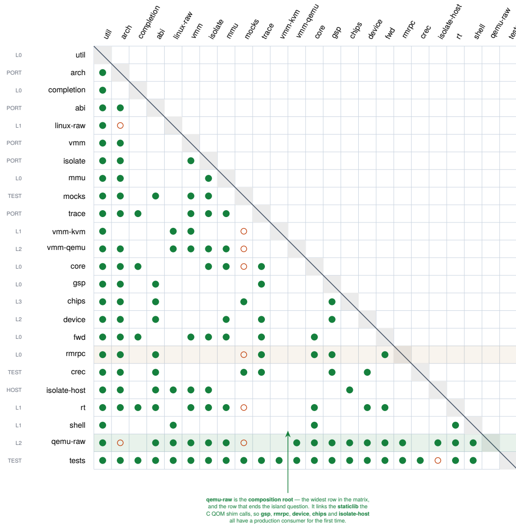
Figure 2: The crate dependency matrix, re-derived from scratch by script from the manifests at 0f577b15 — 24 members , 134 [dependencies] edges and 9 [dev-dependencies] edges that are not already hard edges. kayfabe-qemu-raw (row 23) is the row that matters: it is the composition root, the staticlib a C QOM shim links into a real QEMU, and it depends on eighteen of the twenty-two crates above it. ★ The previous revision's row ordering is no longer topological — qemu-raw has since acquired a dependency on shell, which sat below it — so shell and qemu-raw are swapped here and the strictly-lower-triangular property (which is the acyclicity proof) holds again. Drawn in the old order the matrix would have carried one dot above the diagonal and nothing in the build would have said so.
