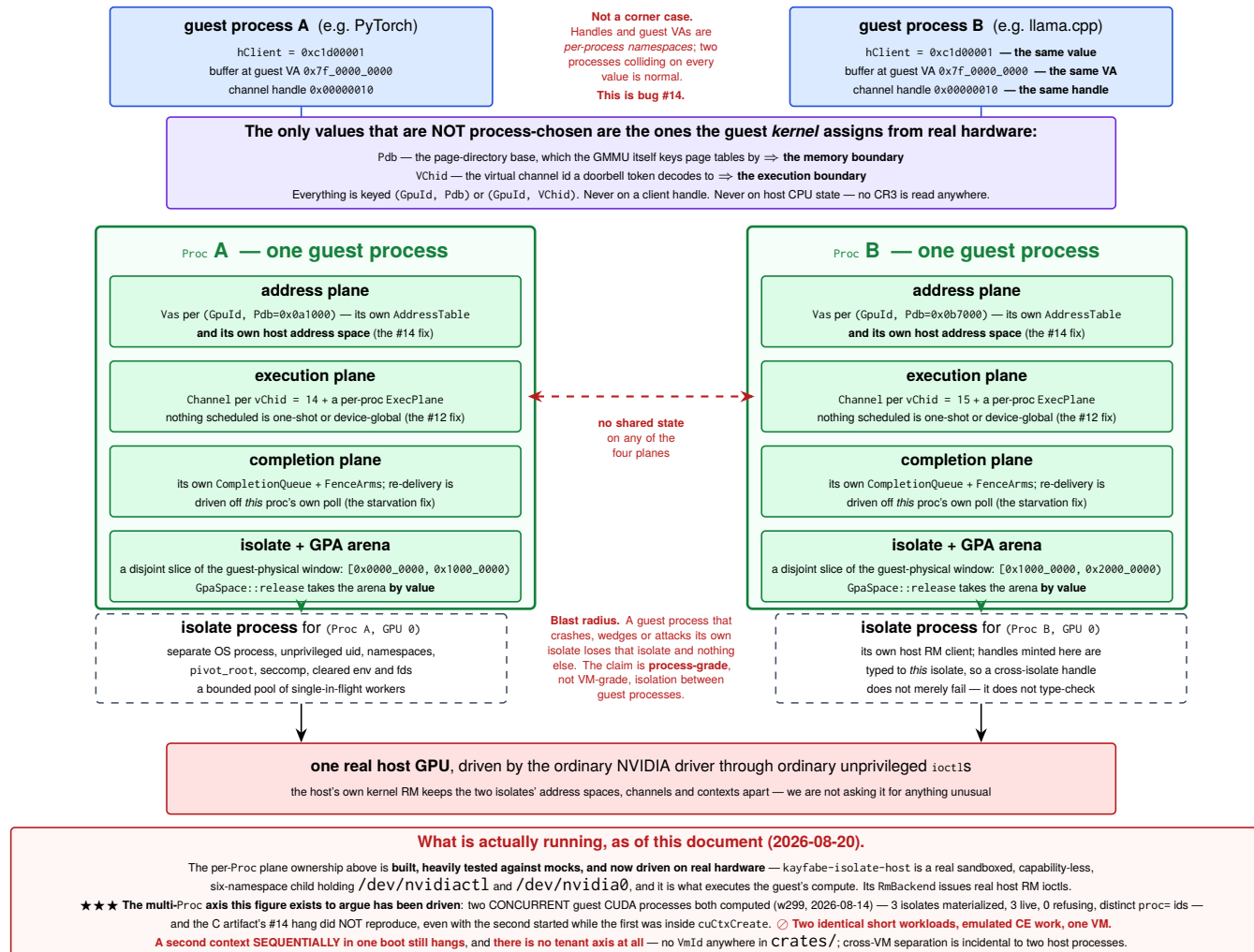
Figure 4: The process and isolation model, and the problem it exists to solve. ★ Two concurrent guest CUDA processes have now been driven through this model on real hardware , each with its own isolate, arena and address space, both computing correctly — so the founding #14 hazard did not reproduce. One VM, two identical short workloads. The per-Proc ownership of all four planes is built and heavily tested against mocks. ★ The sandboxed isolate process at the bottom is now real — capability-less, six fresh namespaces, holding /dev/nvidiactl and /dev/nvidia0, spawned in response to the guest's own action. ☹️ What remains unexercised is the axis above Proc: there is no tenant identity anywhere in the system, no two-VM run has been attempted, and the serialisation that made the two-process run safe is bounded today only by the hypervisor's big lock — a bound that weakens exactly when the forwarded work gets longer.
