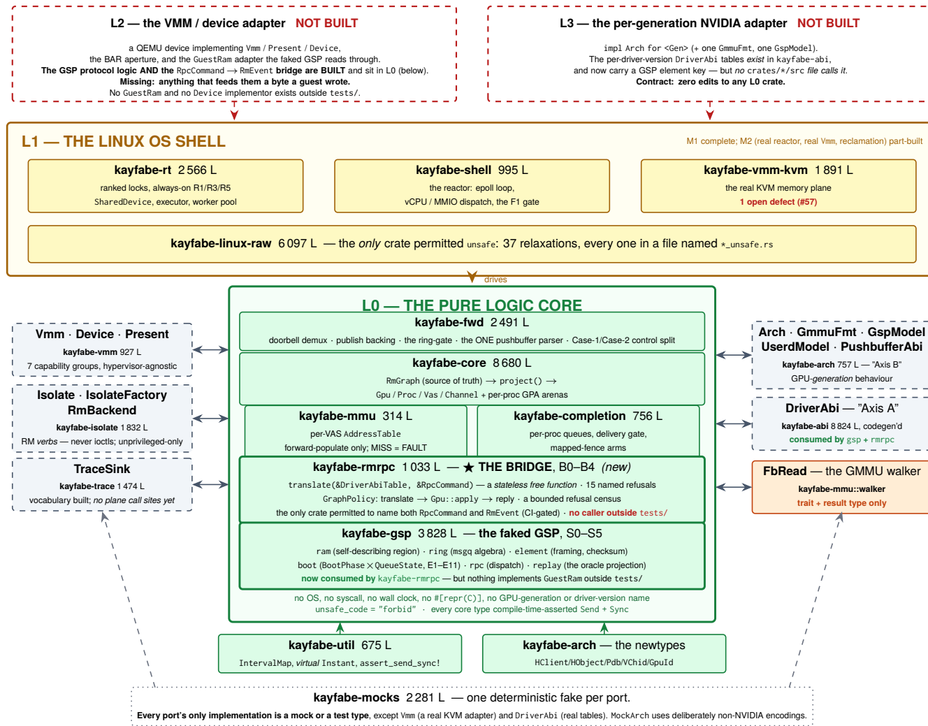
Figure 1: The layer model and the hexagonal ports. Line counts are measured at b612a91 (crates/*/*src/*/*rs; kayfabeshell's figure includes its detached offline generator). Implementor census, counted from impl <Trait> for across the tree: FbRead has no implementation of any kind; Device, Present, Arch, GspModel, Isolate, IsolateFactory and RmBackend have only mocks or test types; Vmm has one real adapter (KvmVmm); TraceSink has three in-crate implementations; CommandPolicy has two, one of which (GraphPolicy) is the new bridge and is production code. kayfabermrpc joined the L0 band at this revision, between gsp and core — but the L2 shell that would feed either of them still does not exist.
