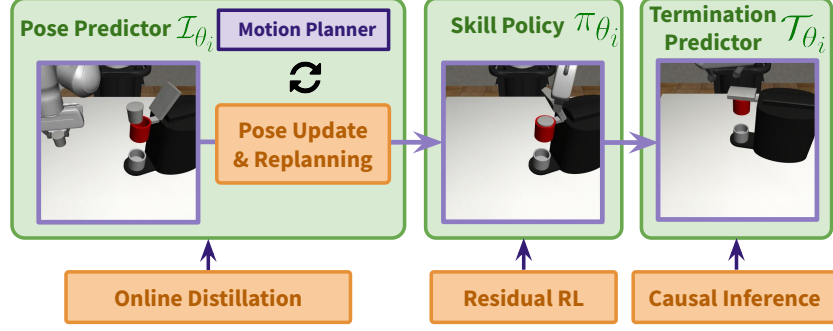
Figure 2: The three main components of a ReinforceGen stage. The pose predictor \mathcal{I}_{\theta_i} predicts the target end-effector pose and updates the goal of the motion planner in real-time. After reaching the destination, the skill policy \pi_{\theta_i} takes control to complete the stage goal, which is determined by the termination predictor \mathcal{T}_{\theta_i} . All three components are first trained offline with supervised learning and then fine-tuned with online data.
