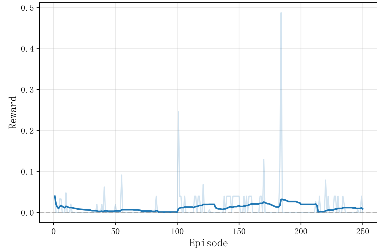
Alignment Reward
