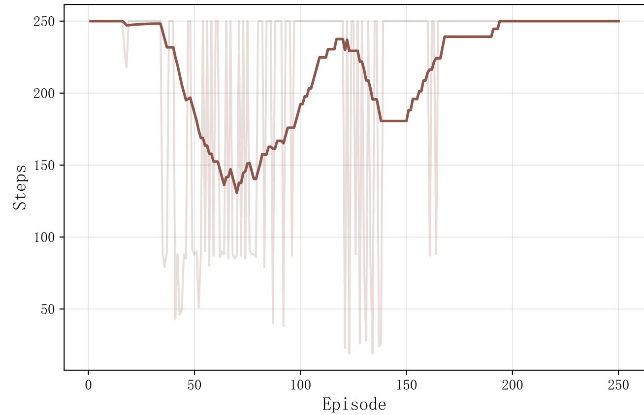
Episode Length
