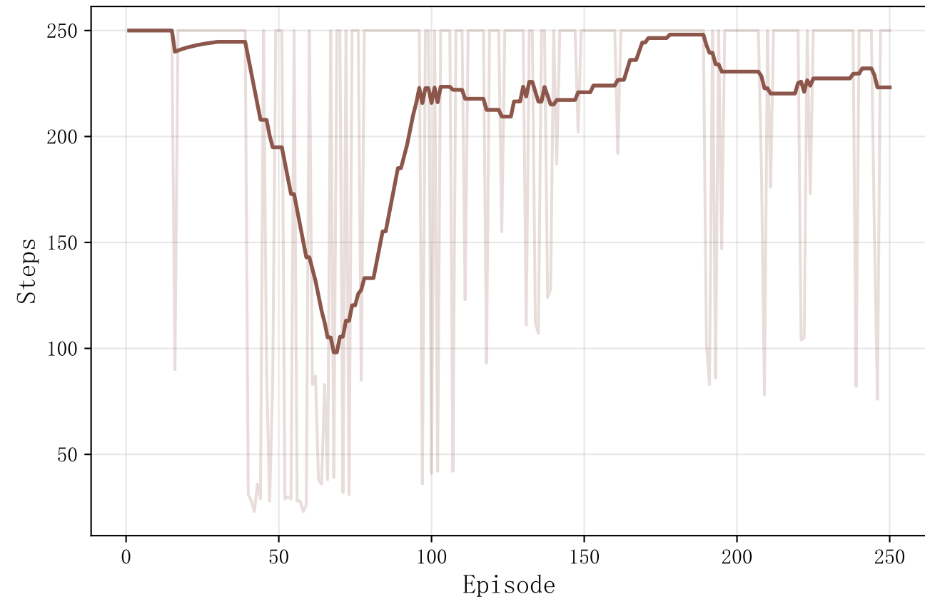
Episode Length
