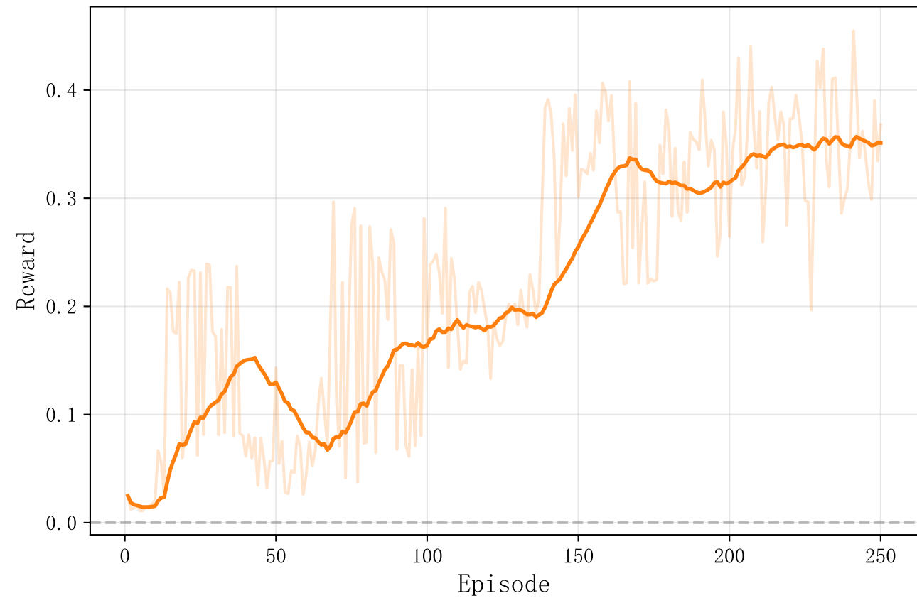
Alignment Reward
