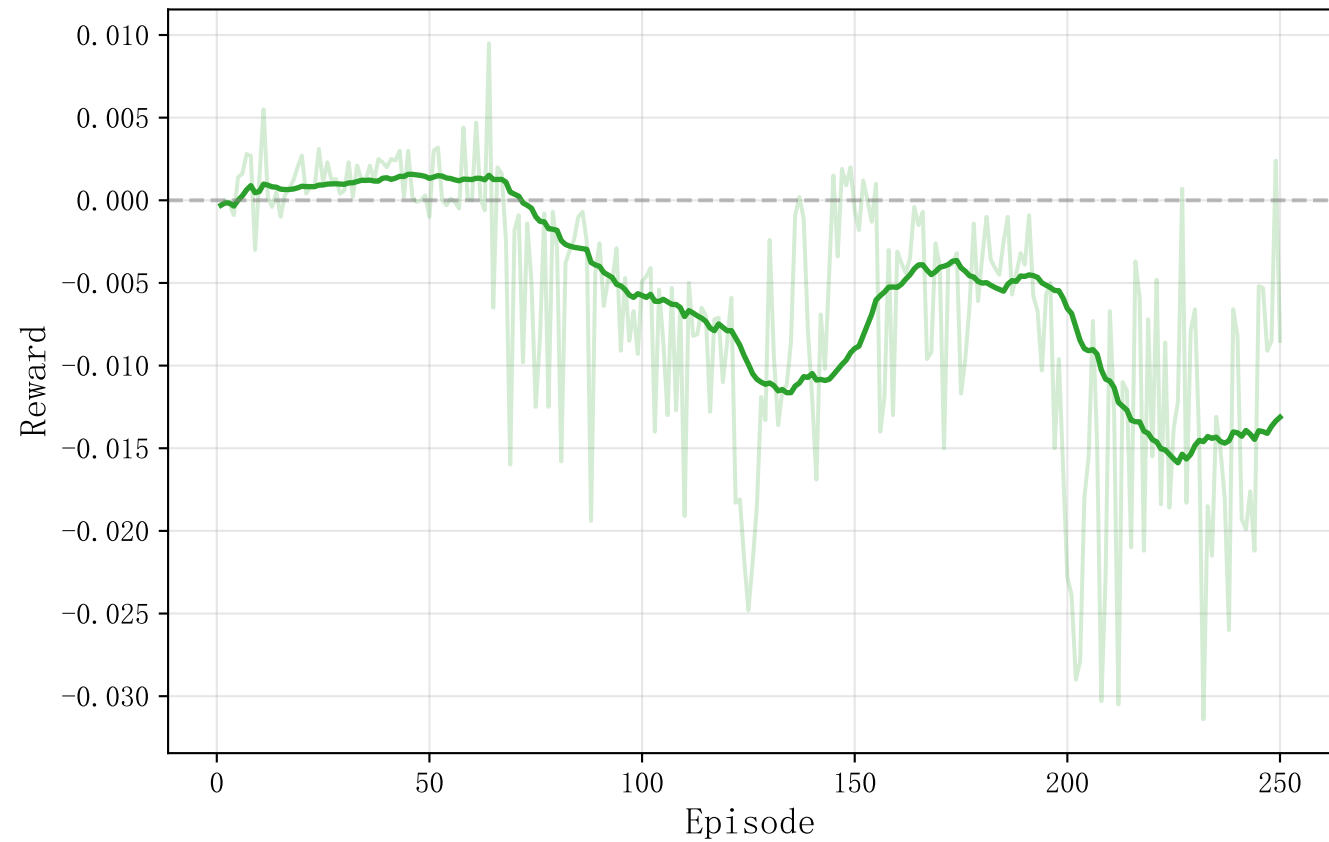
Escape Reward
