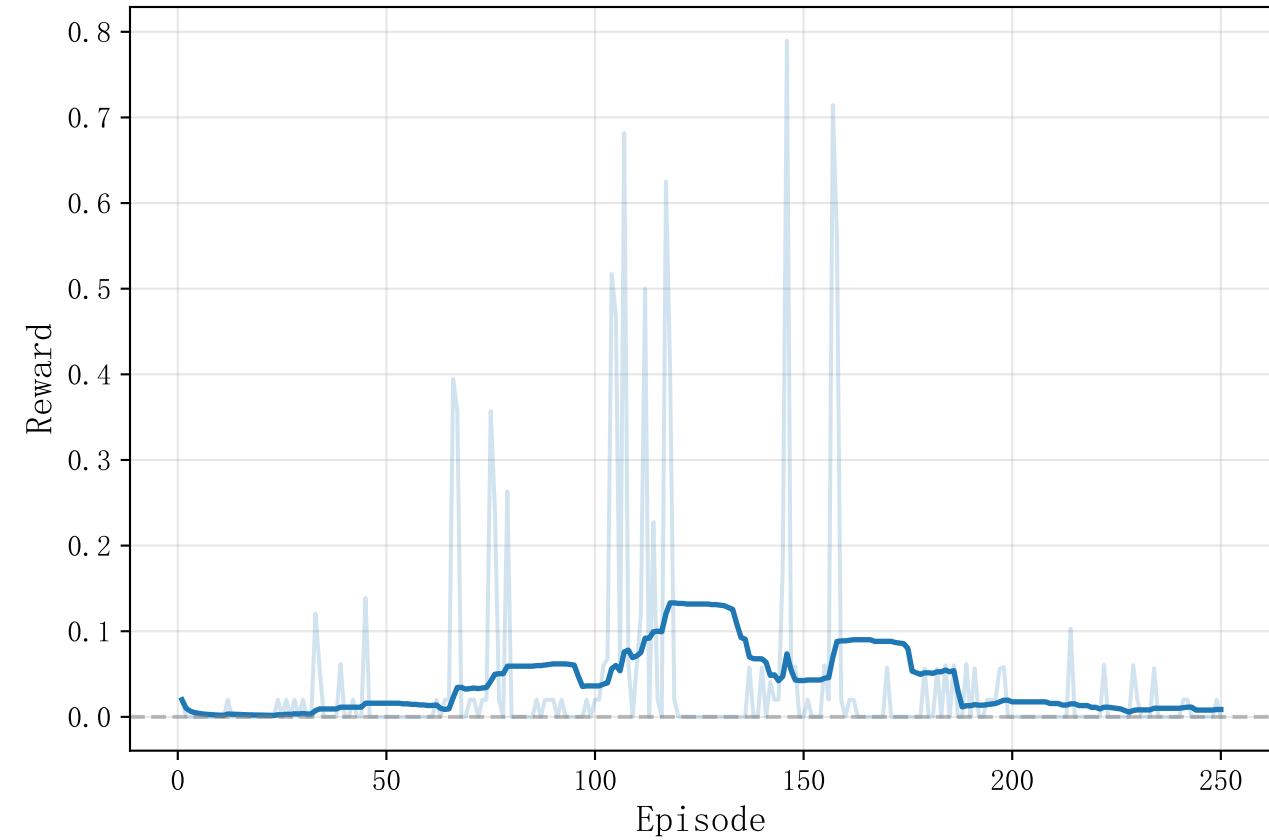
Alignment Reward
