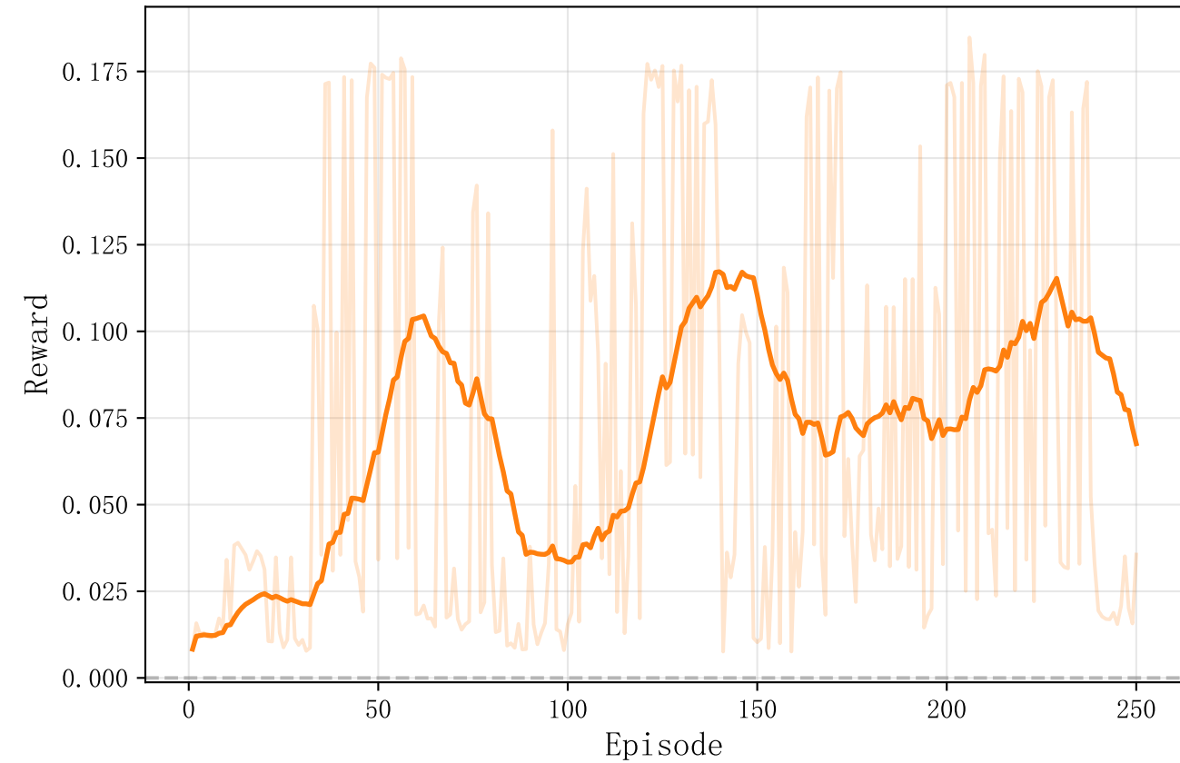
Alignment Reward
