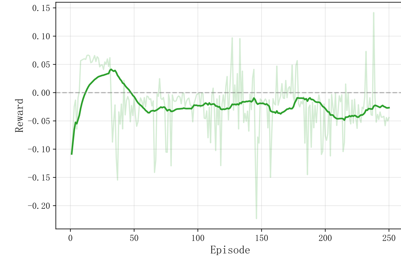
Escape Reward
