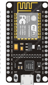
ESP-12E Dev. Board Pinout
