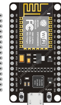
ESP-12E Dev. Board Pinout
