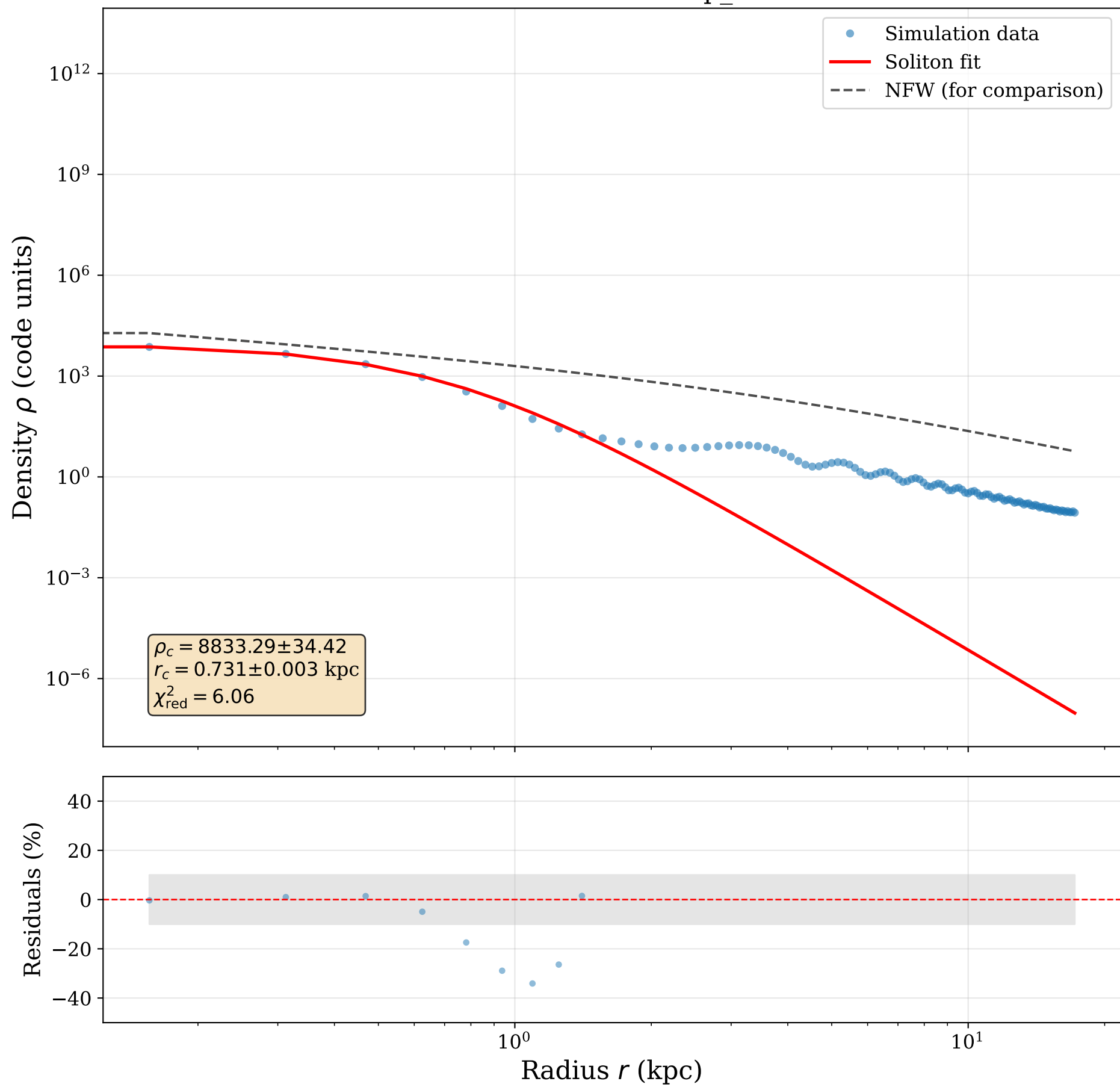
Soliton Core Profile: snap_0100.h5
