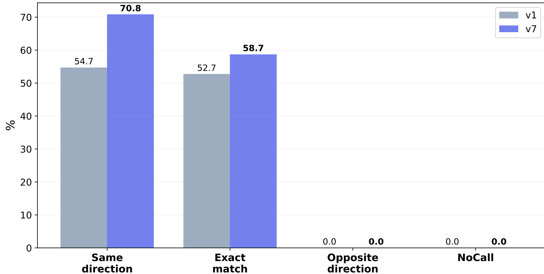
Headline concordance metrics: v1 vs v7
