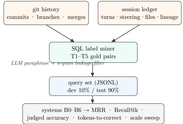
Figure 2: RekalBench pipeline. Labels are mined from structure the tool already records; paraphrase plus an n-gram overlap filter breaks lexical leakage between query and target.
