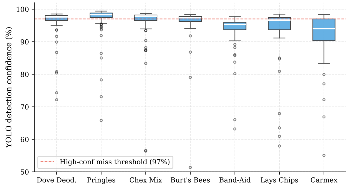
Detection confidence distribution by class
