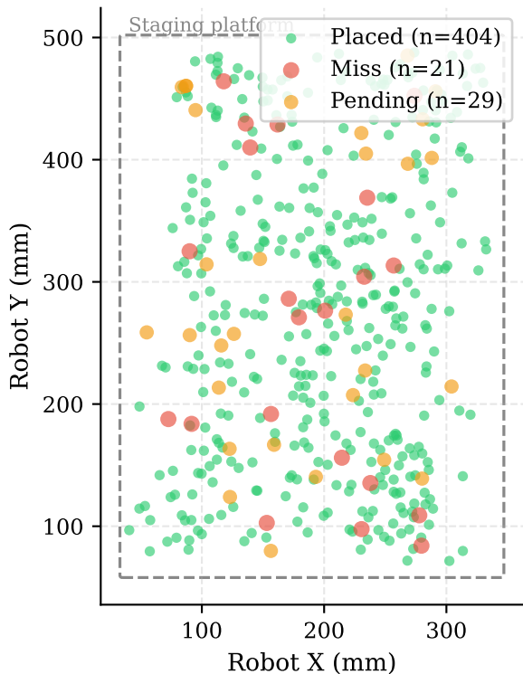
Pick target positions on staging platform (colored by pick outcome)
