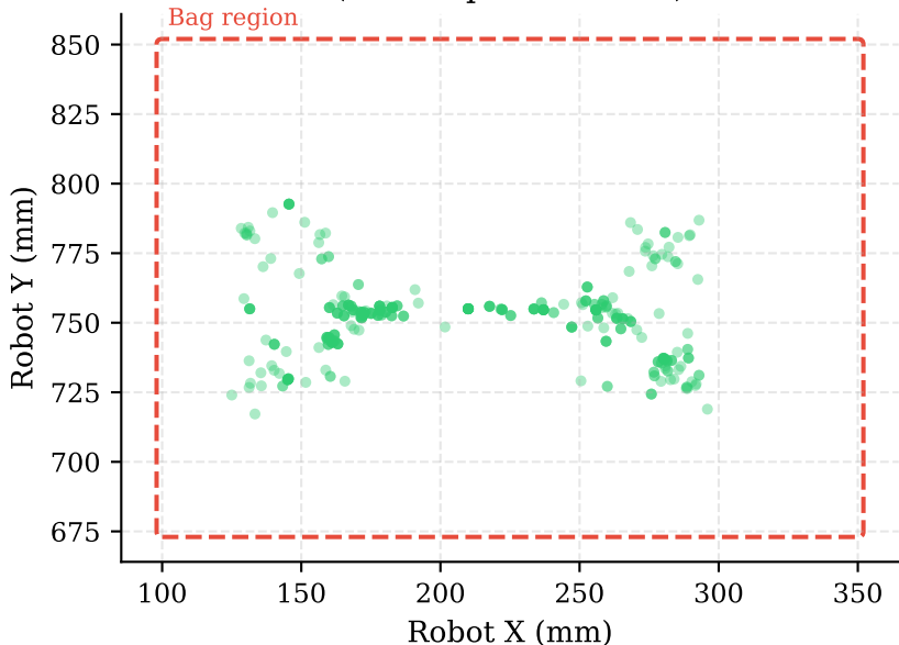
Planned placement positions in bag (n=404 placed items)
