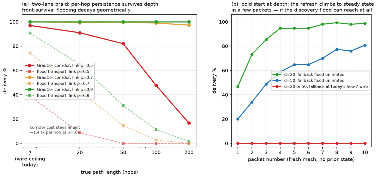
Figure 16. Depth stress test on synthetic braids (300 packets per point). (a) Two-lane braid: warm-gradient corridor delivery (solid) vs unlimited-hop flood transport (dashed) as true path length grows from 7 to 200 hops, per link quality. Persistence per hop survives depth at linear cost; front-survival flooding decays geometrically. (b) Cold start on a fresh mesh ( w=2 , p=0.7 ): per-packet delivery as the refresh plants state — fast ramp to steady state once the discovery flood can reach at all; at today's hop-7 wire ceiling, depth > 7 cold start is zero for any protocol.
