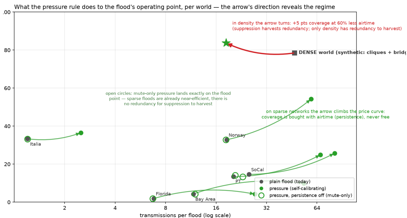
Figure 19. What the pressure rule does to the plain flood's operating point, per world (arrow: flood → pressure in airtime/coverage space). On all six sparse production networks the arrow climbs the price curve — coverage is bought with persistence airtime, never free — and the mute-only variant (open circles) lands exactly on the flood point, confirming sparse floods are already near-efficient. In the dense world — a synthetic construction, since no network in our dataset exhibits this regime — the arrow turns up-and-left: suppression harvests redundancy, and only density has redundancy to harvest. The rule needs no telling which case it is in.
