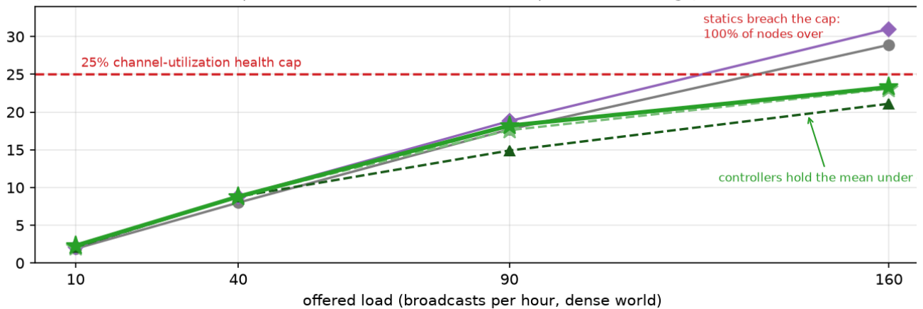
Figure 23. Headroom control under rising offered load (dense world). (a) Coverage: the setpoint controller fills the allowed airtime and takes the best compliant coverage at every load; the threshold ladders defend the cap and retreat earlier. (b) Mean channel utilization against the 25% health cap: every static policy crosses it at saturating load, the controllers stay under.
