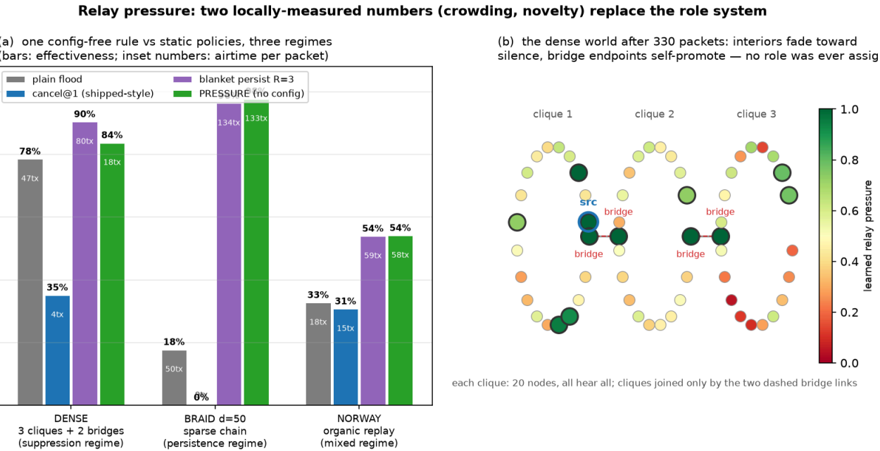
Figure 20. Relay pressure. (a) Effectiveness (bars) and airtime (inset) for three static policies and the pressure rule across the three regimes — each regime's best static differs, pressure tracks it everywhere. (b) The dense world after 330 packets, node colour = learned pressure: clique interiors fade toward silence while all four bridge endpoints self-promote to maximum pressure. The role system's job — deciding who relays with what priority — has been performed by measurement.
