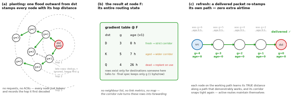
Figure 2. How each node builds its two numbers. (a) The planting flood expands outward from the destination; every node records the hop count at which it first decoded it — late copies are ignored by packet-ID dedup, so g is the shortest observed distance. Nothing is requested and nothing is acknowledged. (b) The result at one node: a table row per active destination; the age column and its lifecycle notes are v1 — the final spec keeps only g (§3.6). (c) When a packet is delivered, every node on the path it actually took is re-stamped with its distance along that proven path and age 0 — riding the existing delivery confirmation, so active conversations keep their own gradients sharp at zero airtime cost.
