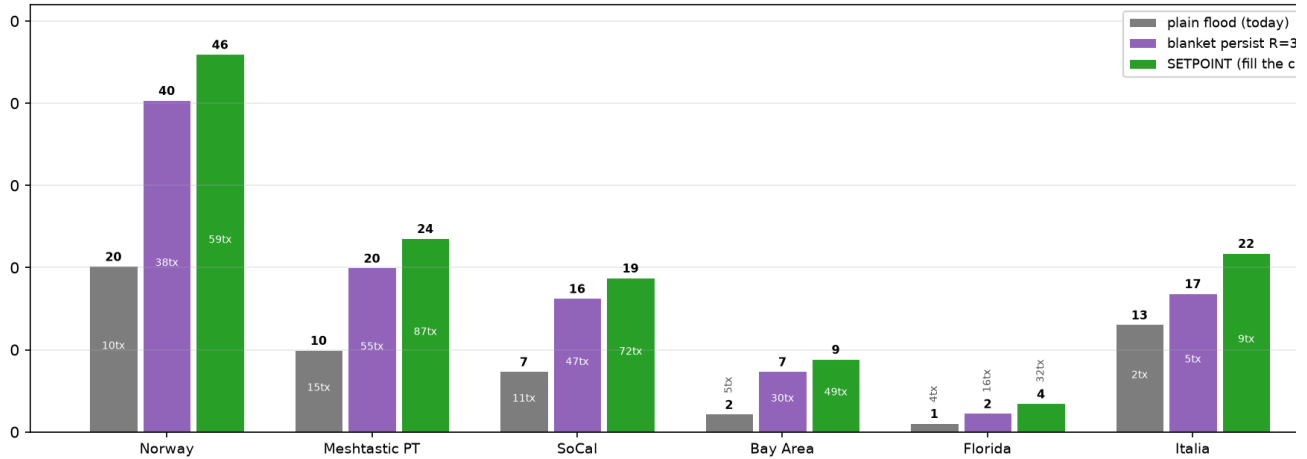
Figure 24. The setpoint controller on all six production networks (20 broadcasts/hour, per-network calibration, utilization-tracked): best coverage everywhere, cap never approached (utilization \leq 0.2\% on every network), dense-regime retreat never triggered — the controller validates as safe on real sparse meshes while its cap-enforcement value lives in the dense regime of Figure 23.
