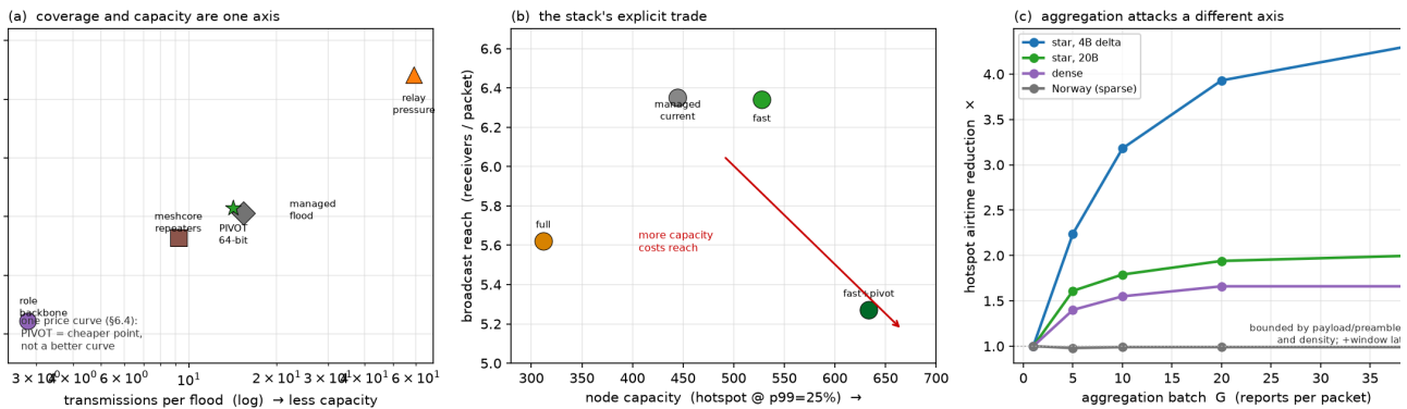
Figure 18. The coverage-capacity-load tension. (a) Every Norway broadcast policy is a point on one airtime→coverage price curve; PIVOT is a cheaper point (more capacity, less coverage), not a better curve. (b) The integrated stack’s explicit trade: fast+PIVOT raises node capacity but lowers broadcast reach; full mode raises reliability but cuts capacity. (c) Aggregation attacks a different axis — hotspot airtime reduction vs batch size G —
