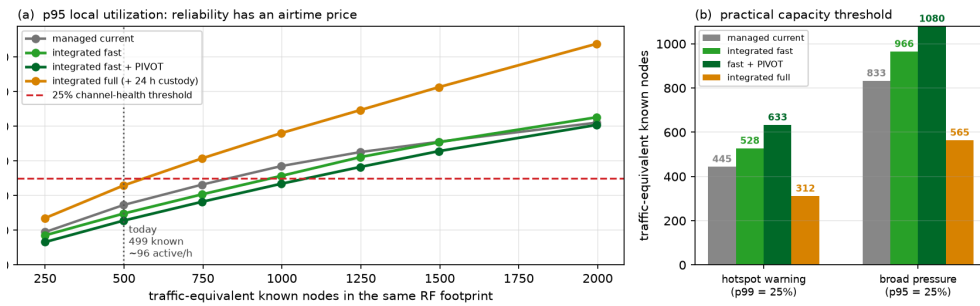
Figure 25. The complete stack under production-shaped load (identical event schedules, three seeds). (a) P95 local utilization: integrated fast+PIVOT combines every airtime-saving mechanism and stays lowest; integrated-full adds 24-hour custody and trades capacity for reliability. (b) The 25% thresholds make the policy boundary explicit: fast+PIVOT expands hotspot / broad capacity 42% / 30%; universal custody contracts them 30% / 32%. Counts assume the same RF footprint and per-node traffic; geographic growth with spatial reuse does not obey this x-axis.
