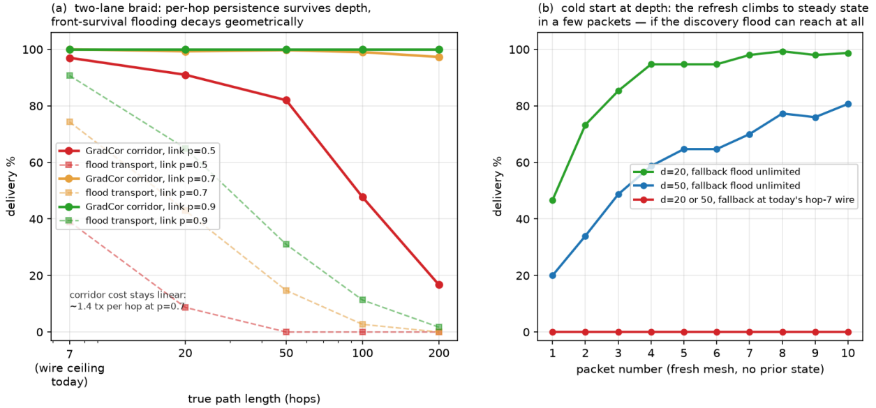
Figure 19. Depth stress test on synthetic braids (300 packets per point). (a) Two-lane braid: warm-gradient corridor delivery (solid) vs unlimited-hop flood transport (dashed) as true path length grows from 7 to 200 hops, per link quality. Persistence per hop survives depth at linear cost; front-survival flooding decays geometrically. (b) Cold start on a fresh mesh ( w=2 , p=0.7 ): per-packet delivery as the refresh plants state — fast ramp to steady state once the discovery flood can reach at all; at today's hop-7 wire ceiling, depth > 7 cold start is zero for any protocol.
