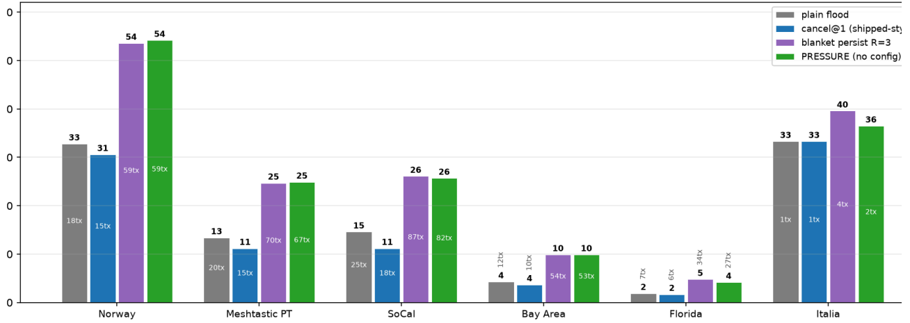
Figure 21. Relay pressure on the six production networks (per-network calibration, every node allowed to relay, 30-packet warm-up). Bars: coverage of BFS-reachable online nodes; insets: transmissions per flood. The self-calibrating rule tracks the best static policy on each network without knowing which network it is on.
