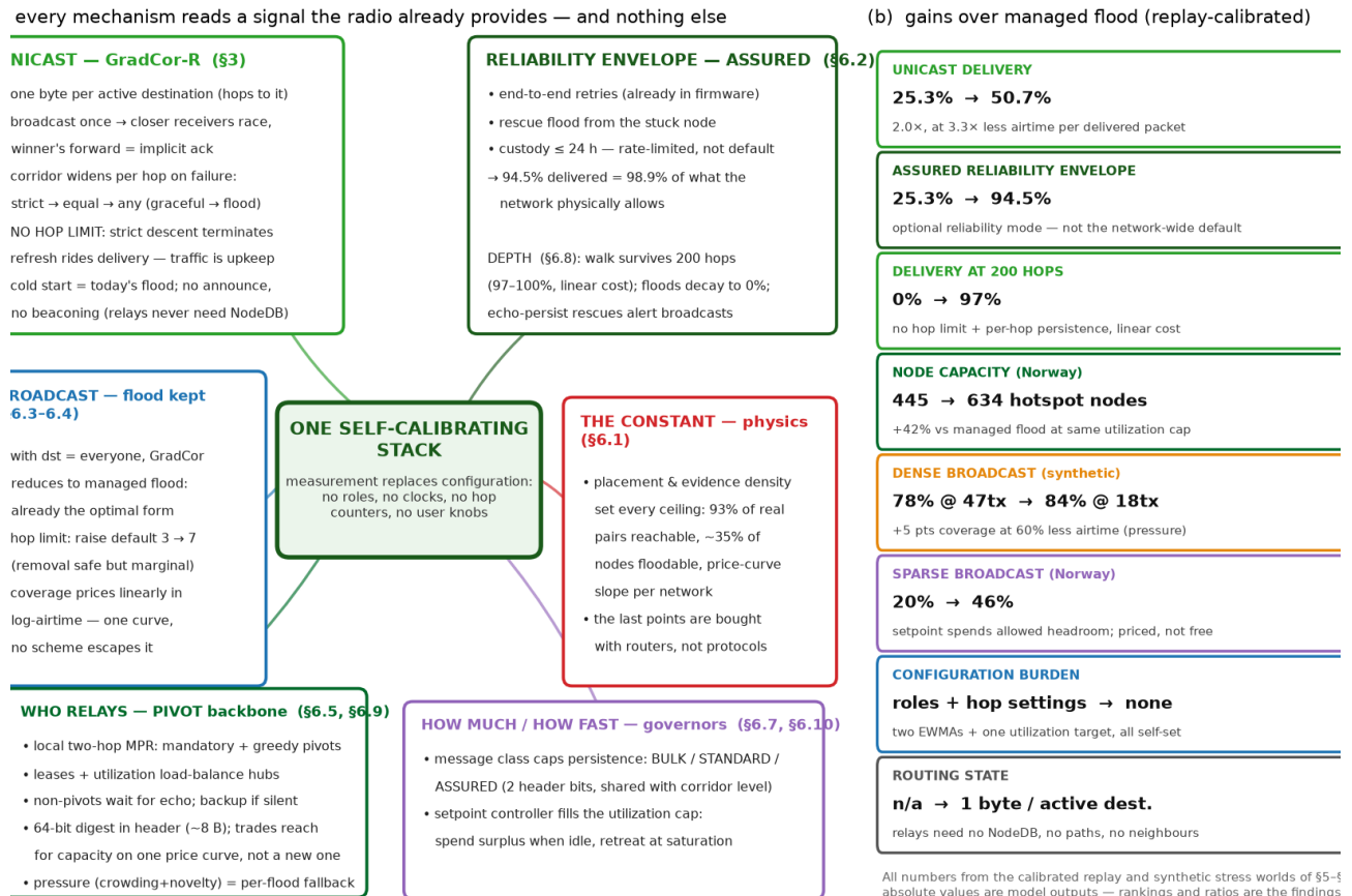
Figure 26. The complete stack and its measured gains. (a) All mechanisms of §3-§6 as one system, each annotated with its section: unicast routing, its rate-limited ASSURED reliability envelope, the broadcast side, and the three self-calibrating governors, resting on the one thing no protocol changes — physical placement. (b) Gains over managed flood, one line per claim, each traceable to a table in the body. Absolute values are model outputs; rankings and ratios are the findings.
