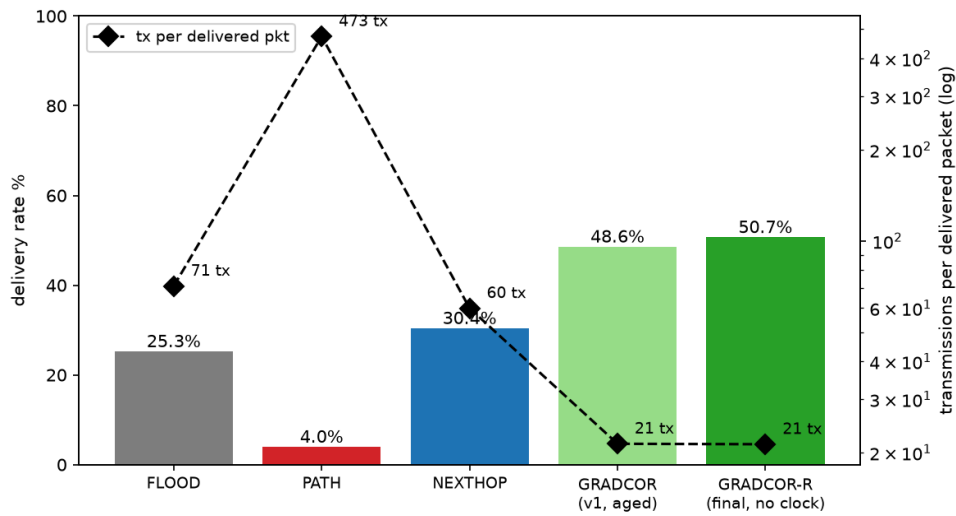
Figure 11. Delivery rate (bars, left axis) and airtime cost per delivered packet (diamonds, right axis, log scale), with both GradCor forms side by side. GradCor-R dominates flooding on both axes simultaneously: +25.4 points of delivery (2.0×) at 3.3\times less airtime per delivered packet — with no state clocks.
