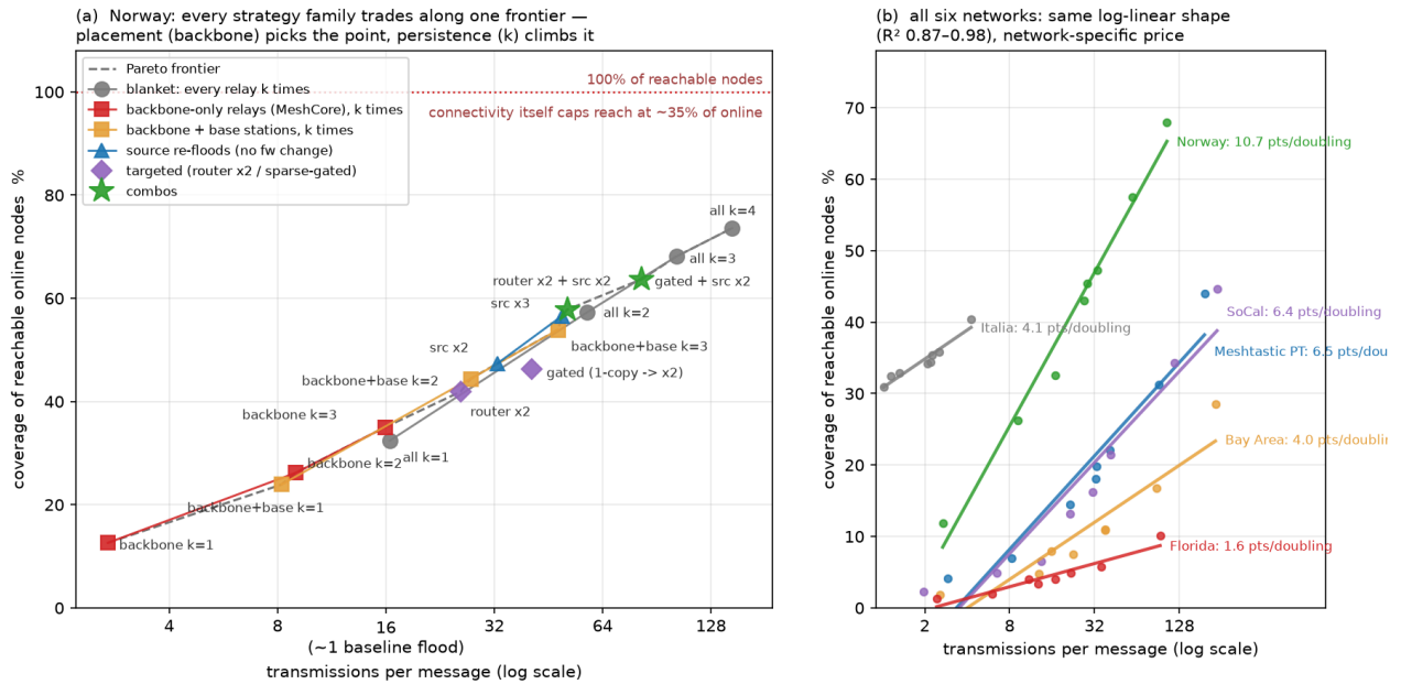
Figure 16. The all-to-all delivery strategy space. (a) Norway (900 floods per point): coverage of BFS-reachable online nodes vs transmissions per message (log scale). Families: blanket persistence (every relay k times), infrastructure-only relaying (MeshCore pattern, with and without fixed base stations), source re-floods, targeted and gated variants and combos. All families track one Pareto frontier (dashed): placement chooses a point on the curve, persistence climbs it and no adaptive rule beats it — consistent with §6.3's finding that without a destination there is nothing to steer by. (b) The same reduced grid on all six networks: the log-linear shape is universal (fitted lines, R^2 0.87–0.98) while the slope — what a doubling of airtime buys — is a network property, ordered exactly by the evidence density of Table 4.
