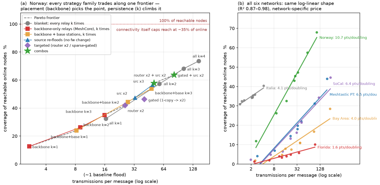
Figure 15. The all-to-all delivery strategy space. (a) Norway (900 floods per point): coverage of BFS-reachable online nodes vs transmissions per message (log scale). Families: blanket persistence (every relay k times), infrastructure-only relaying (MeshCore pattern, with and without fixed base stations), source re-floods, targeted and gated variants, and combos. All families track one Pareto frontier (dashed): placement chooses a point on the curve, persistence climbs it and no adaptive rule beats it — consistent with §6.3's finding that without a destination there is nothing to steer by. (b) The same reduced grid on all six networks: the log-linear shape is universal (fitted lines, R^2 0.87–0.98) while the slope — what a doubling of airtime buys — is a network property, ordered exactly by the evidence density of Table 4.
