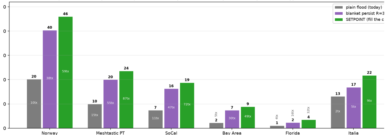
Figure 22. The setpoint controller on all six production networks (20 broadcasts/hour, per-network calibration, utilization-tracked): best coverage everywhere, cap never approached (utilization \leq 0.2\% on every network), dense-regime retreat never triggered — the controller validates as safe on real sparse meshes while its cap-enforcement value lives in the dense regime of Figure 21.
