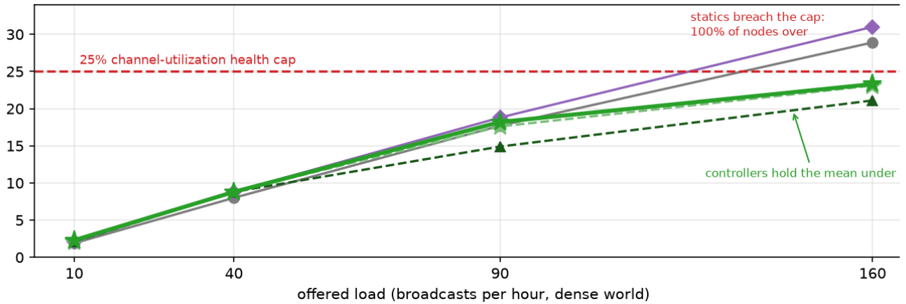
Figure 21. Headroom control under rising offered load (dense world). (a) Coverage: the setpoint controller fills the allowed airtime and takes the best compliant coverage at every load; the threshold ladders defend the cap and retreat earlier. (b) Mean channel utilization against the 25% health cap: every static policy crosses it at saturating load, the controllers stay under.
