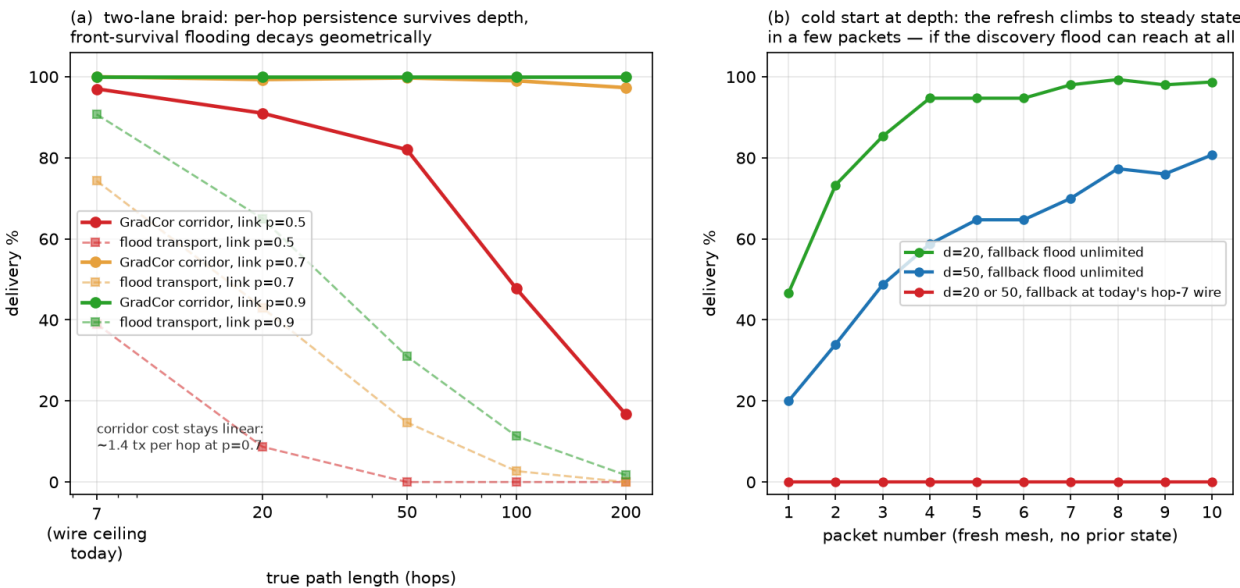
Figure 17. Depth stress test on synthetic braids (300 packets per point). (a) Two-lane braid: warm-gradient corridor delivery (solid) vs unlimited-hop flood transport (dashed) as true path length grows from 7 to 200 hops, per link quality. Persistence per hop survives depth at linear cost; front-survival flooding decays geometrically. (b) Cold start
