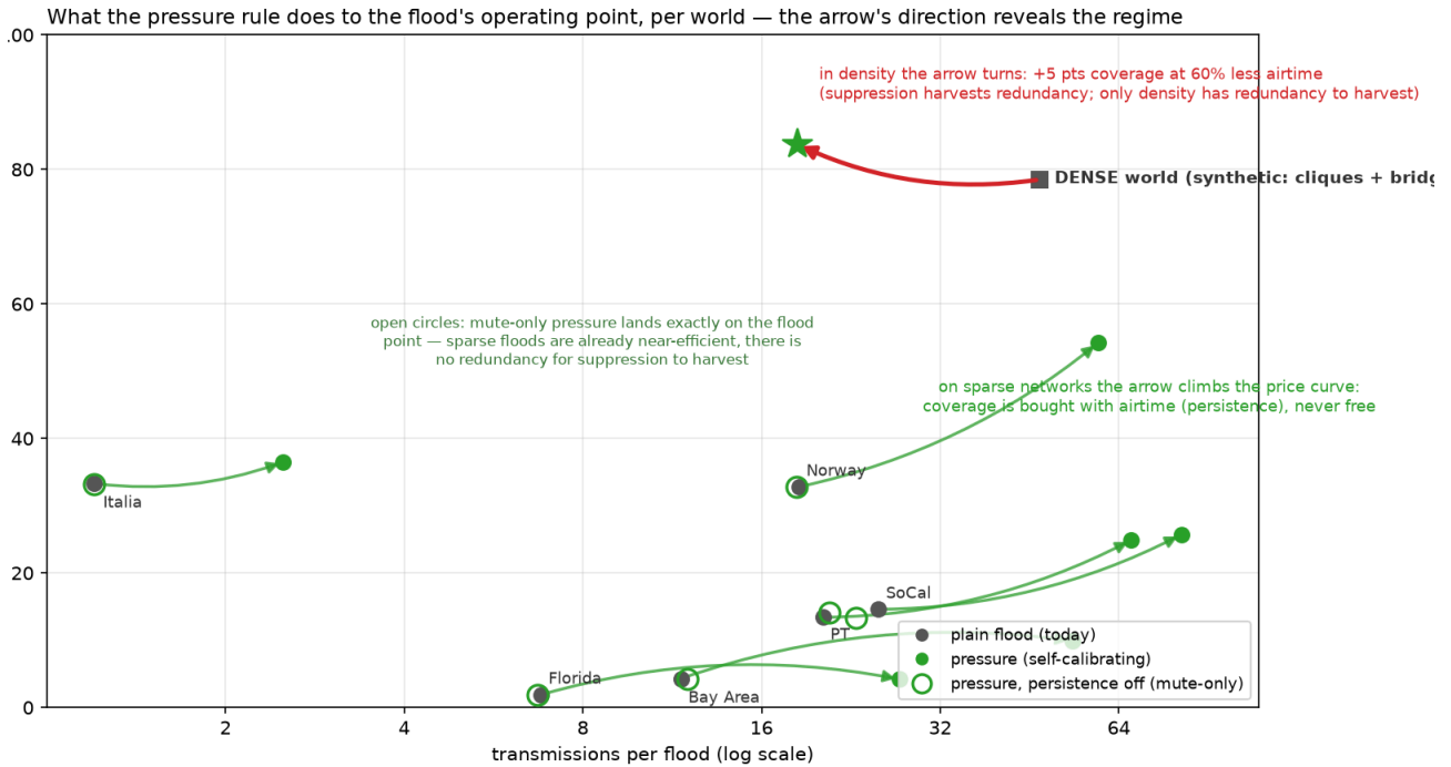
Figure 20. What the pressure rule does to the plain flood's operating point, per world (arrow: flood → pressure in airtime/coverage space). On all six sparse production networks the arrow climbs the price curve — coverage is bought with persistence airtime, never free — and the mute-only variant (open circles) lands exactly on the flood point, confirming sparse floods are already near-efficient. In the dense world — a synthetic construction, since no network in our dataset exhibits this regime — the arrow turns up-and-left: suppression harvests redundancy, and only density has redundancy to harvest. The rule needs no telling which case it is in.
