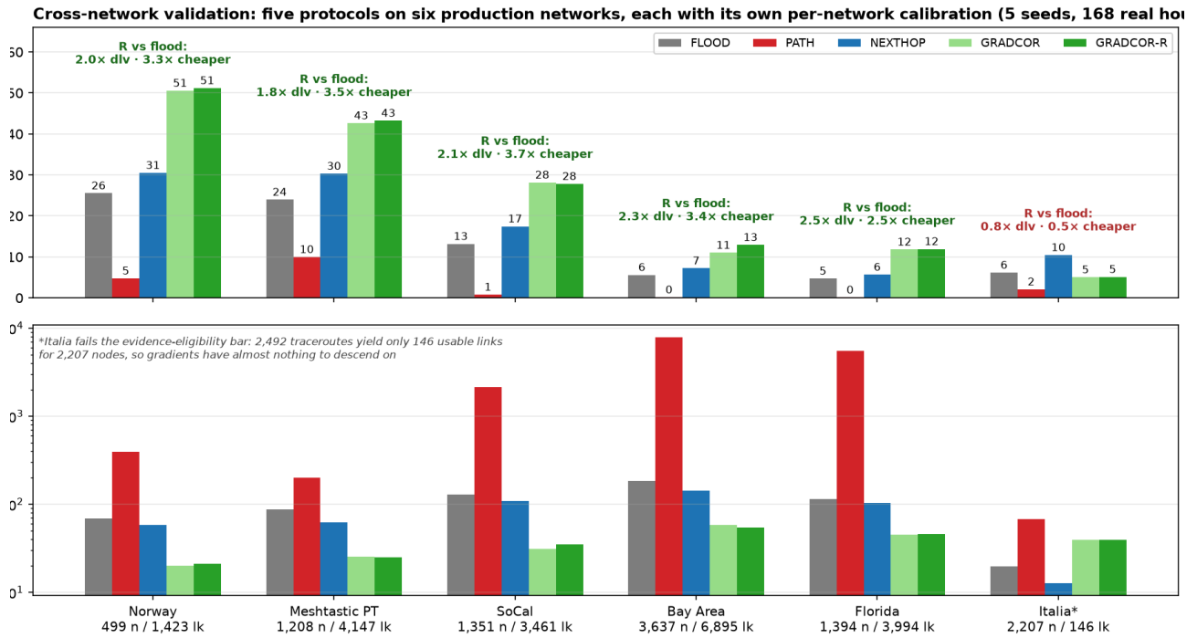
Figure 13. Cross-network validation on six production networks (5 seeds each, same 168-hour week, per-network calibration). Top: delivery rate; bottom: airtime per delivered packet (log). On every network with adequate traceroute evidence the ranking is identical — GradCor-R \approx GradCor v1 > NEXTHOP > FLOOD >> PATH — with GradCor-R delivering 1.8–2.5 \times flood's rate at 2.5–3.7 \times less airtime per delivered packet. Italia (starred) is the honest boundary case: its 2,492 traceroutes yield only 146 usable links for 2,207 nodes, gradients have almost nothing to descend on and gradient routing degrades to flood level while NEXTHOP's simpler cache wins.
