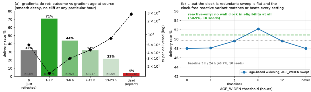
Figure 5. Clock ablation on the Norway replay. (a) Outcome by gradient age at the source (baseline protocol, 3 seeds): usefulness decays smoothly — staleness is real but has no characteristic hour. (b) Delivery is nearly flat across the entire widening-threshold sweep (blue) and the clock-free reactive variant (green, 10 seeds) matches or beats every fixed setting: the per-hop escalation already measures staleness at the moment it matters. One caveat: this network's churn is duty-cycle-dominated with a stable router backbone; in a high-mobility mesh, wall-clock aging could recover value.
