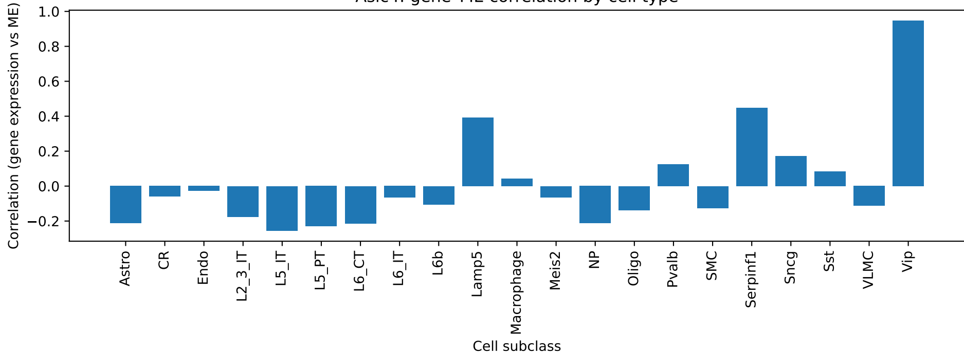
Asic4: gene-ME correlation by cell type
