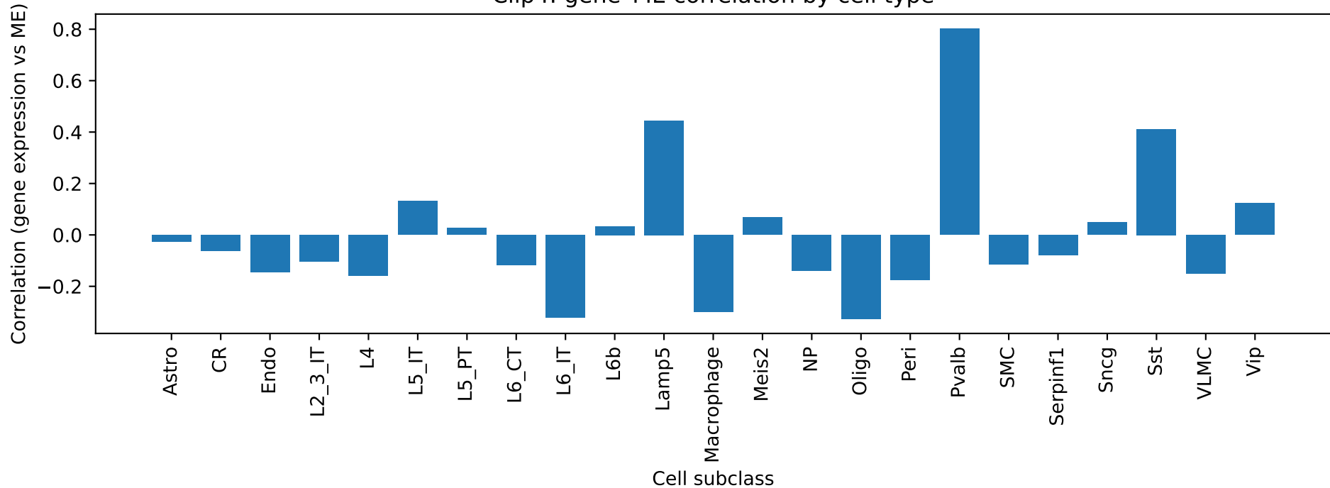
Clip4: gene-ME correlation by cell type
