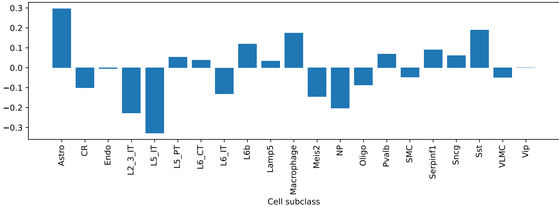
Gm14418: exon ENSMUSG00000078867_ProteinCoding_2 ME correlation by cell type
