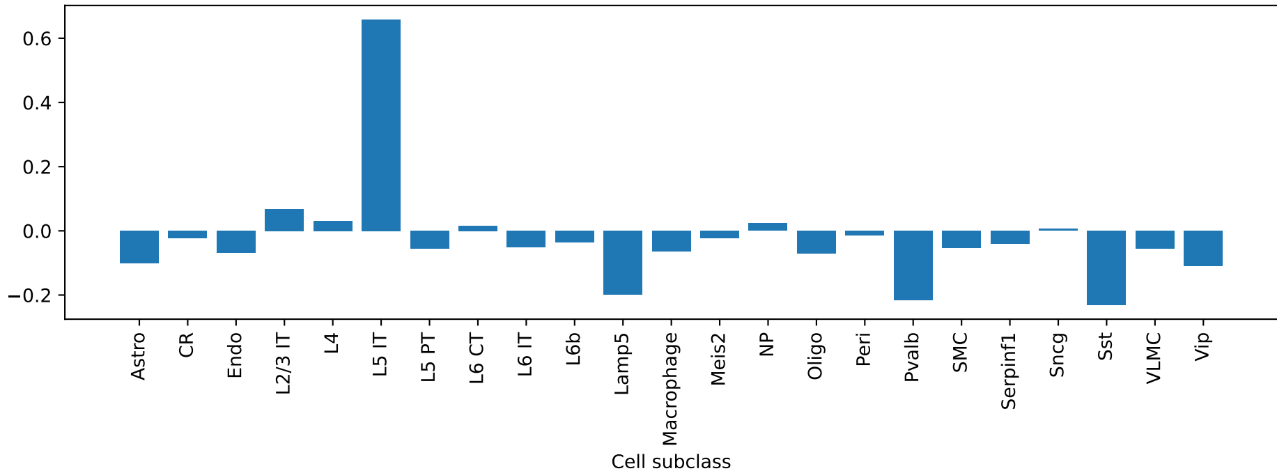
Tpd52l1: exon ENSMUSG00000000296_ProteinCoding_5 correlation by cell type
