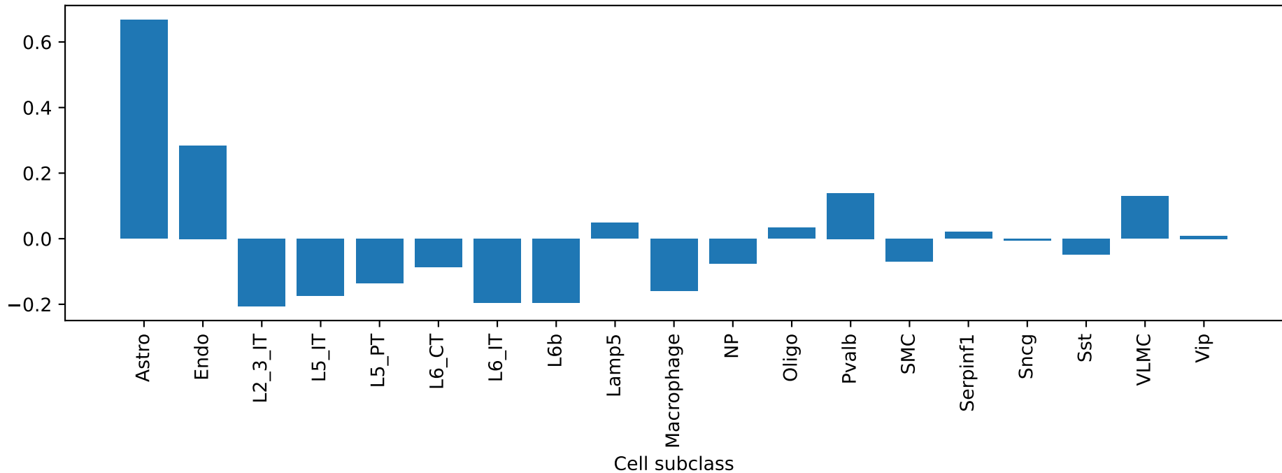
Fars2: exon ENSMUSG00000021420_ProteinCoding_2 ME correlation by cell type
