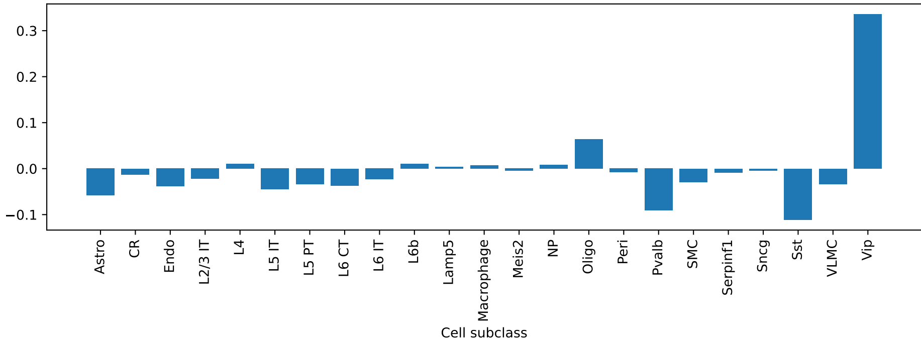
Csmd3: exon ENSMUSG00000022311_ProteinCoding_2 correlation by cell type
