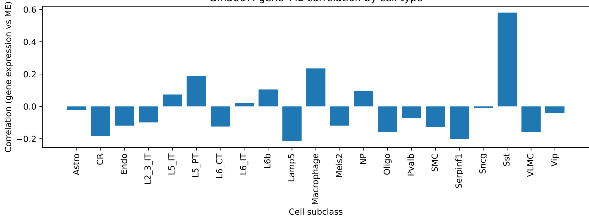
Gm3667: gene-ME correlation by cell type
