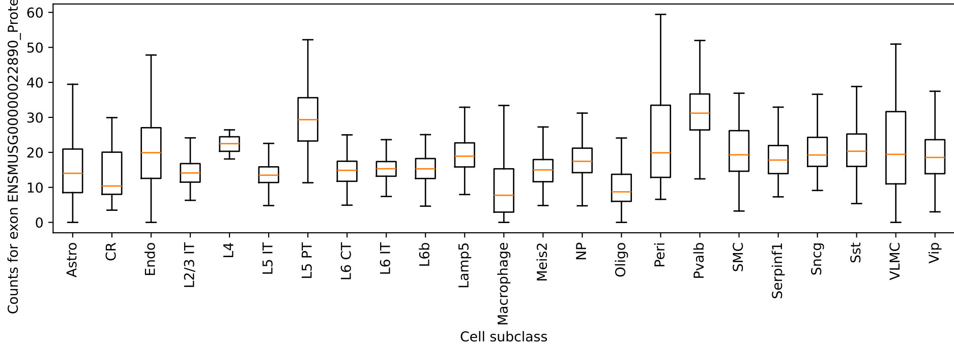
Atp5pf: exon ENSMUSG00000022890_ProteinCoding_2 counts by cell type
