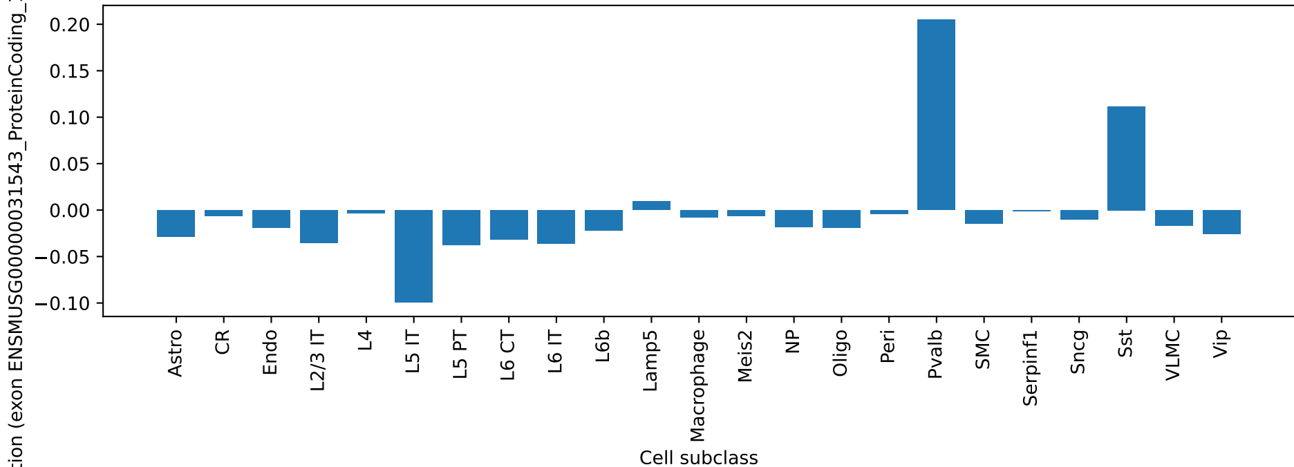
Ank1: exon ENSMUSG00000031543_ProteinCoding_1 correlation by cell type
