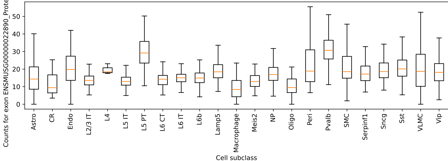
Atp5pf: exon ENSMUSG00000022890_ProteinCoding_1 counts by cell type
