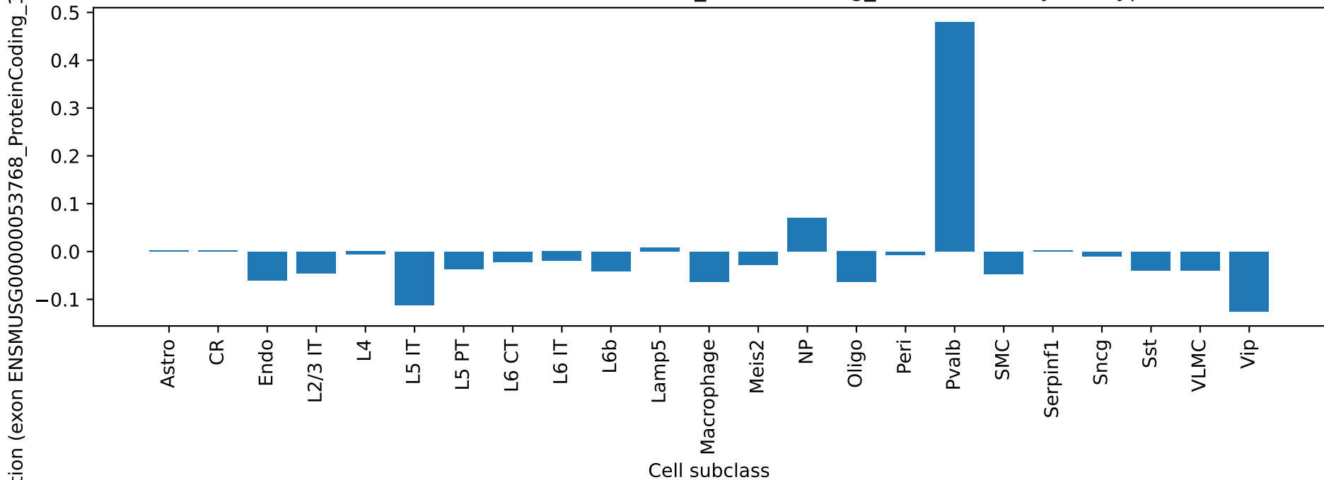
Chchd3: exon ENSMUSG00000053768_ProteinCoding_1 correlation by cell type
