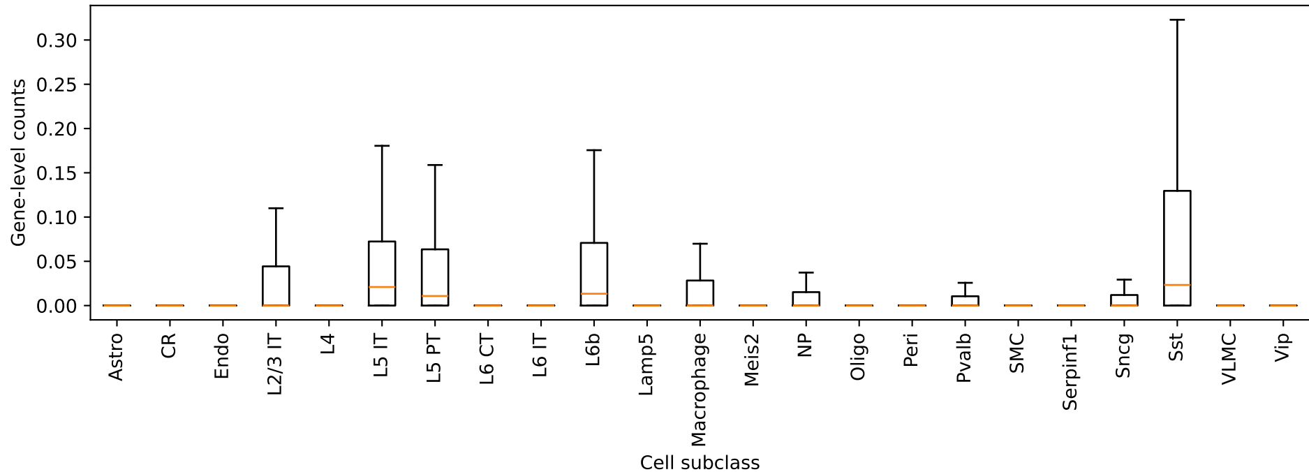
Gm3667: gene-level counts by cell type
