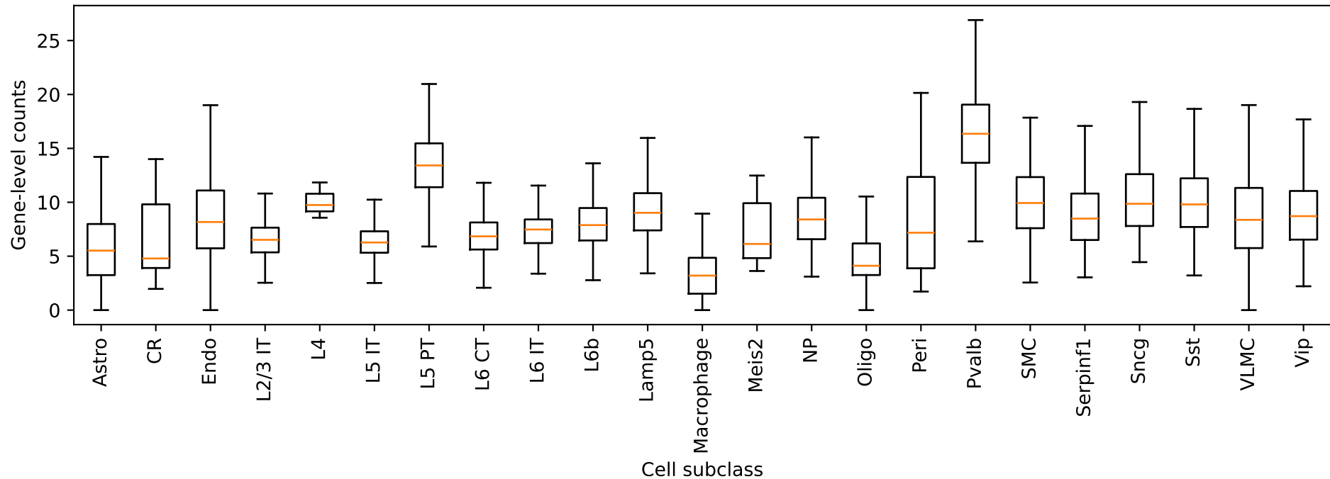
Atp5pf: gene-level counts by cell type
