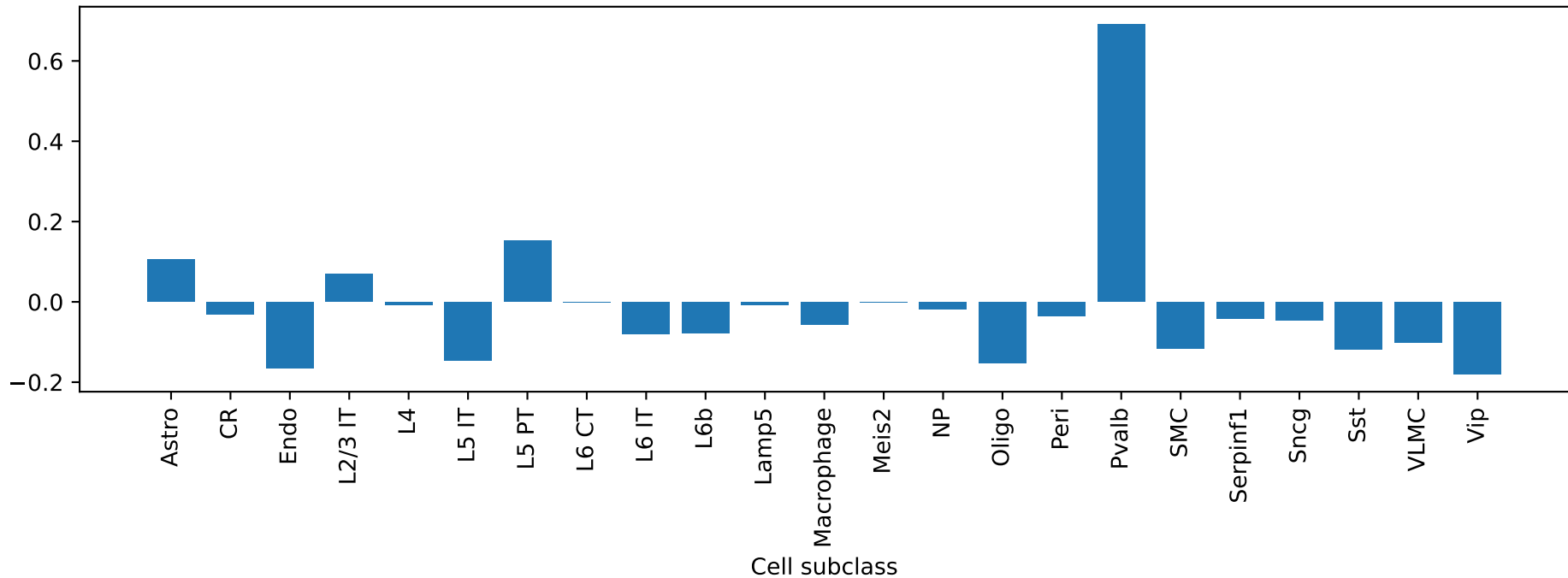
Ldhb: exon ENSMUSG00000030246_ProteinCoding_2 correlation by cell type
