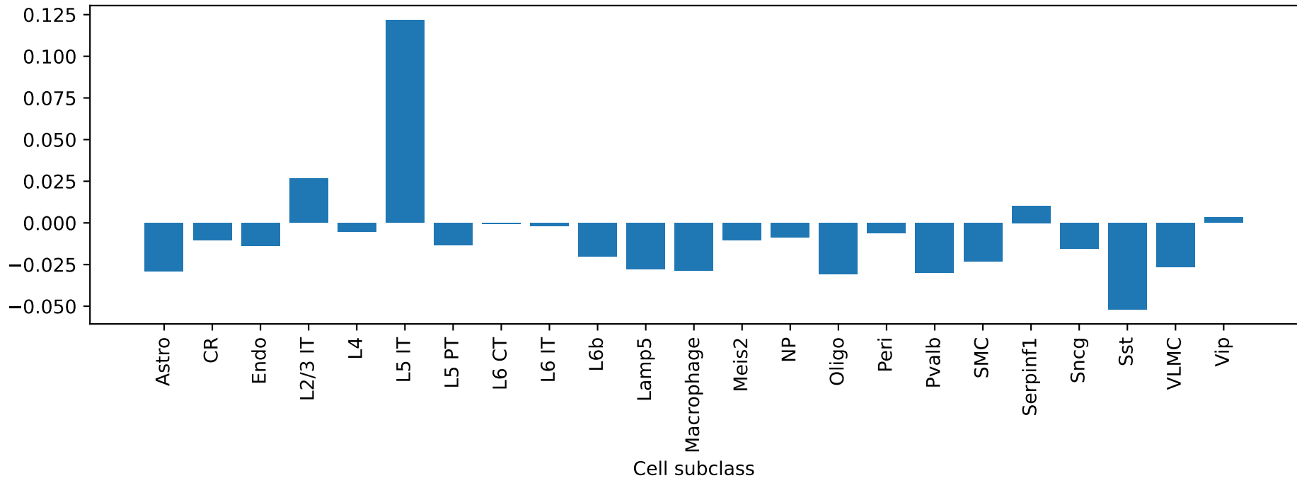
Tcte2: exon ENSMUSG00000038347_other_3 correlation by cell type
