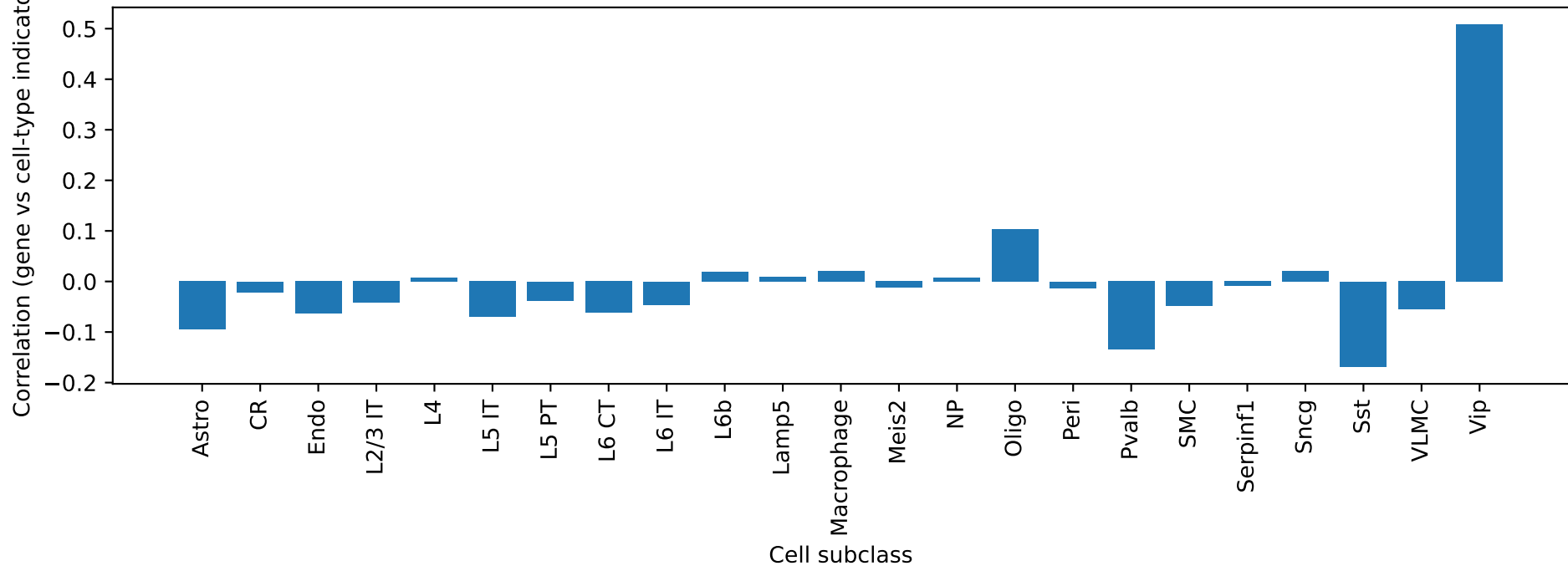
Csmd3: gene-level correlation by cell type
