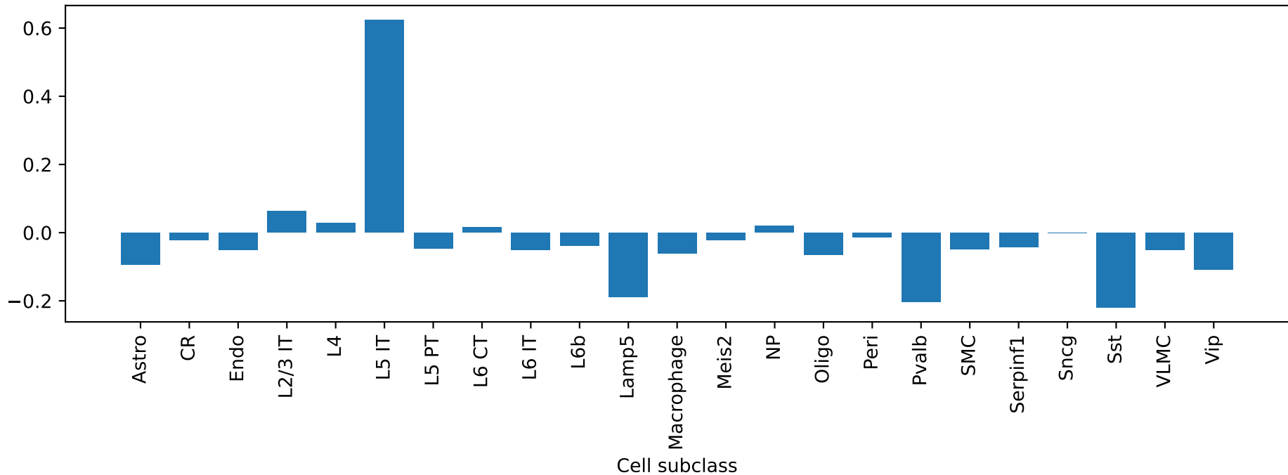
Tpd52l1: exon ENSMUSG00000000296_ProteinCoding_4 correlation by cell type
