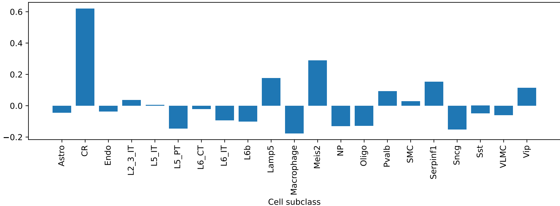
L3mbtl3: exon ENSMUSG00000039089_ProteinCoding_1 ME correlation by cell type
