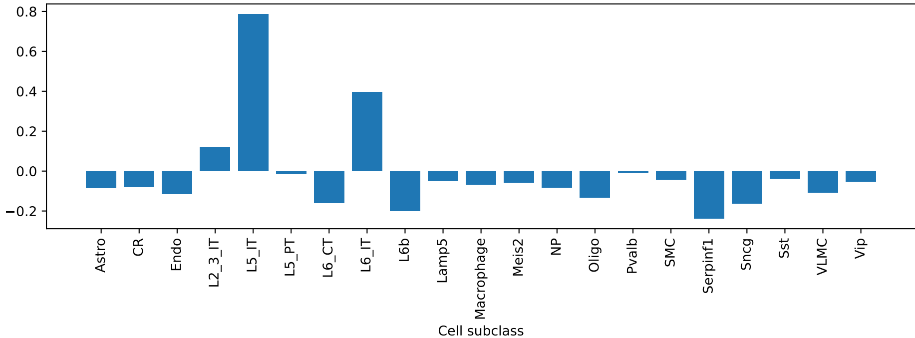
Dkl1: exon ENSMUSG00000030792_ProteinCoding_1 ME correlation by cell type
