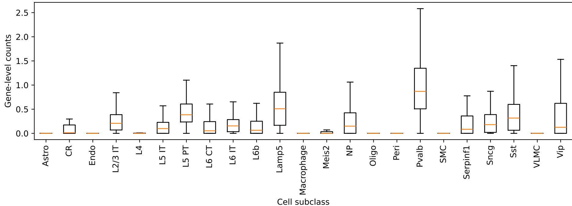
Clip4: gene-level counts by cell type
