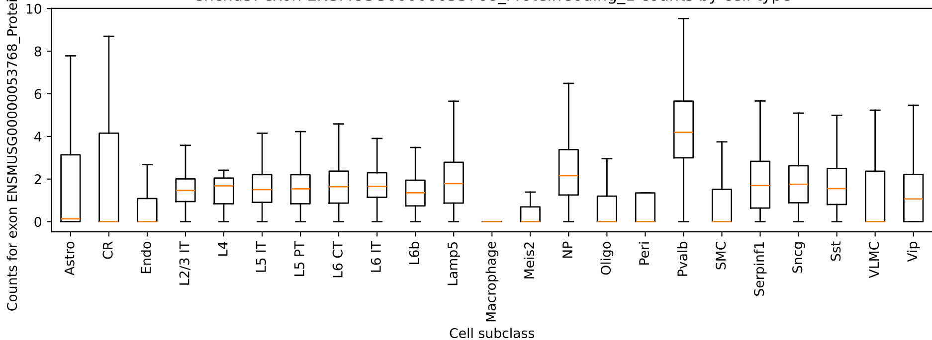
Chchd3: exon ENSMUSG00000053768_ProteinCoding_1 counts by cell type
