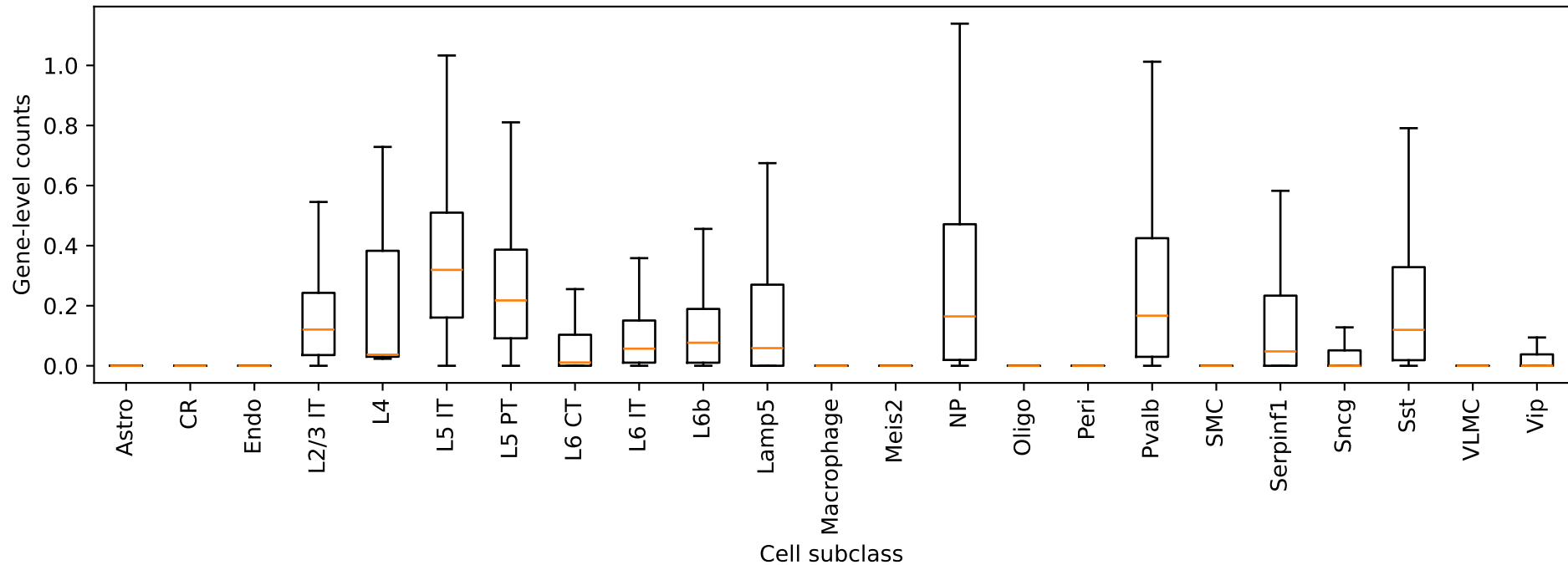
Efna5: gene-level counts by cell type
