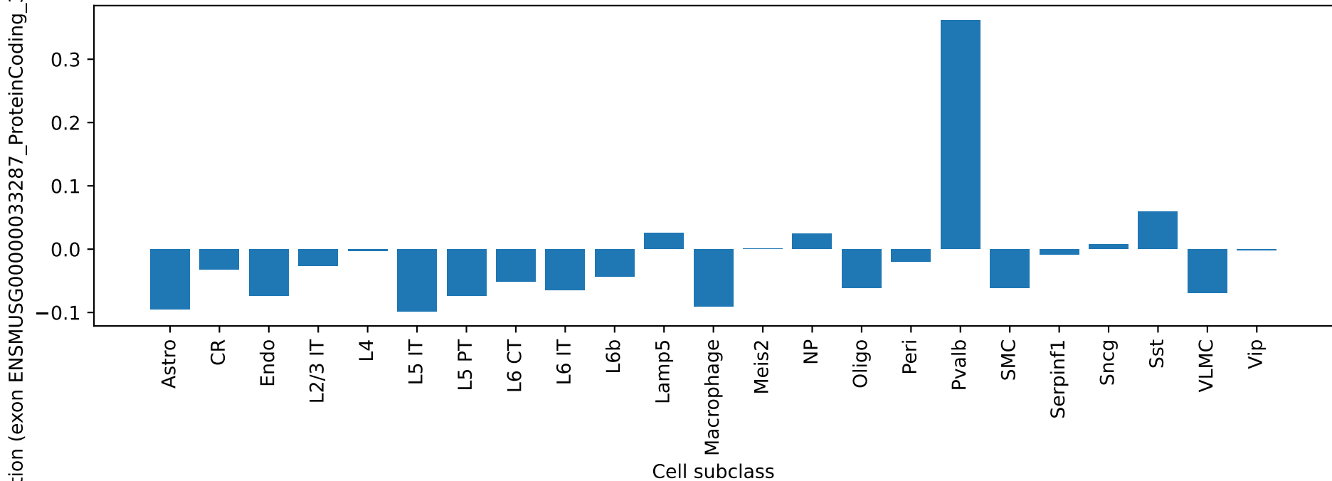
Kctd17: exon ENSMUSG00000033287_ProteinCoding_3 correlation by cell type
