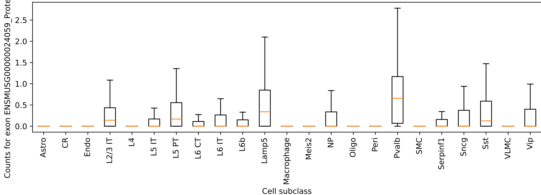
Clip4: exon ENSMUSG00000024059_ProteinCoding_4 counts by cell type
