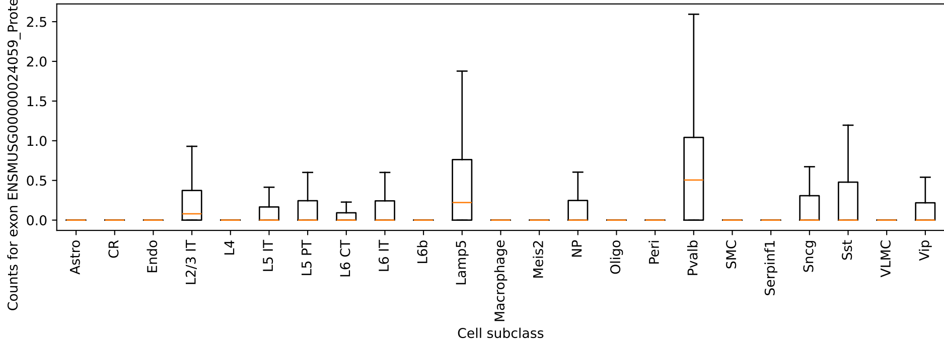
Clip4: exon ENSMUSG00000024059_ProteinCoding_2 counts by cell type
