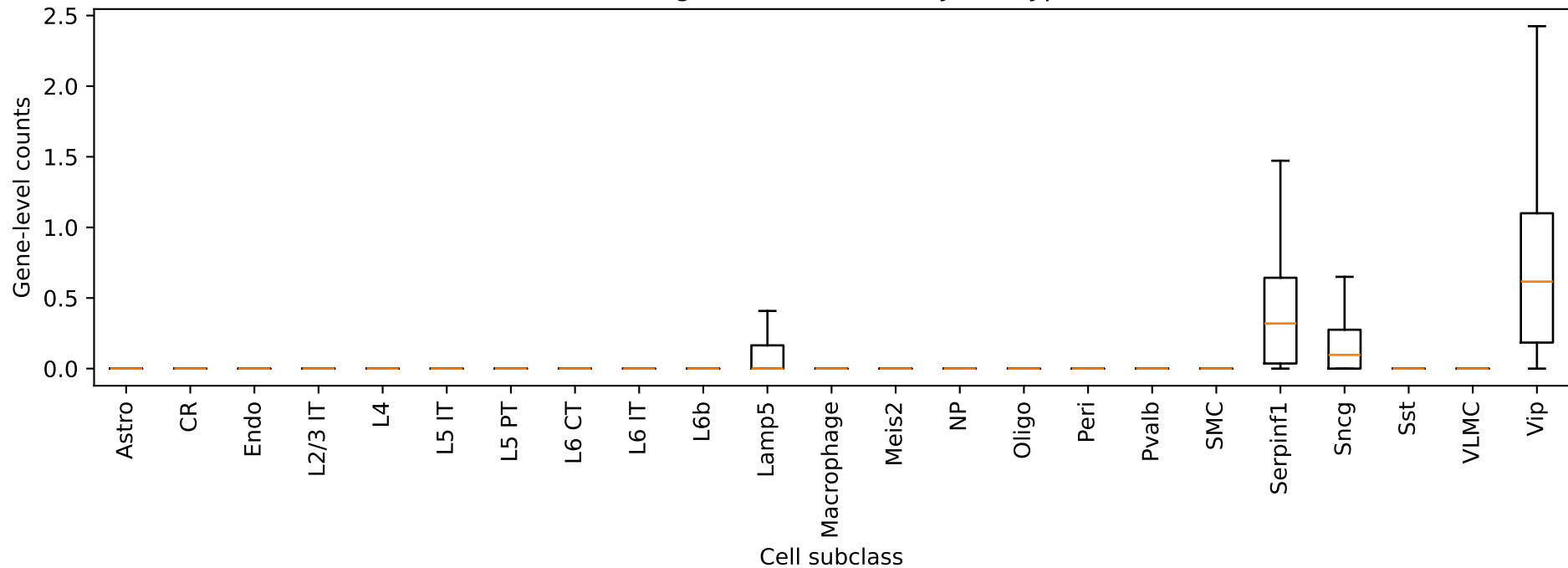
Asic4: gene-level counts by cell type
