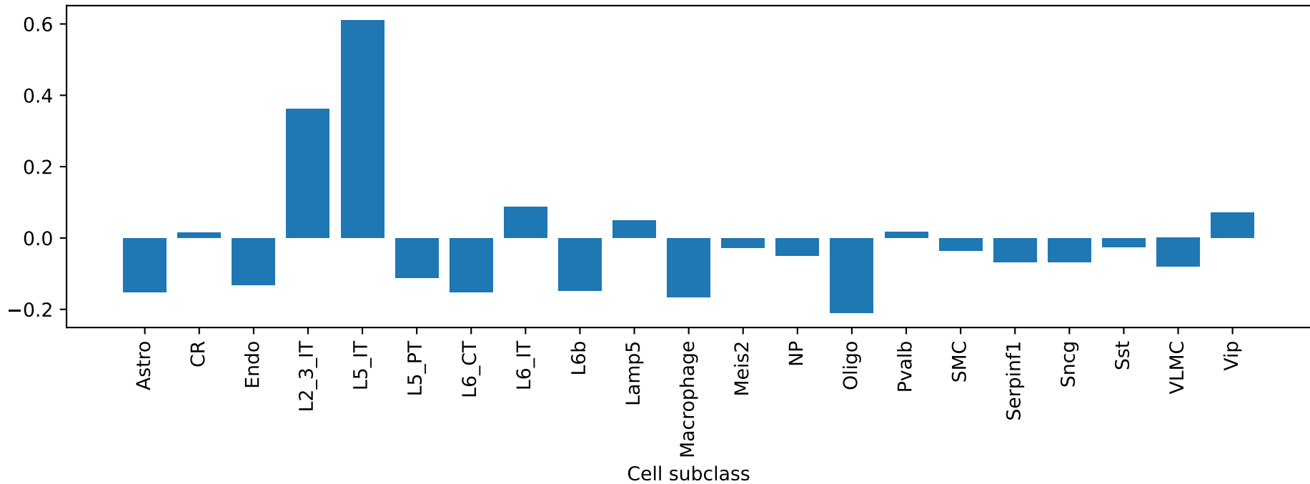
Or4d1: exon ENSMUSG00000060787_ProteinCoding_1 ME correlation by cell type
