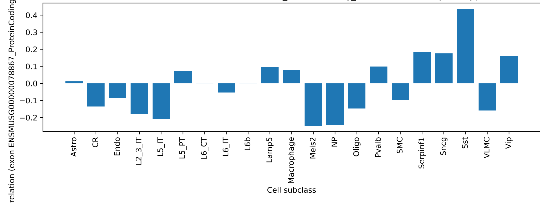
Gm14418: exon ENSMUSG00000078867_ProteinCoding_1 ME correlation by cell type
