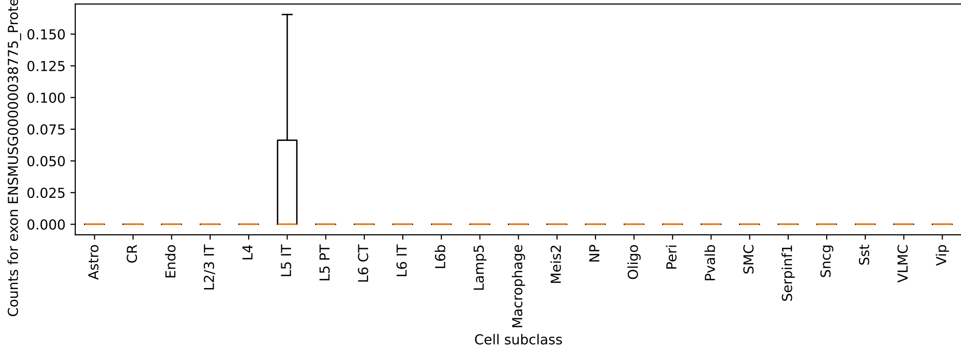
Vill: exon ENSMUSG00000038775_ProteinCoding_2 counts by cell type
