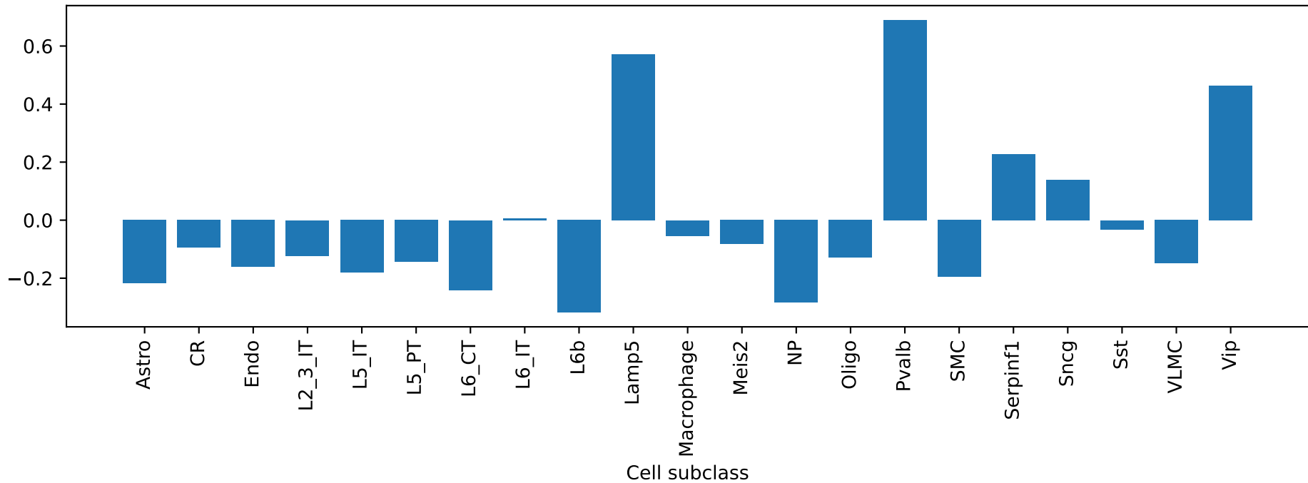
Erb4: exon ENSMUSG00000062209_ProteinCoding_1 ME correlation by cell type
