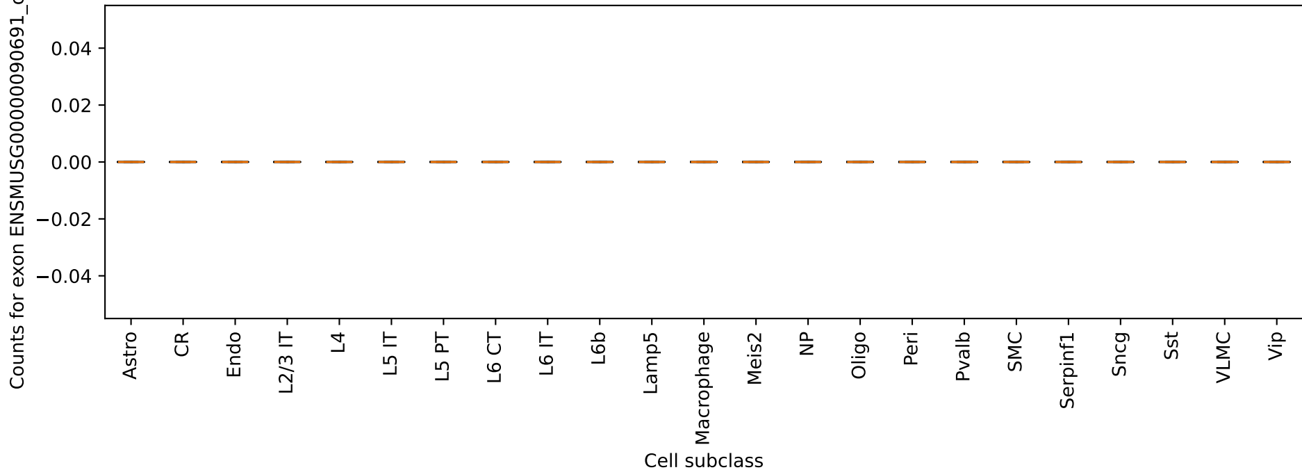
Gm3667: exon ENSMUSG00000090691_other_1 counts by cell type
