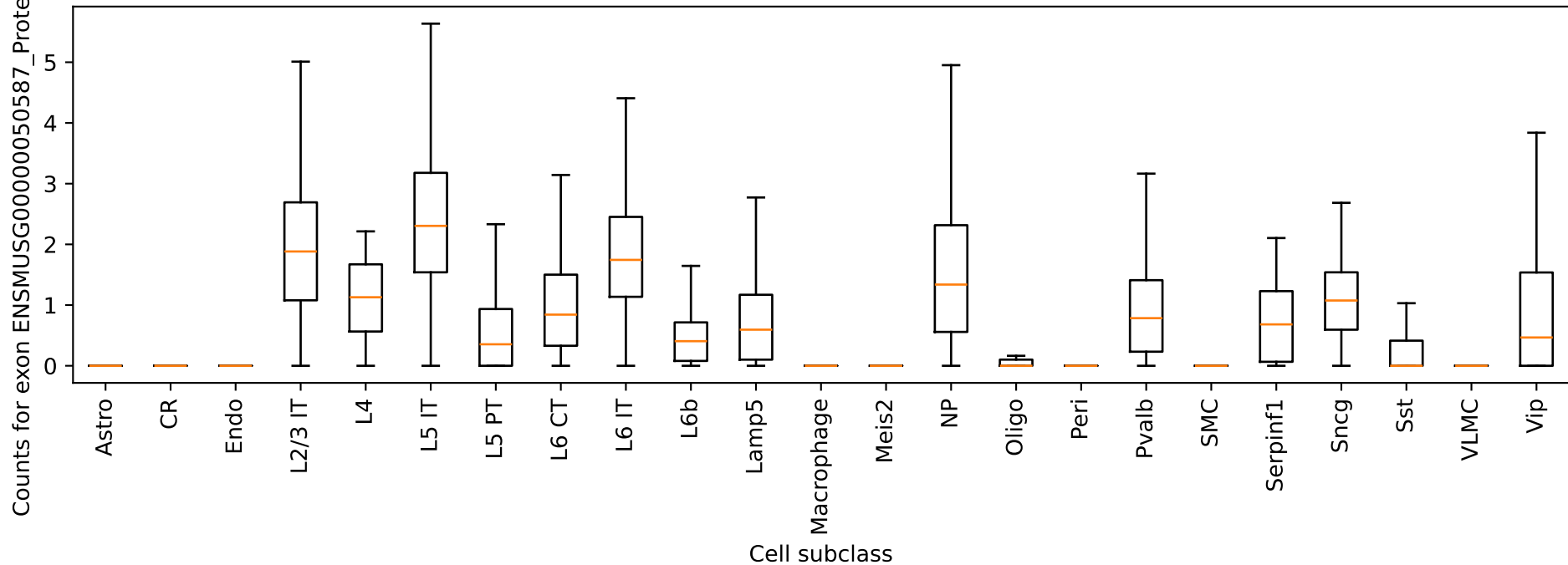
Lrrc4c: exon ENSMUSG00000050587_ProteinCoding_2 counts by cell type
