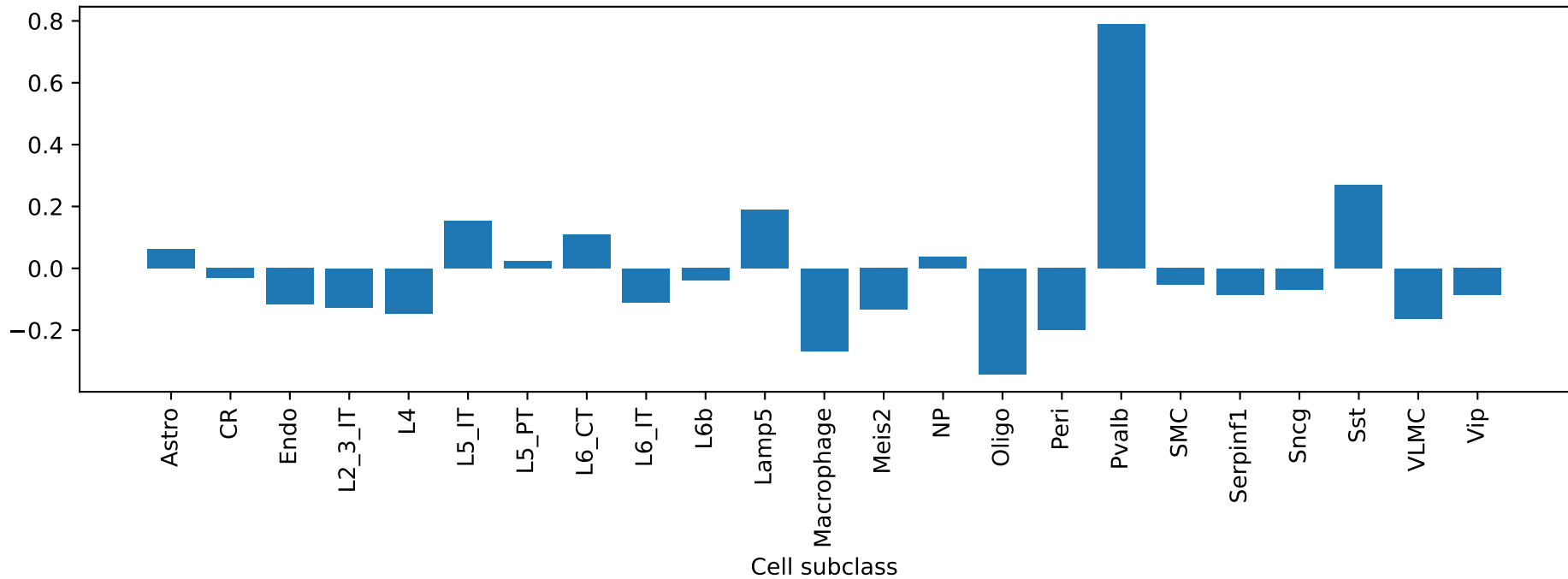
Chchd3: exon ENSMUSG00000053768_ProteinCoding_1 ME correlation by cell type
