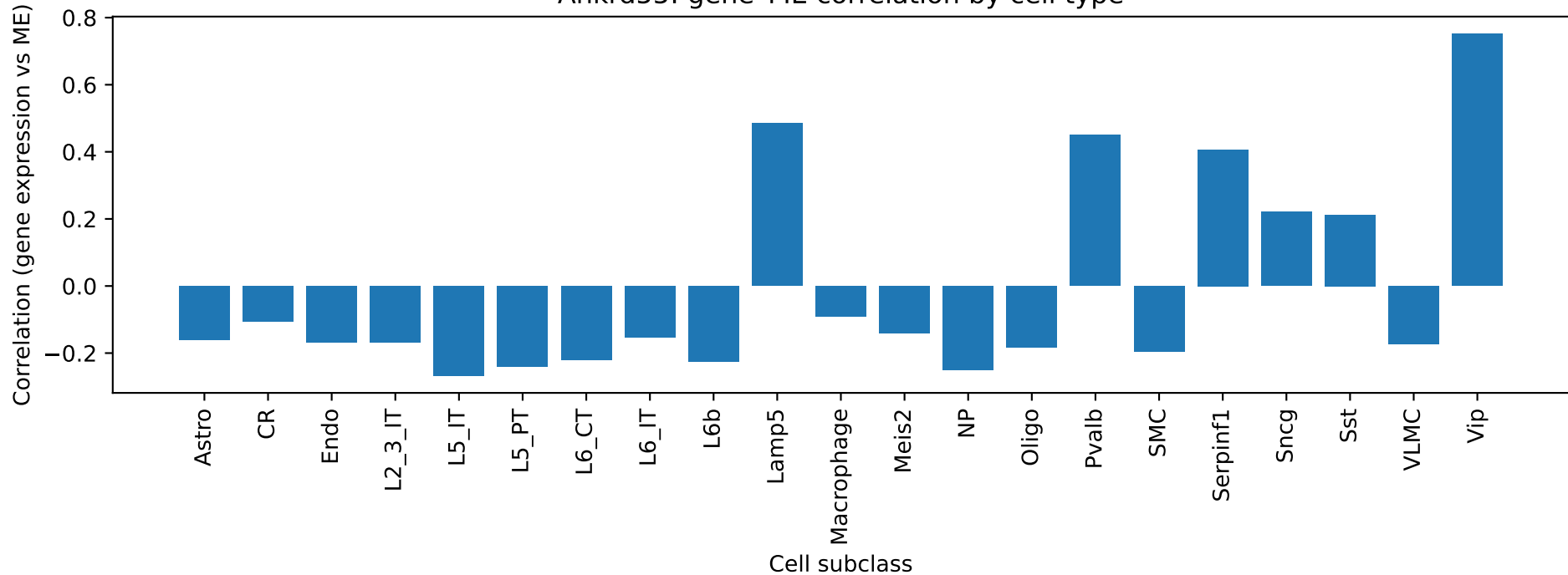
Ankrd55: gene-ME correlation by cell type
