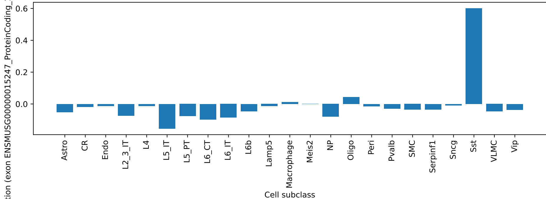
Nipsnap3b: exon ENSMUSG00000015247_ProteinCoding_1 correlation by cell type
