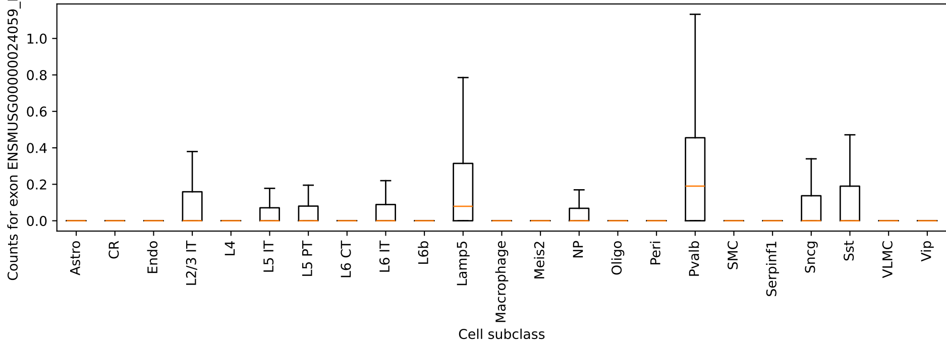
Clip4: exon ENSMUSG00000024059_NMD_1 counts by cell type
