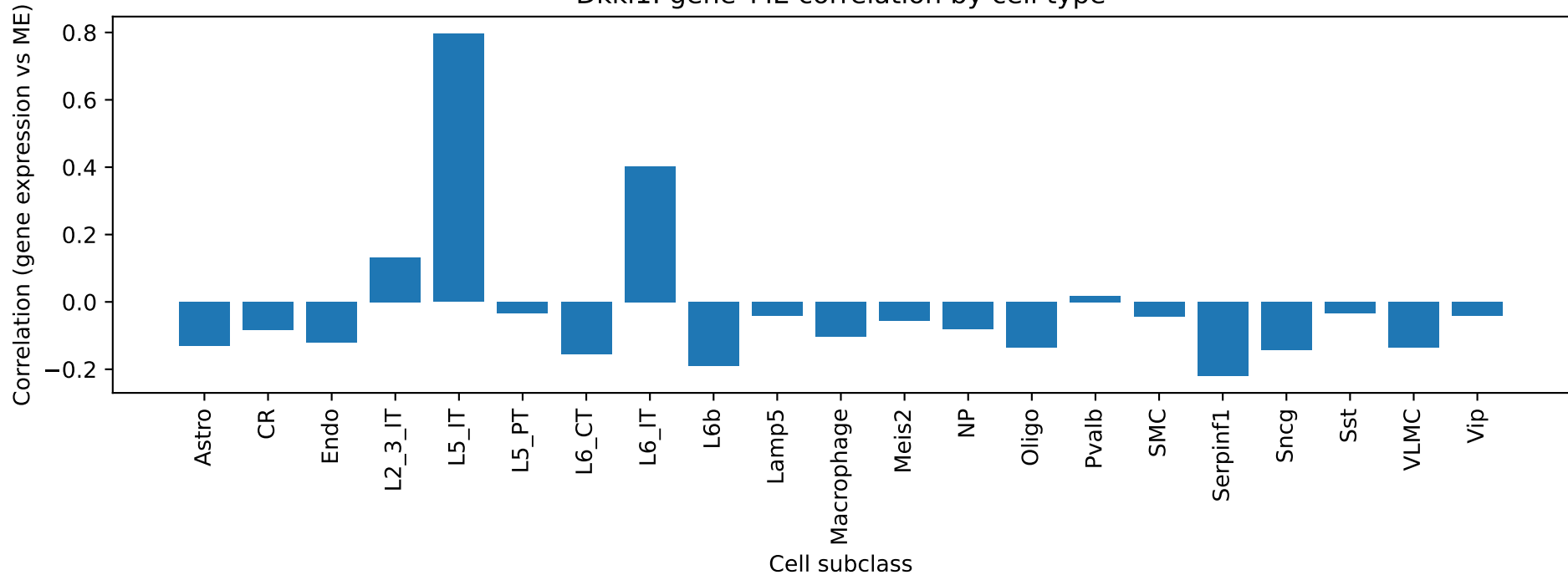
Dkk1: gene-ME correlation by cell type
