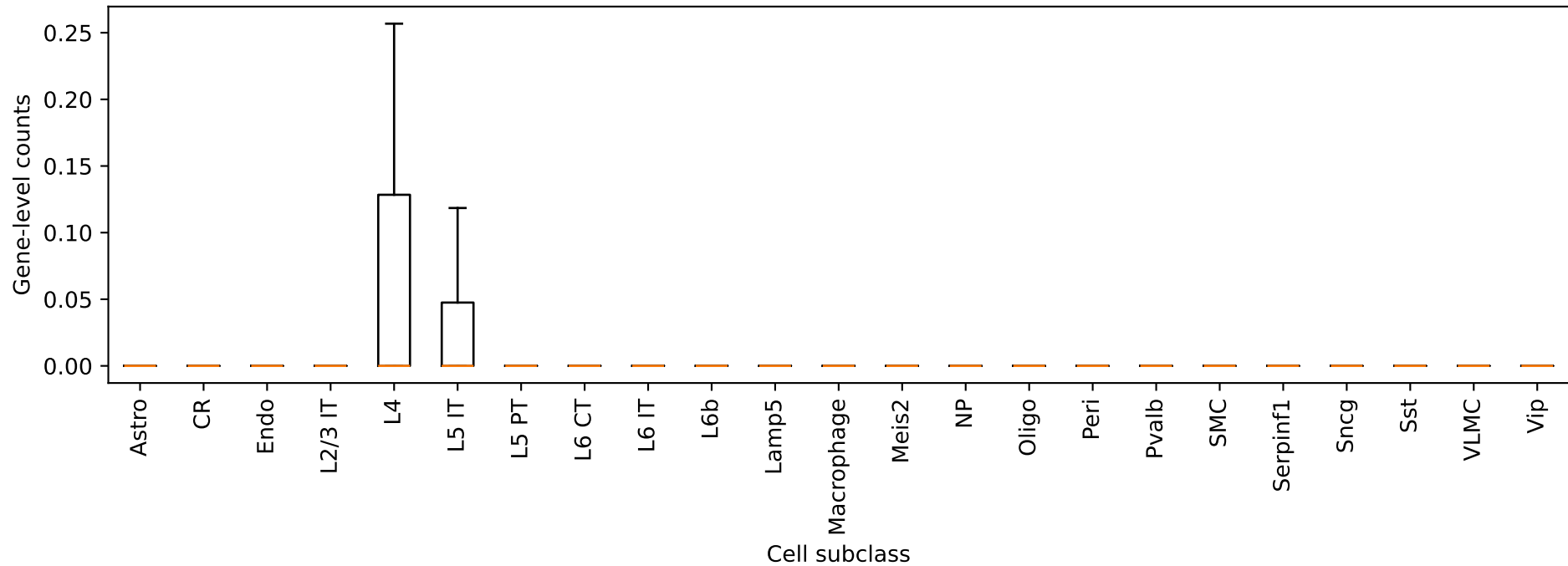
2810408I11Rik: gene-level counts by cell type
