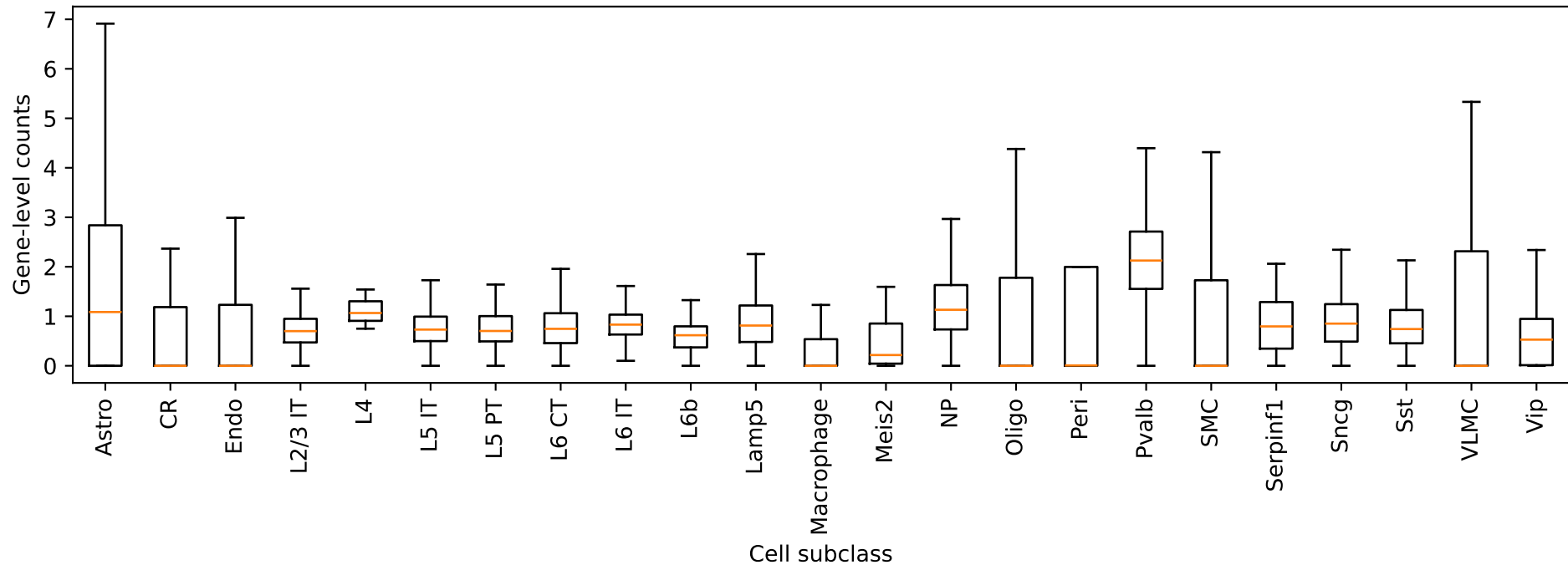
Chchd3: gene-level counts by cell type
