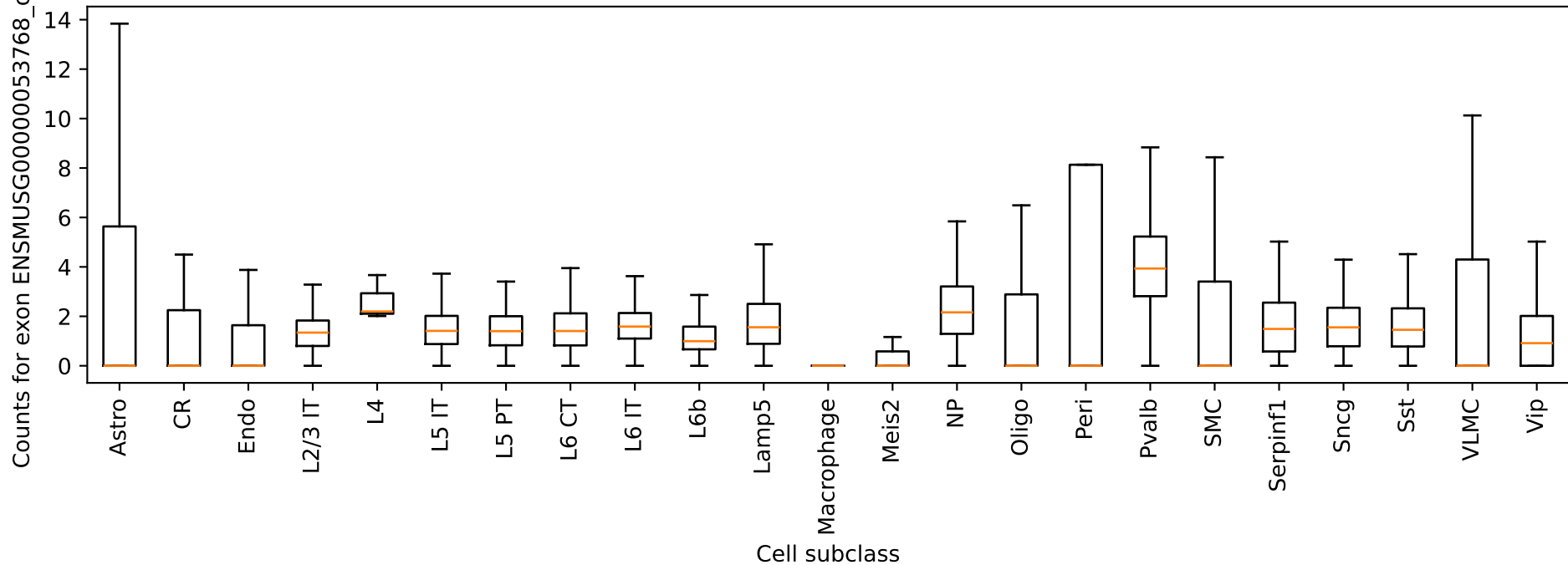
Chchd3: exon ENSMUSG00000053768_other_3 counts by cell type
