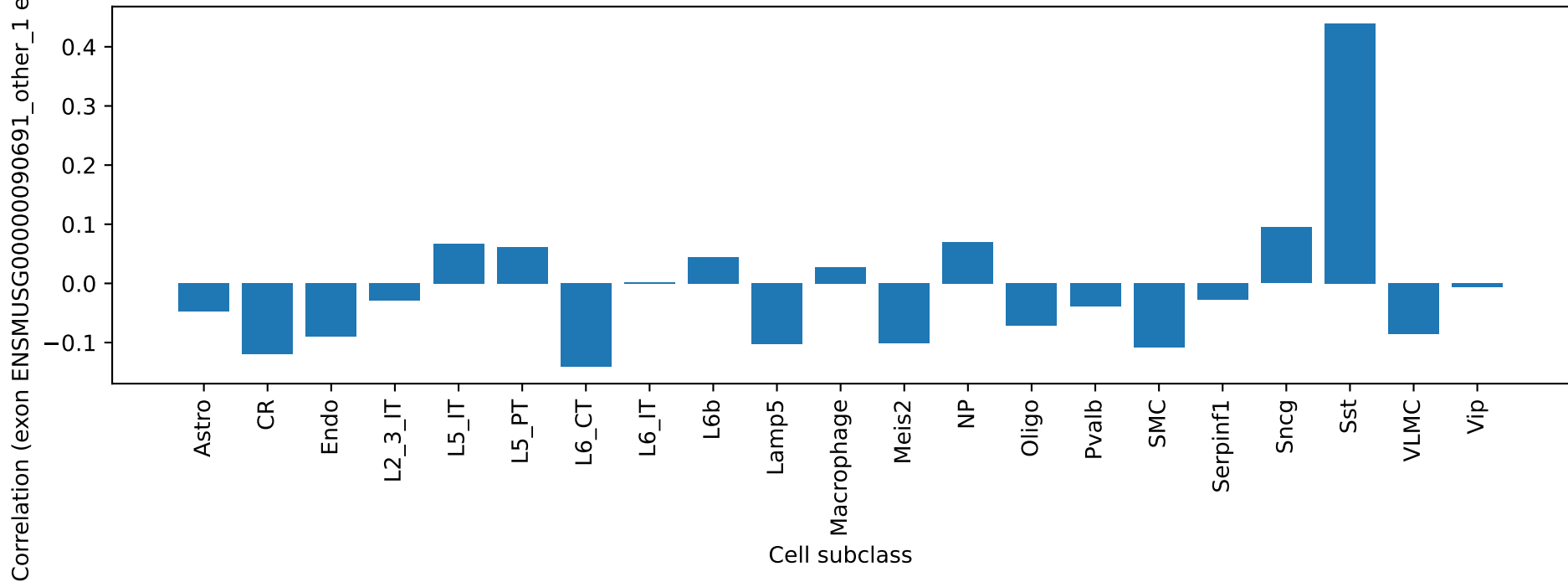
Gm3667: exon ENSMUSG00000090691_other_1 ME correlation by cell type
