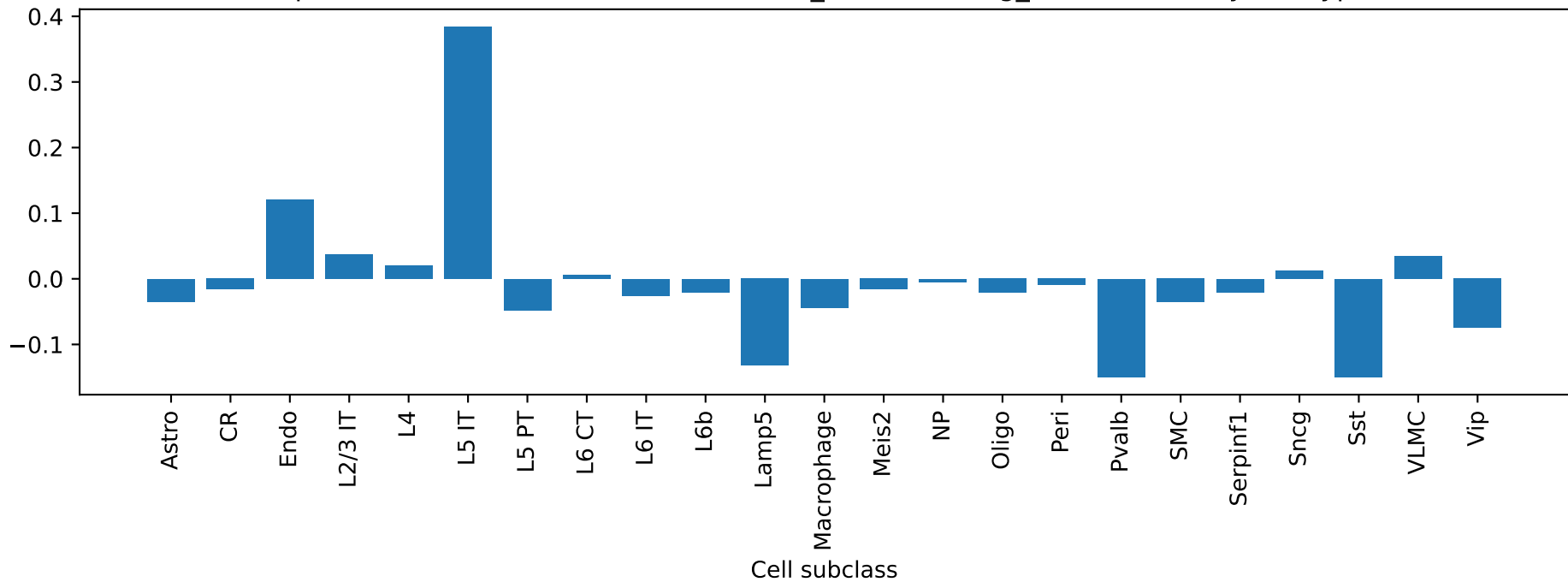
Tpd52l1: exon ENSMUSG00000000296_ProteinCoding_3 correlation by cell type
