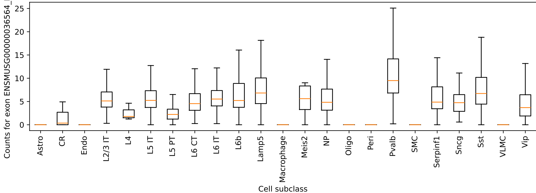
Ndr4: exon ENSMUSG00000036564_NMD_1 counts by cell type
