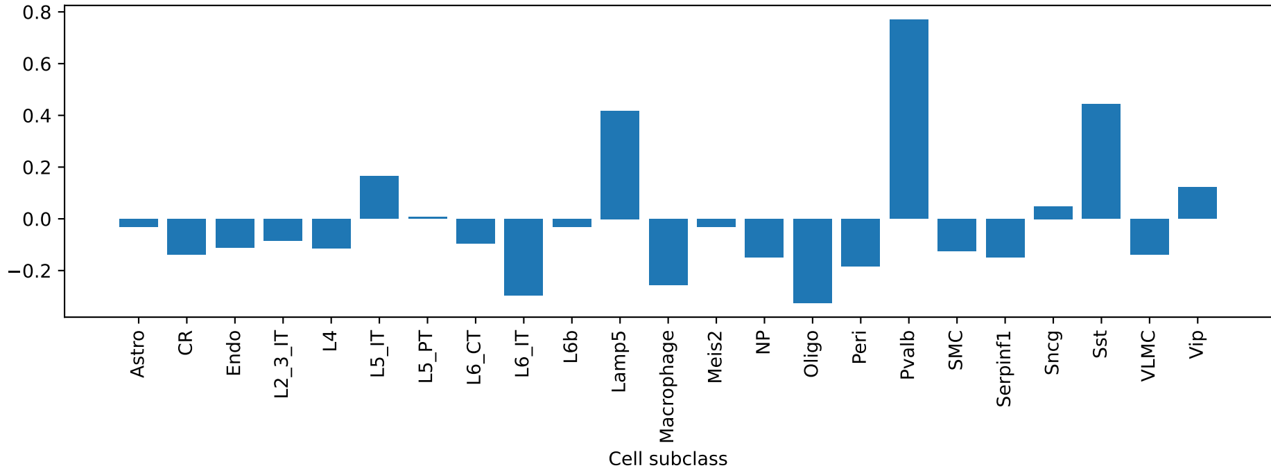
Clip4: exon ENSMUSG00000024059_ProteinCoding_3 ME correlation by cell type
