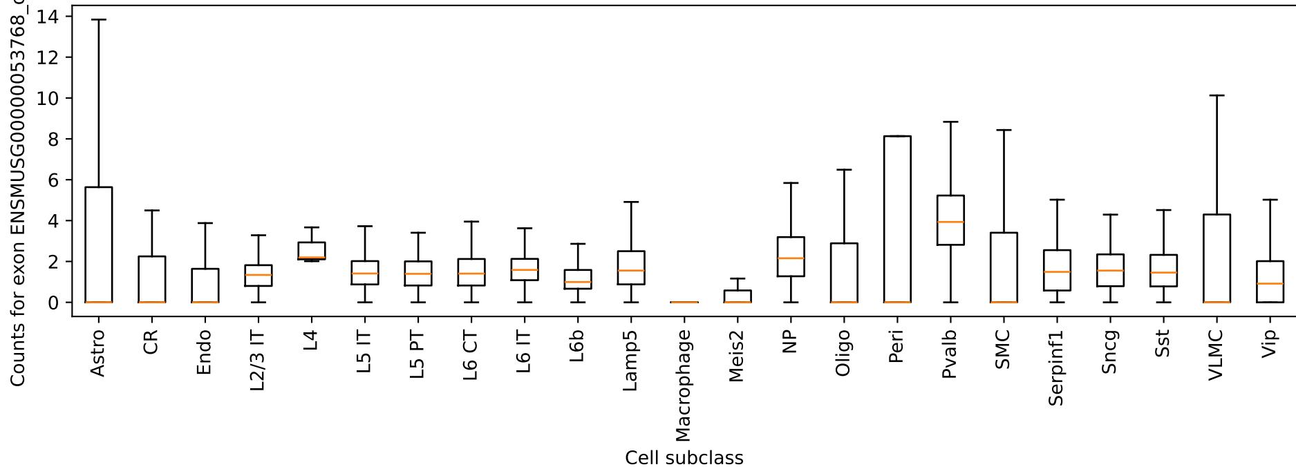
Chchd3: exon ENSMUSG00000053768_other_1 counts by cell type
