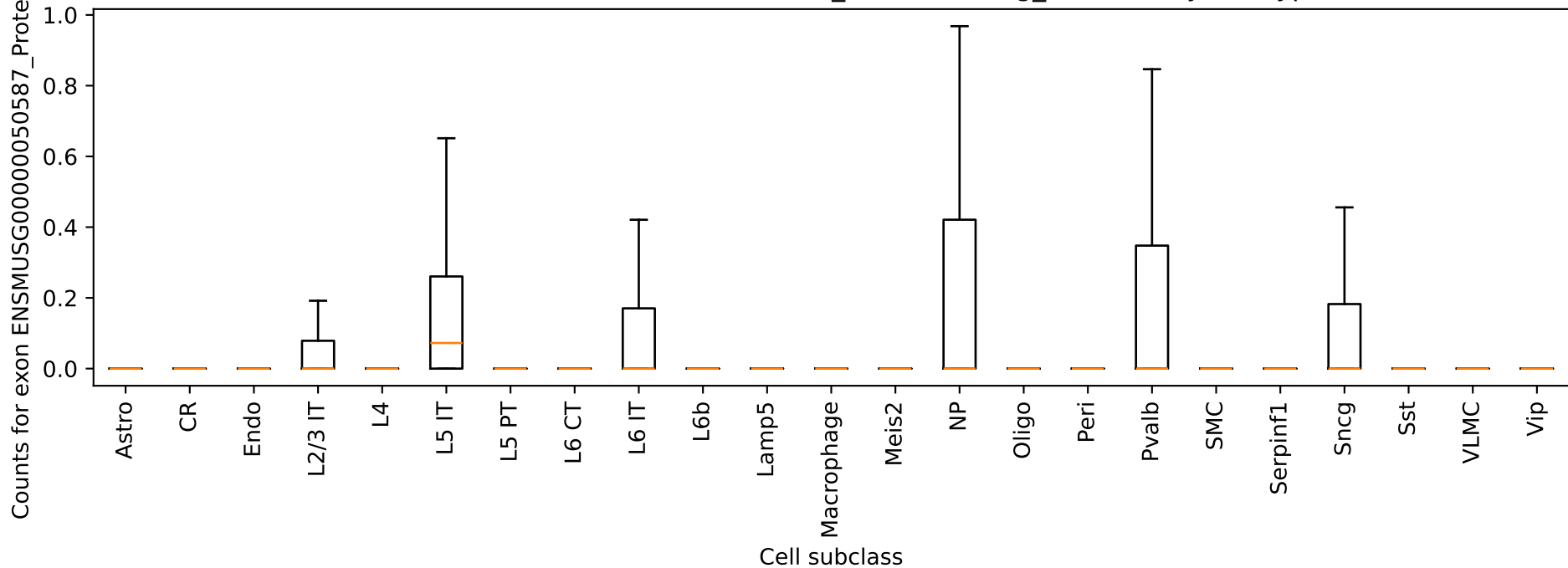
Lrrc4c: exon ENSMUSG00000050587_ProteinCoding_1 counts by cell type
