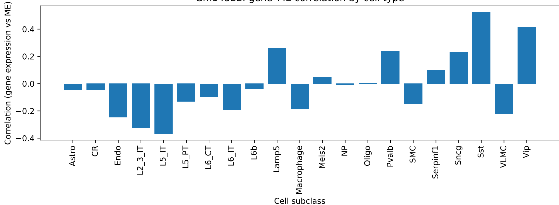
Gm14322: gene-ME correlation by cell type
