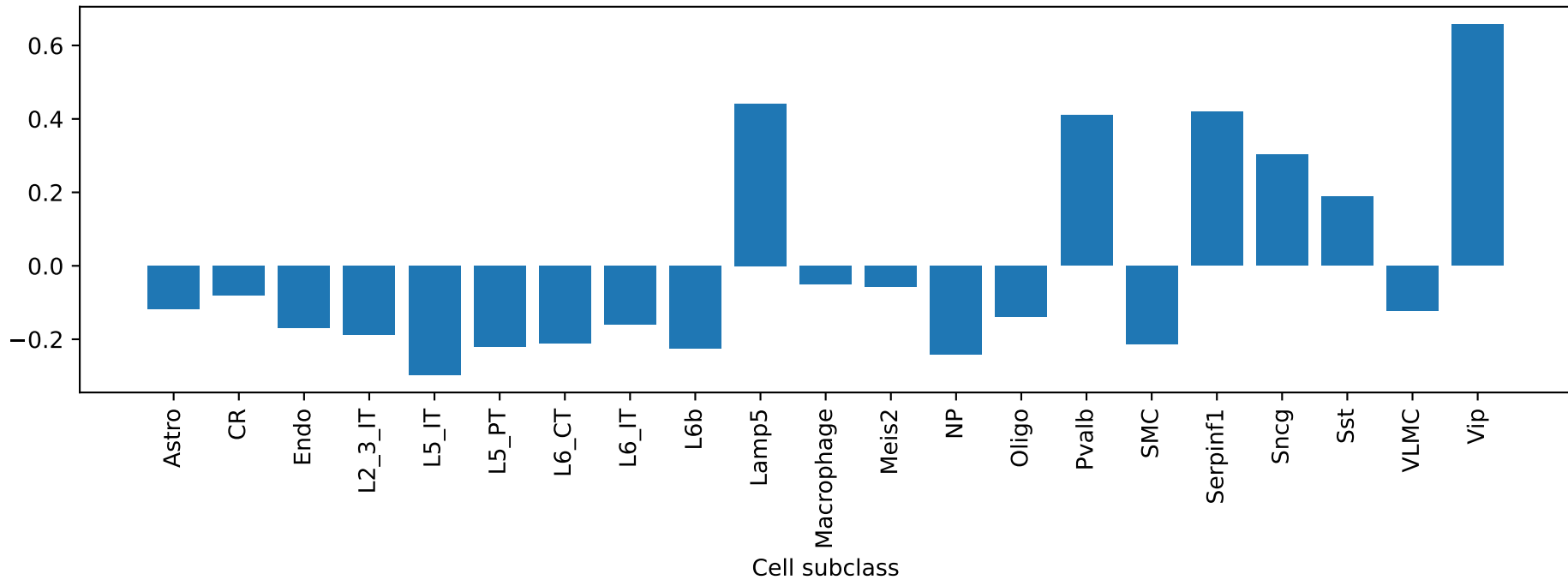
Ankrd55: exon ENSMUSG00000049985_ProteinCoding_1 ME correlation by cell type
