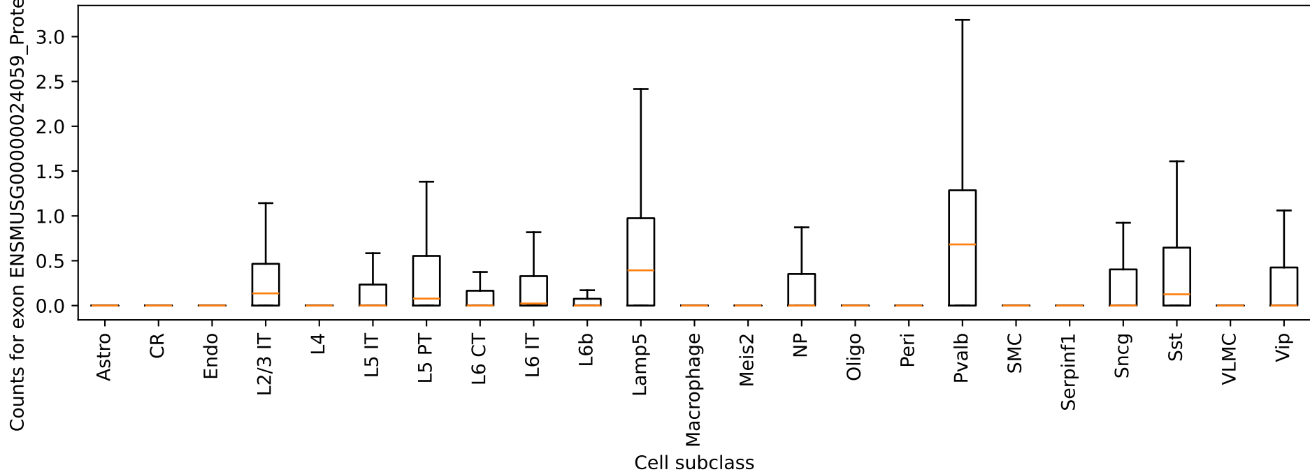
Clip4: exon ENSMUSG00000024059_ProteinCoding_3 counts by cell type
