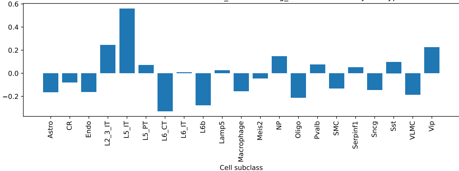
Cdh8: exon ENSMUSG00000036510_ProteinCoding_1 ME correlation by cell type
