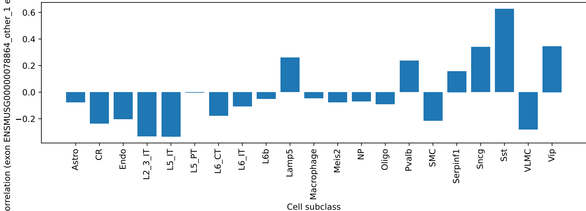
Gm14322: exon ENSMUSG00000078864_other_1 ME correlation by cell type
