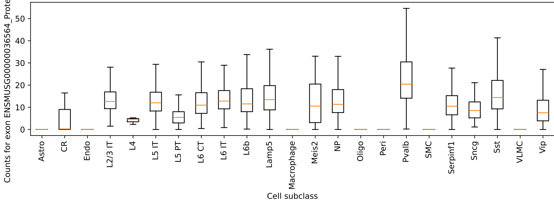
Ndr4: exon ENSMUSG00000036564_ProteinCoding_2 counts by cell type
