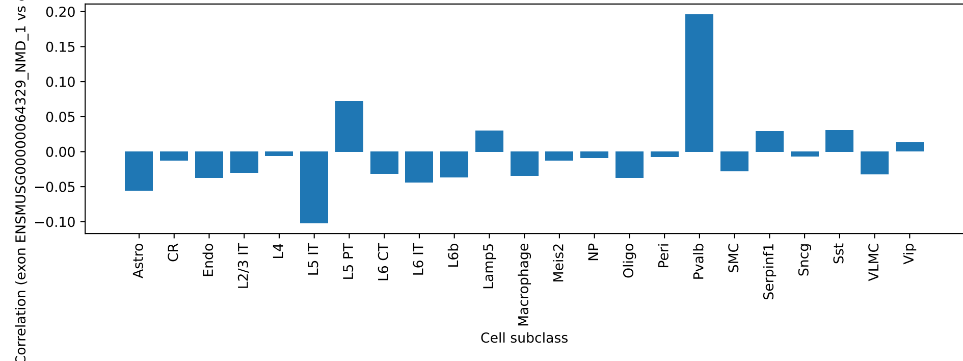
Scn1a: exon ENSMUSG00000064329_NMD_1 correlation by cell type
