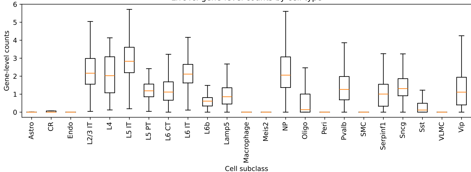
Lrrc4c: gene-level counts by cell type
