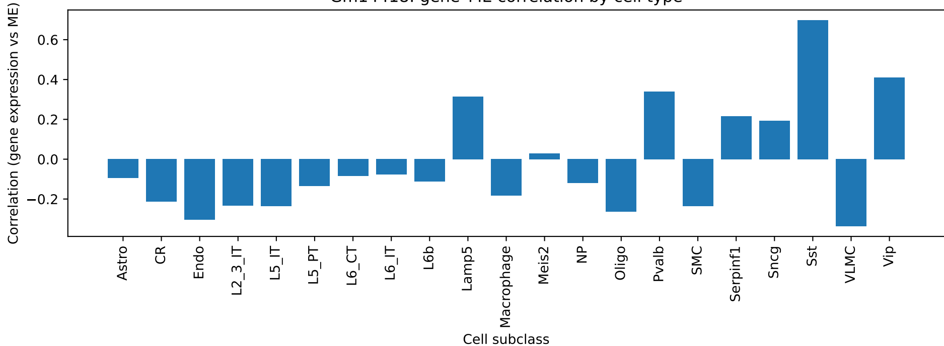
Gm14418: gene-ME correlation by cell type
