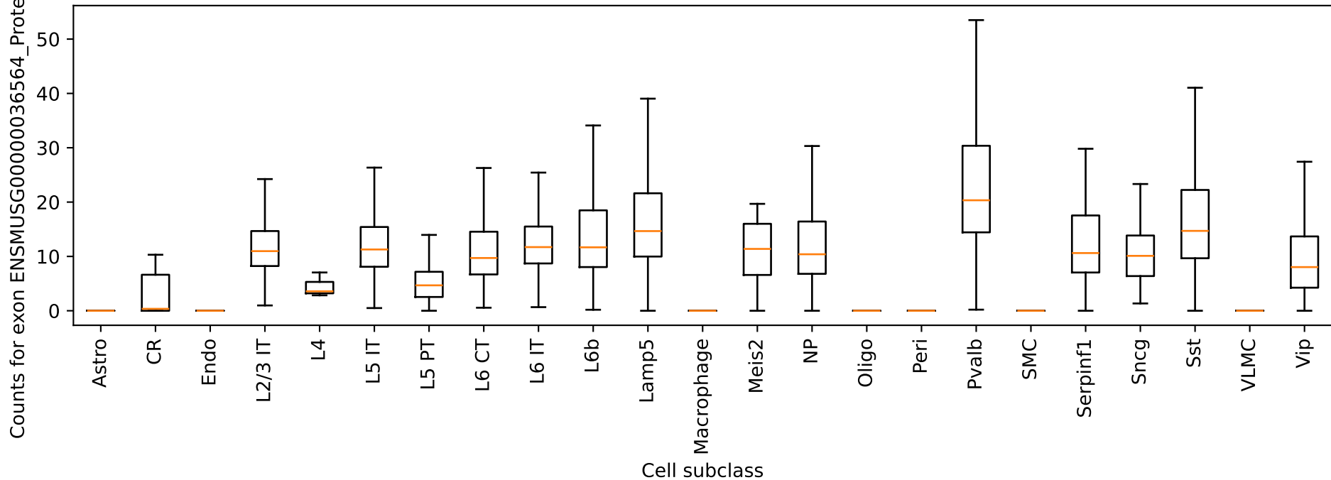
Ndr4: exon ENSMUSG00000036564_ProteinCoding_1 counts by cell type
