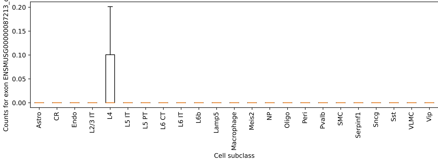
2810408I11Rik: exon ENSMUSG00000087213_other_1 counts by cell type
