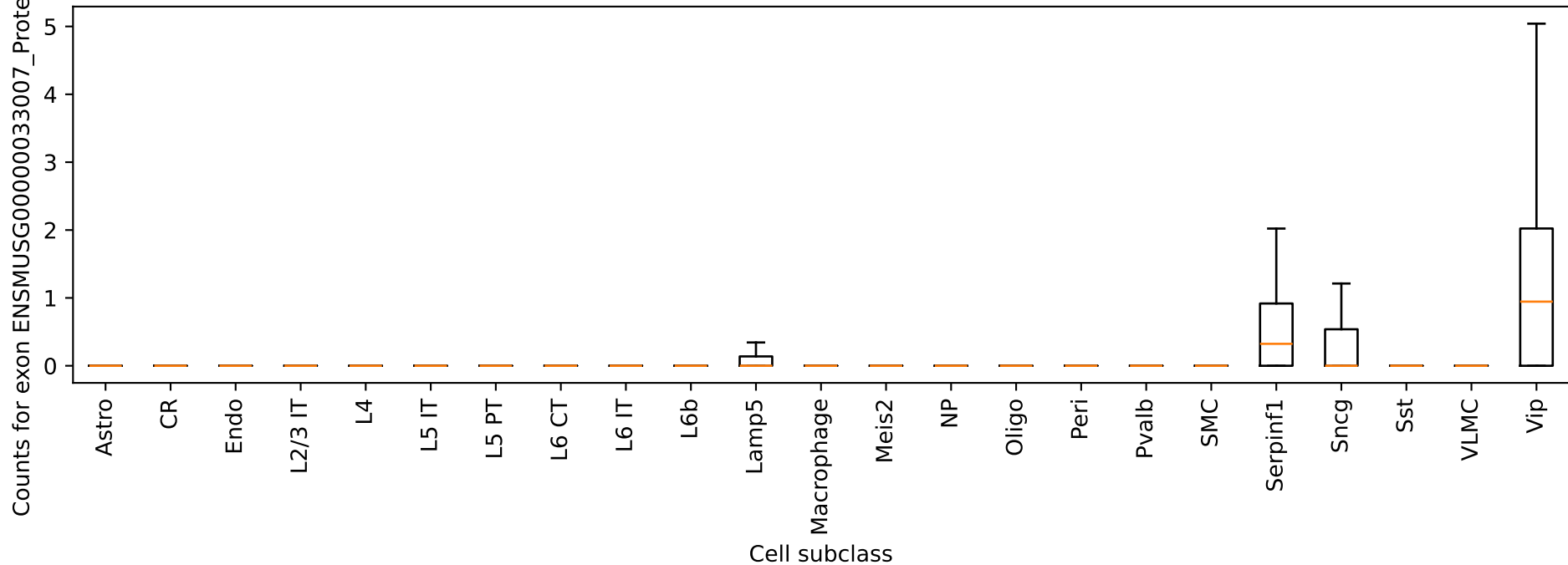
Asic4: exon ENSMUSG00000033007_ProteinCoding_1 counts by cell type
