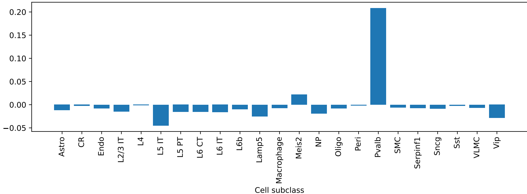
Th: exon ENSMUSG00000000214_ProteinCoding_1 correlation by cell type
