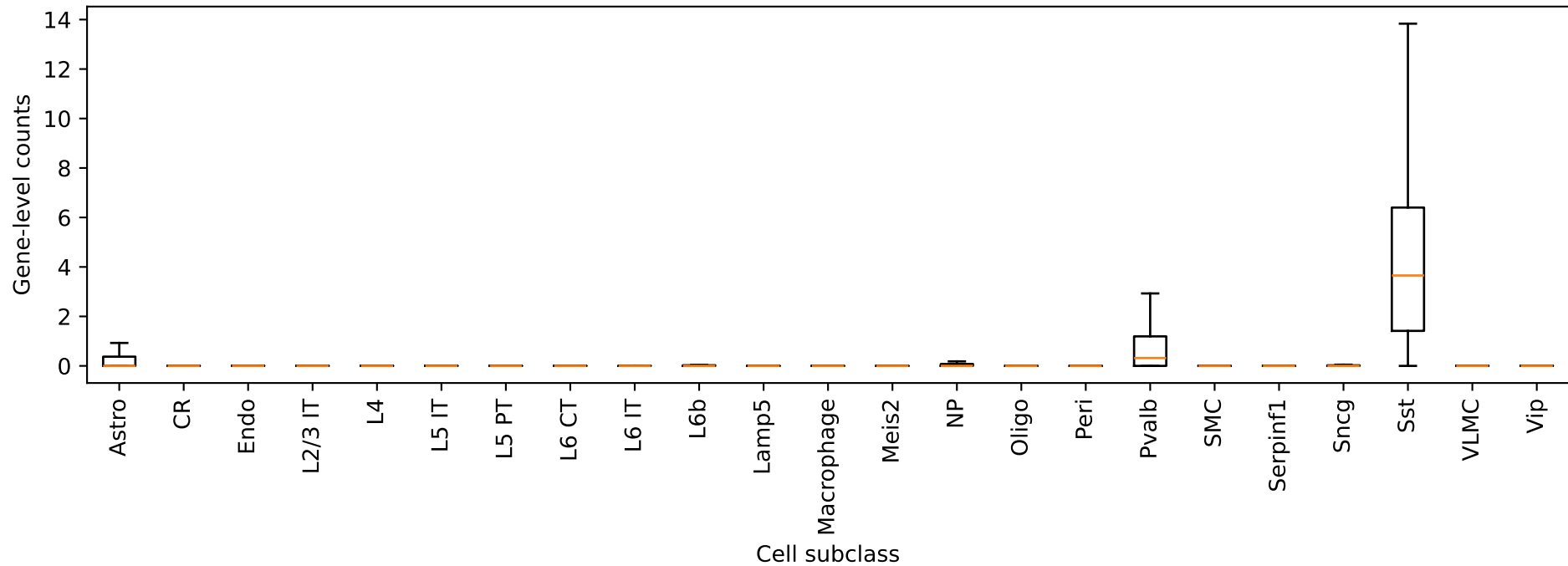
Lypd6: gene-level counts by cell type
