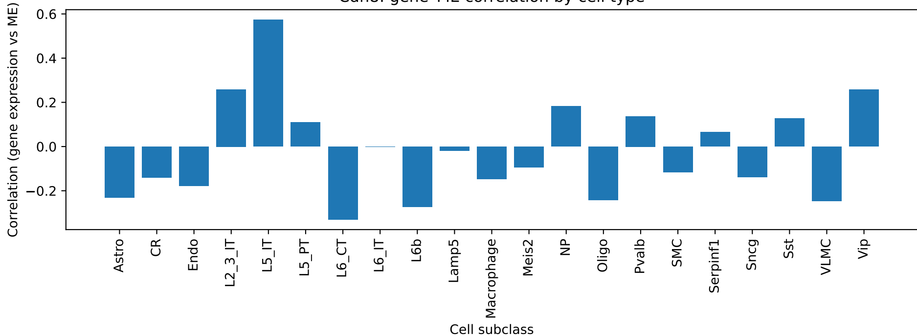
Cdh8: gene-ME correlation by cell type
