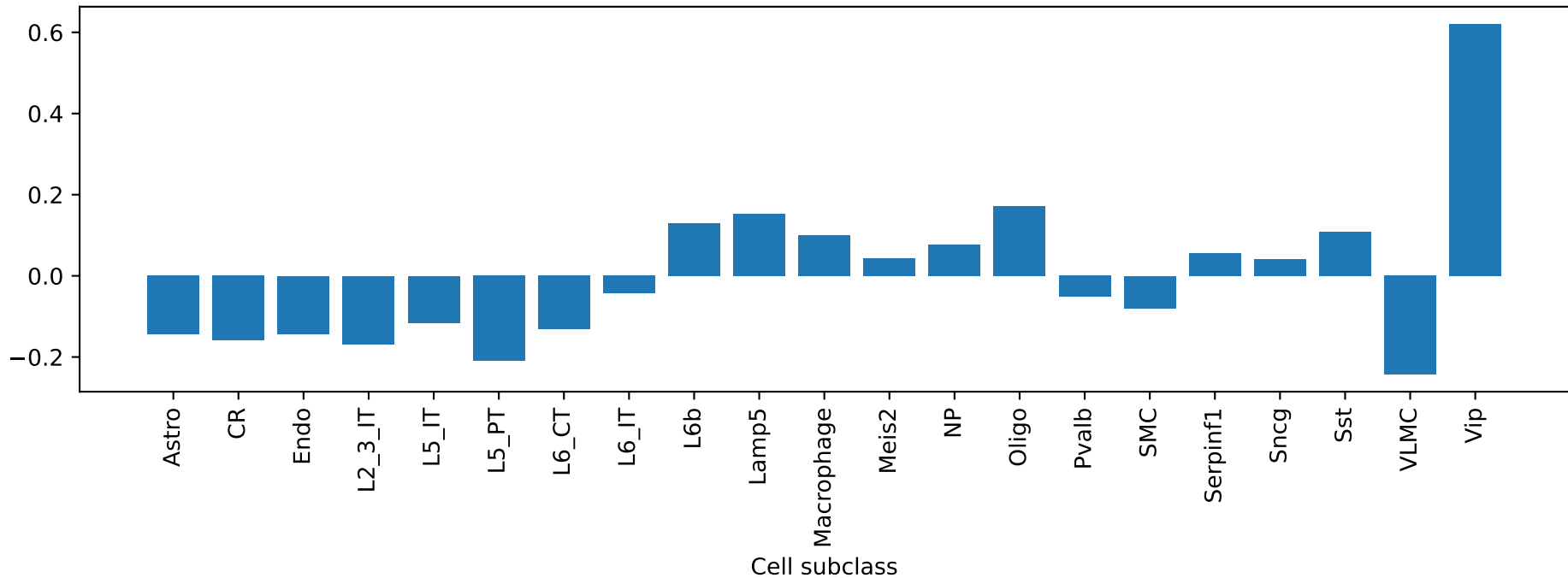
Csmd3: exon ENSMUSG00000022311_ProteinCoding_2 ME correlation by cell type
