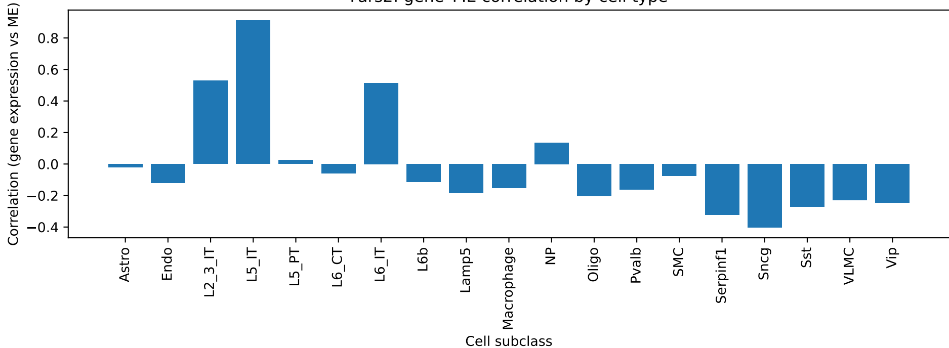
Fars2: gene-ME correlation by cell type
