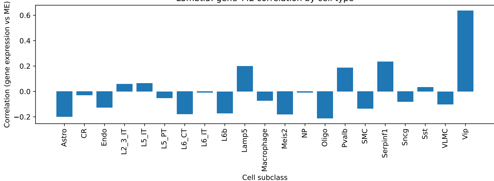
L3mbtl3: gene-ME correlation by cell type
