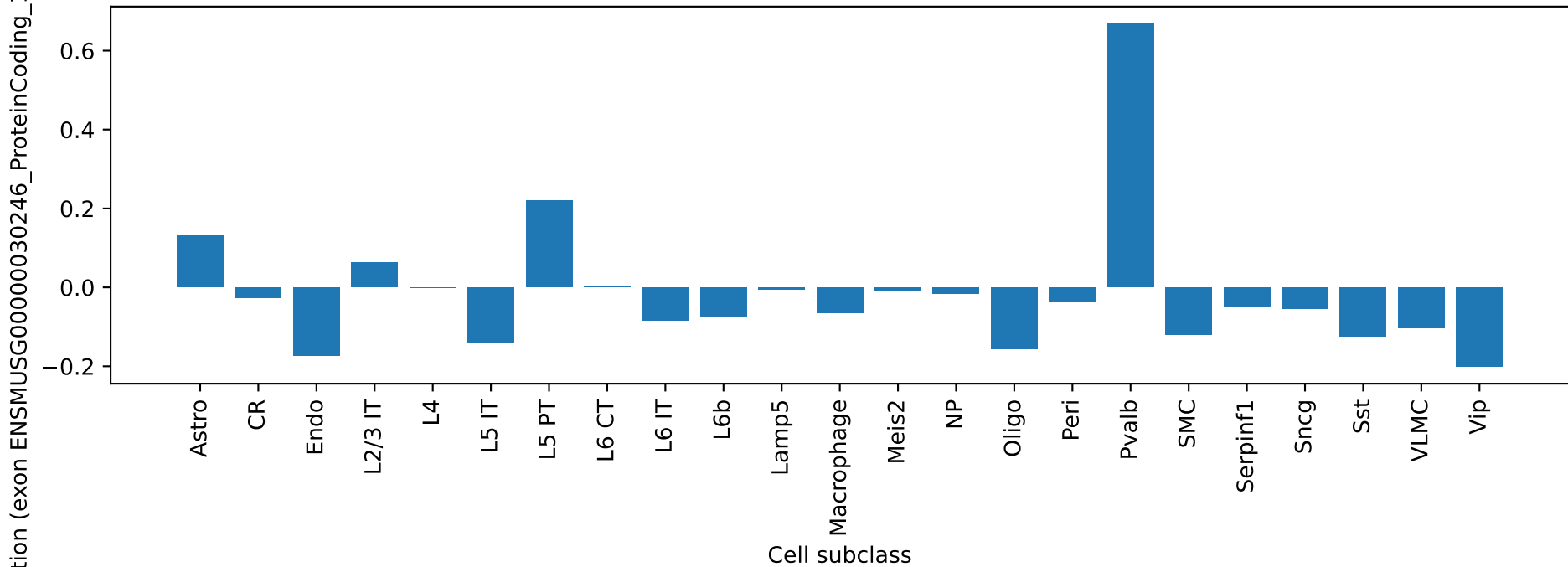
Ldhb: exon ENSMUSG00000030246_ProteinCoding_1 correlation by cell type
