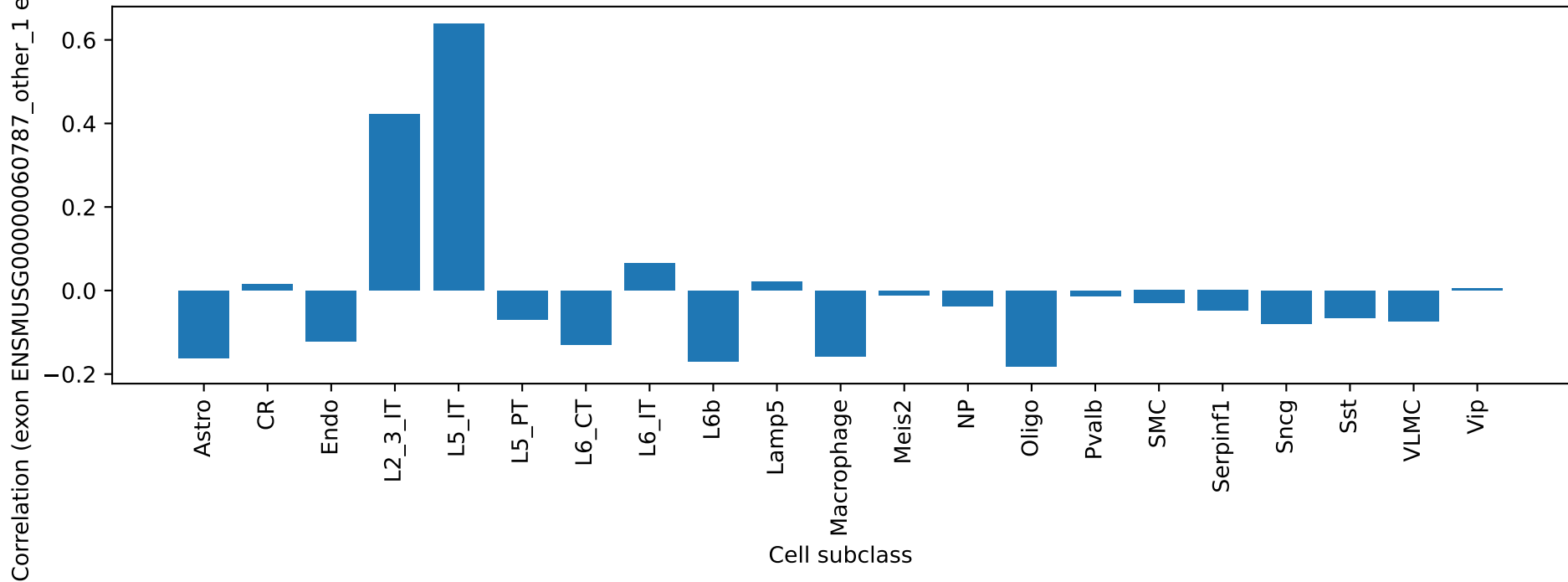
Or4d1: exon ENSMUSG00000060787_other_1 ME correlation by cell type
