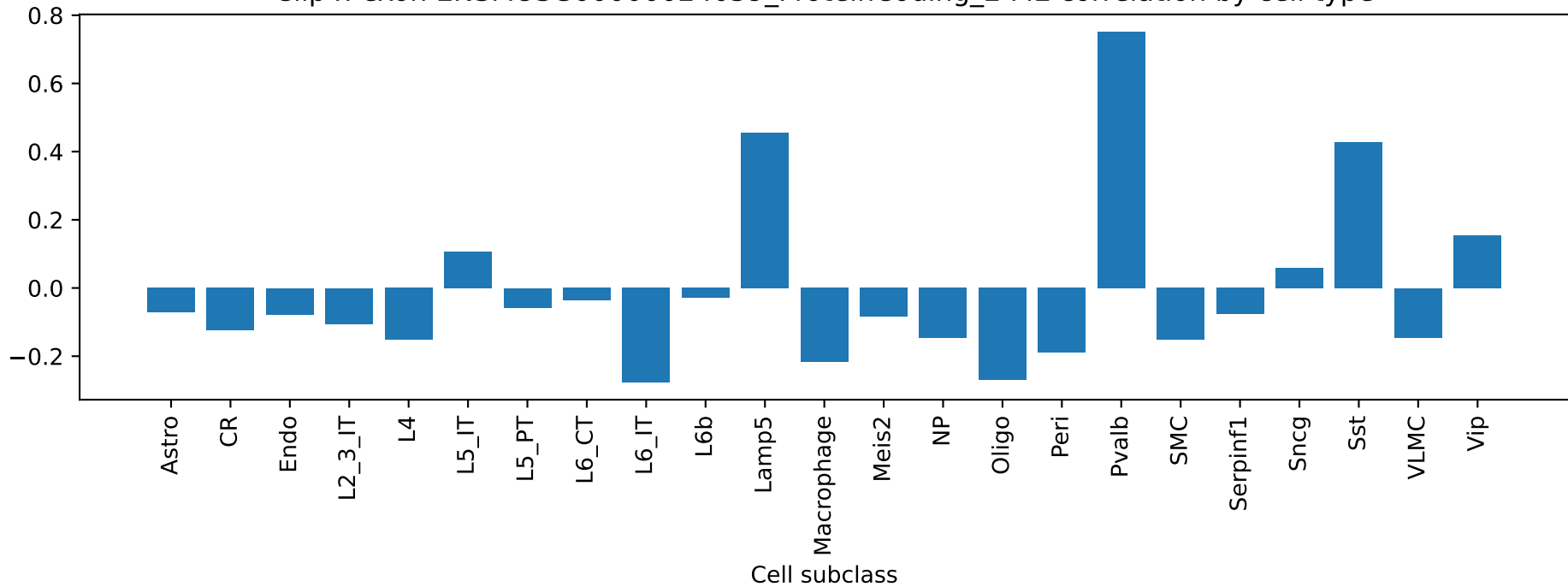
Clip4: exon ENSMUSG00000024059_ProteinCoding_2 ME correlation by cell type
