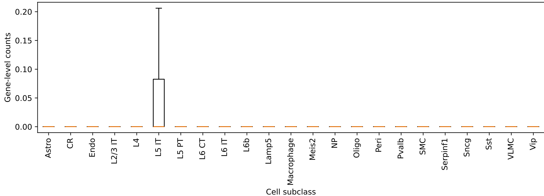
Vill: gene-level counts by cell type
