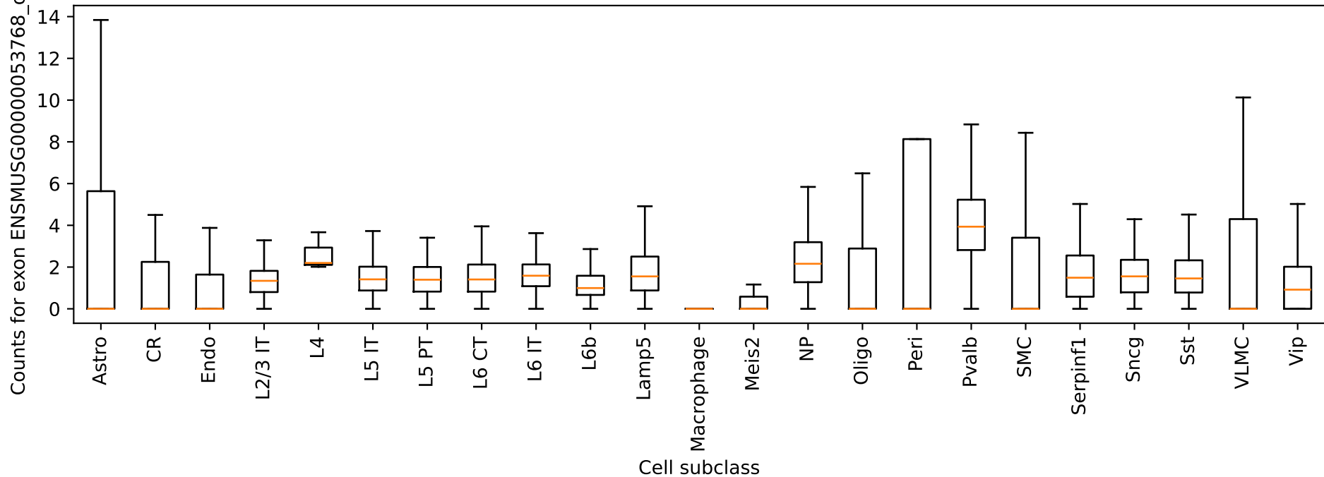
Chchd3: exon ENSMUSG00000053768_other_2 counts by cell type
