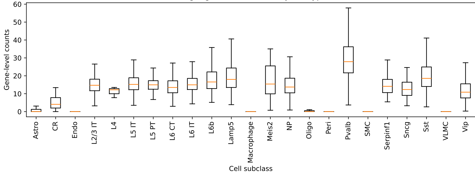
Ndr4: gene-level counts by cell type
