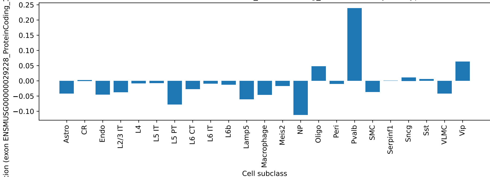
LnX1: exon ENSMUSG00000029228_ProteinCoding_1 correlation by cell type
