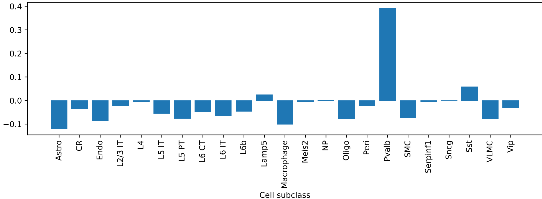
Kctd17: exon ENSMUSG00000033287_ProteinCoding_5 correlation by cell type
