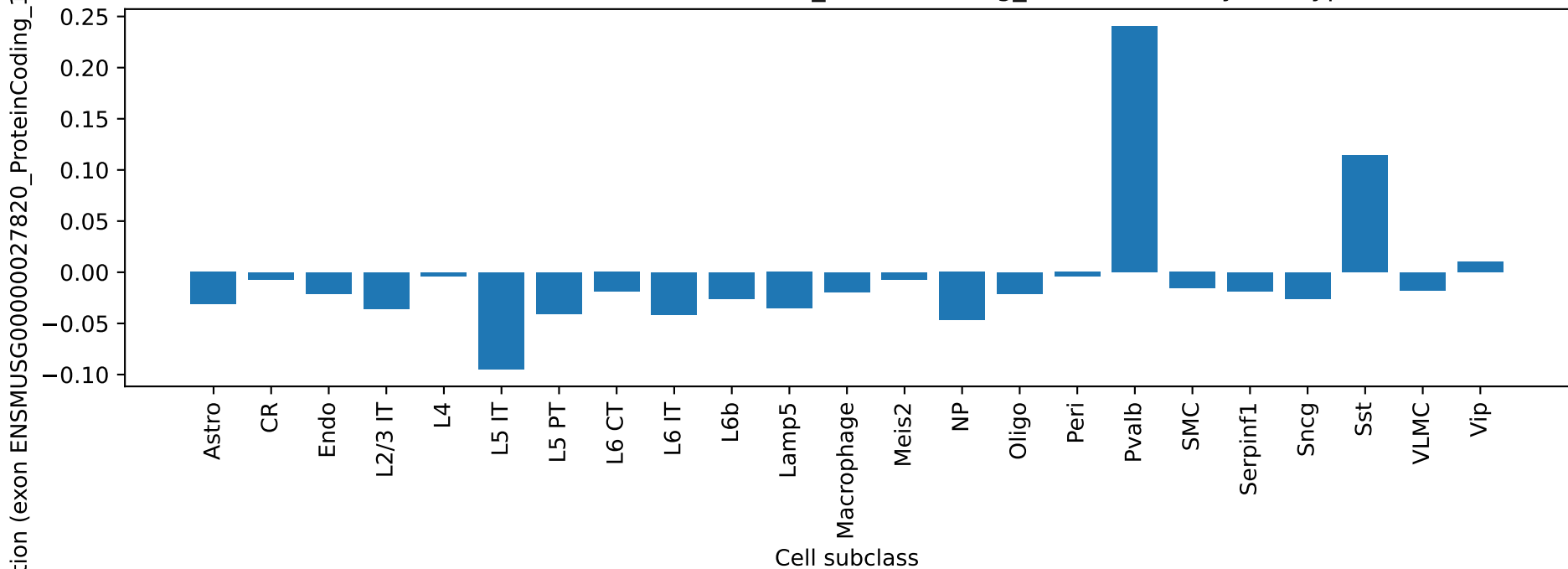
Mme: exon ENSMUSG00000027820_ProteinCoding_1 correlation by cell type
