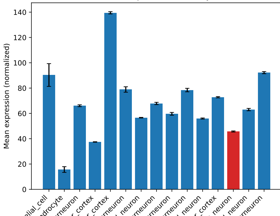
Gene expression for Nbdy
