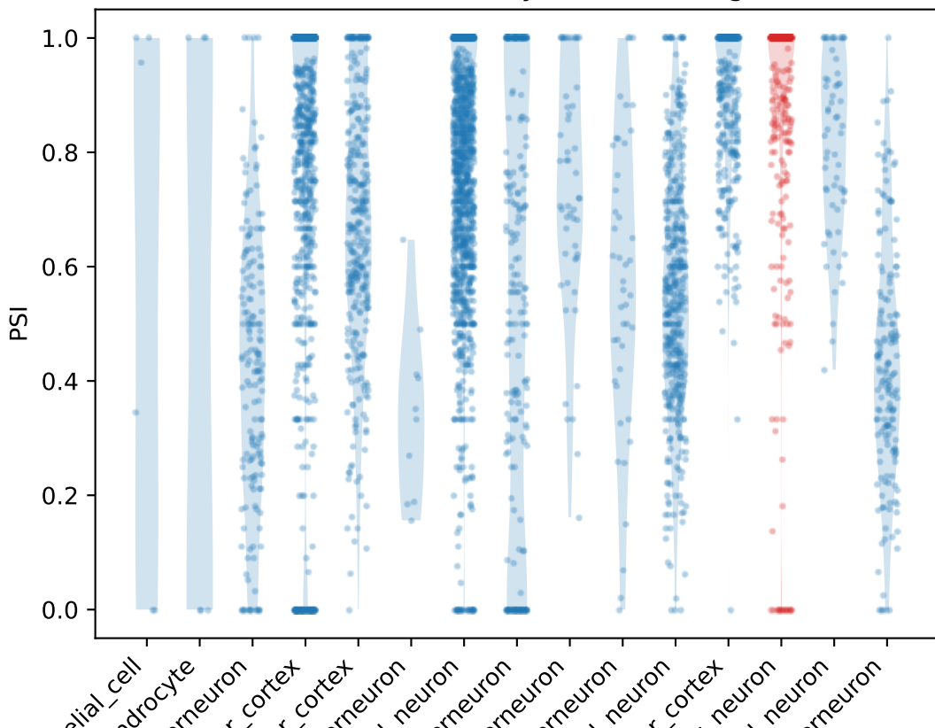
PSI distribution for Nbdy ProteinCoding2 exon
