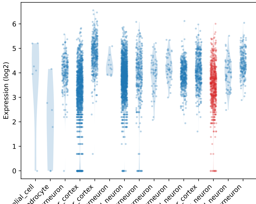
Count distribution for Nbdy
