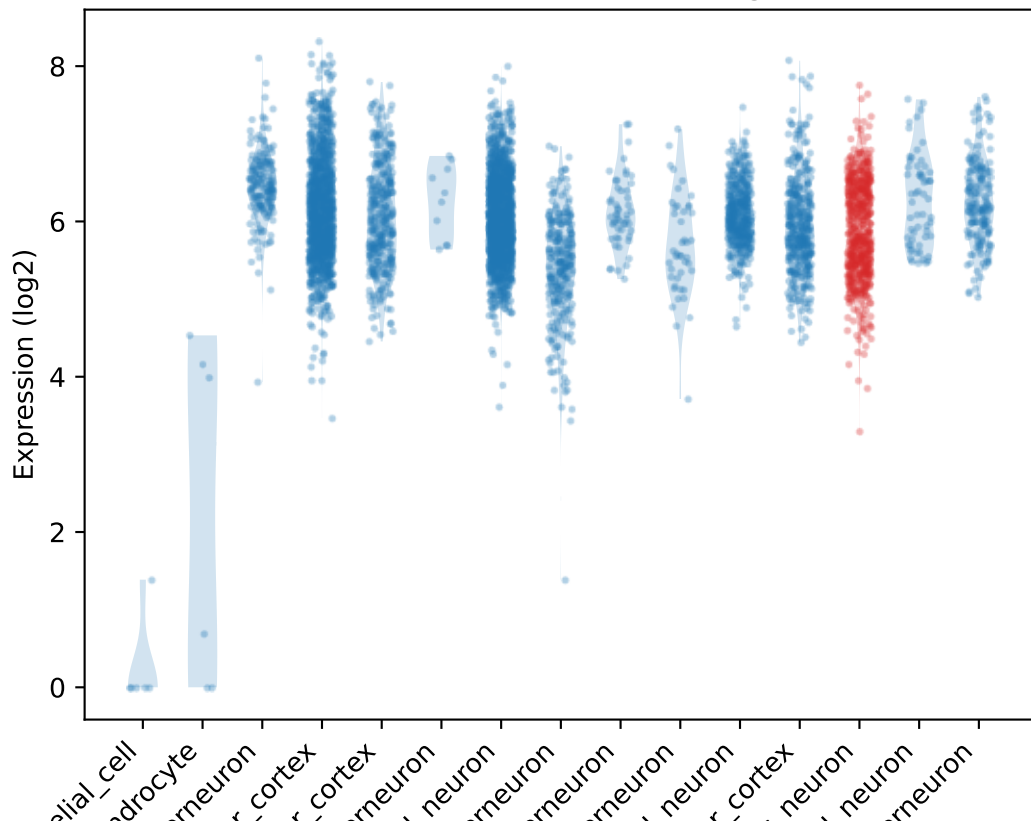
Count distribution for Ndr4
