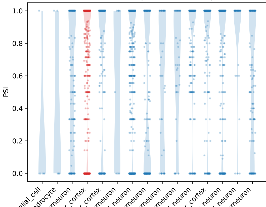
PSI distribution for Rnps1 ProteinCoding1 exon
