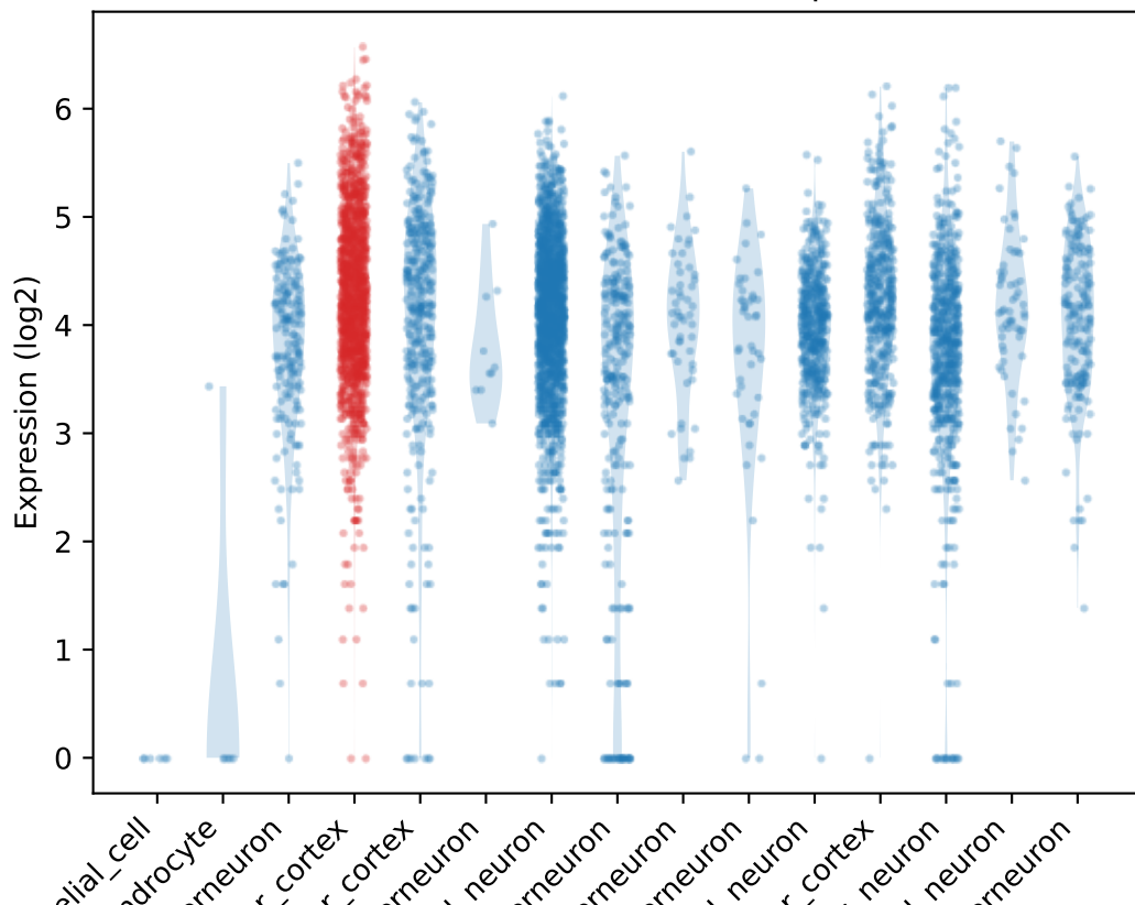
Count distribution for Snap91
