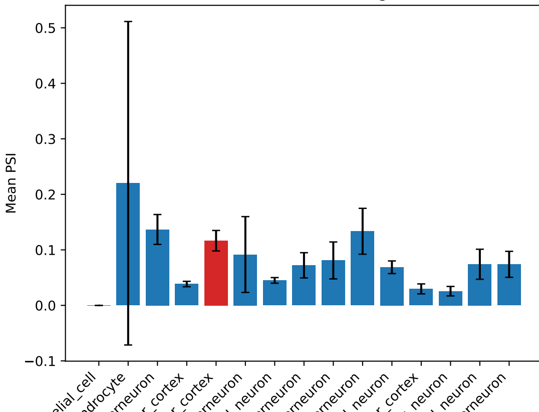
PSI for Dctn6 ProteinCoding4 exon
