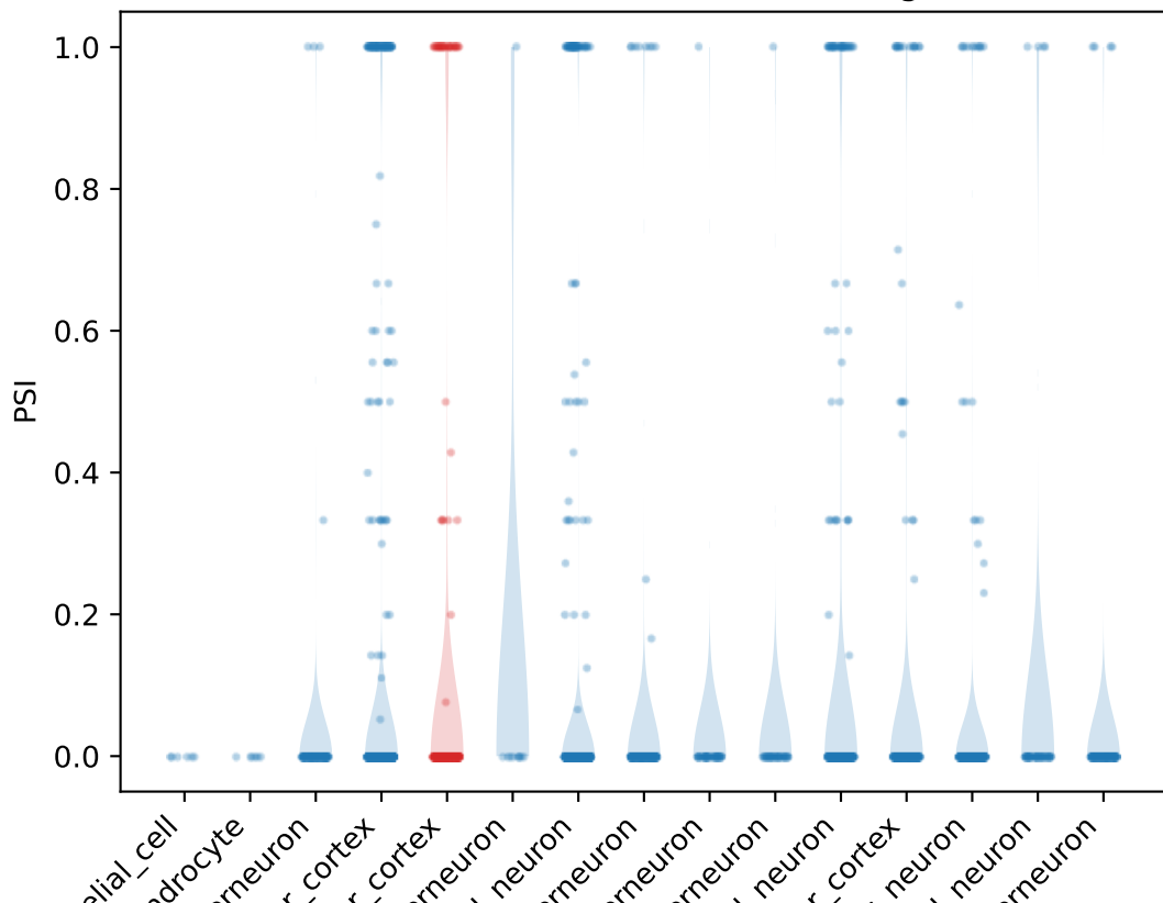
PSI distribution for Erc1 ProteinCoding4 exon
