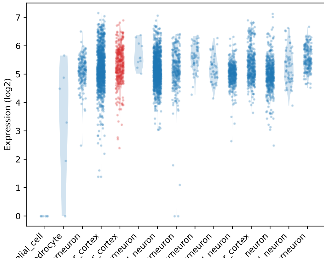
Count distribution for Grina
