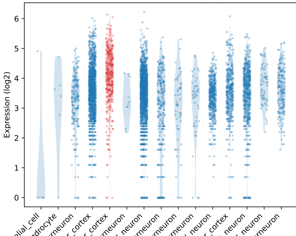
Count distribution for Hp1bp3
