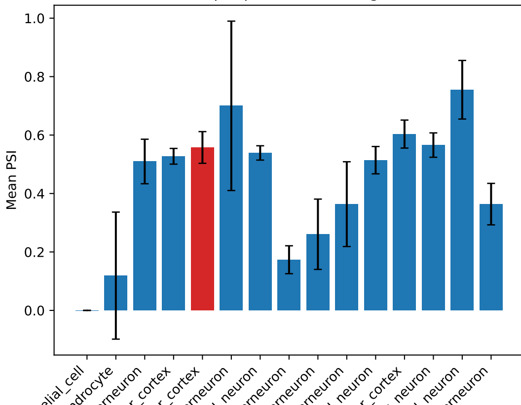
PSI for Hp1bp3 ProteinCoding2 exon
