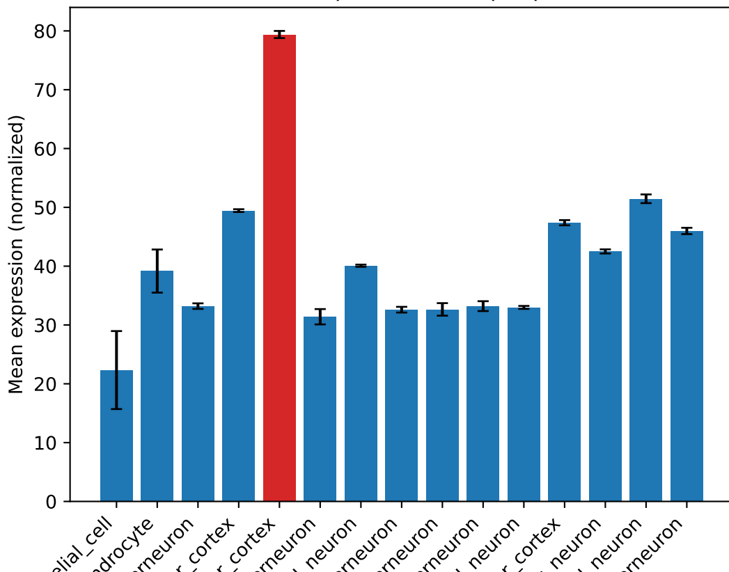
Gene expression for Hp1bp3
