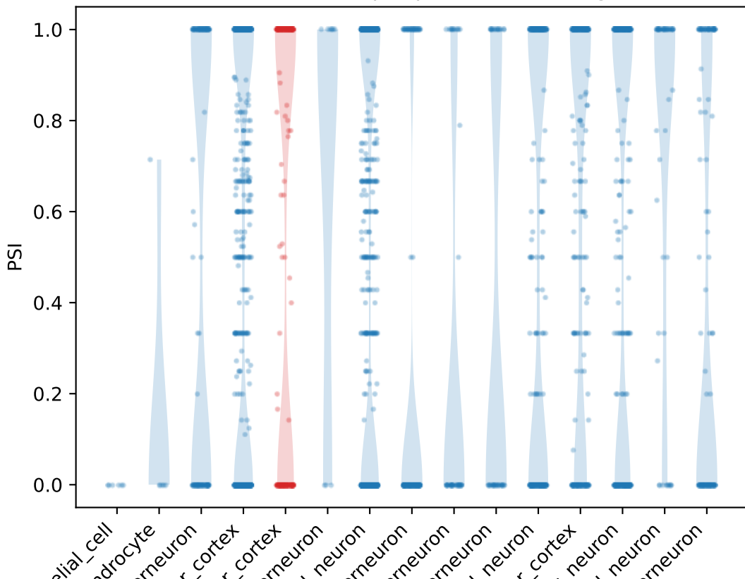
PSI distribution for Hp1bp3 ProteinCoding2 exon
