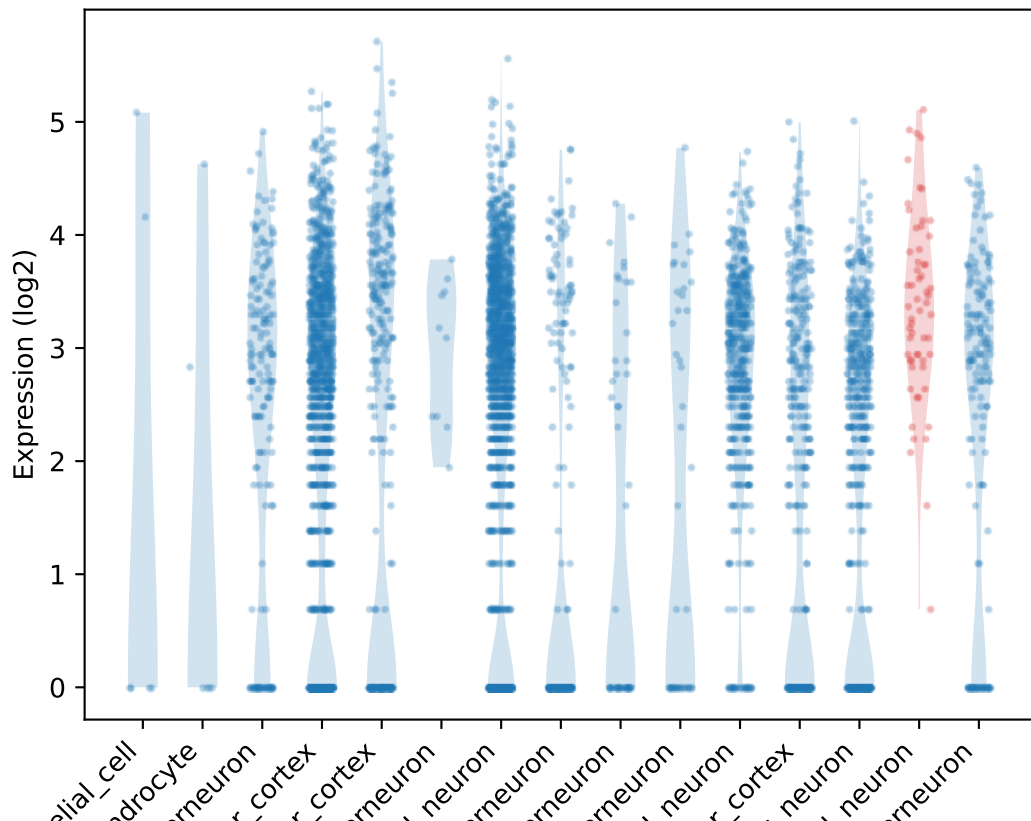
Count distribution for Fez2
