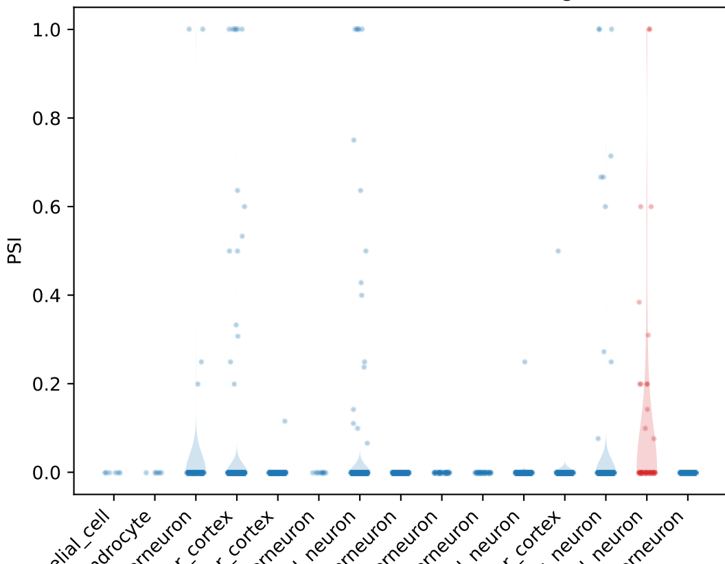
PSI distribution for Fez2 ProteinCoding1 exon
